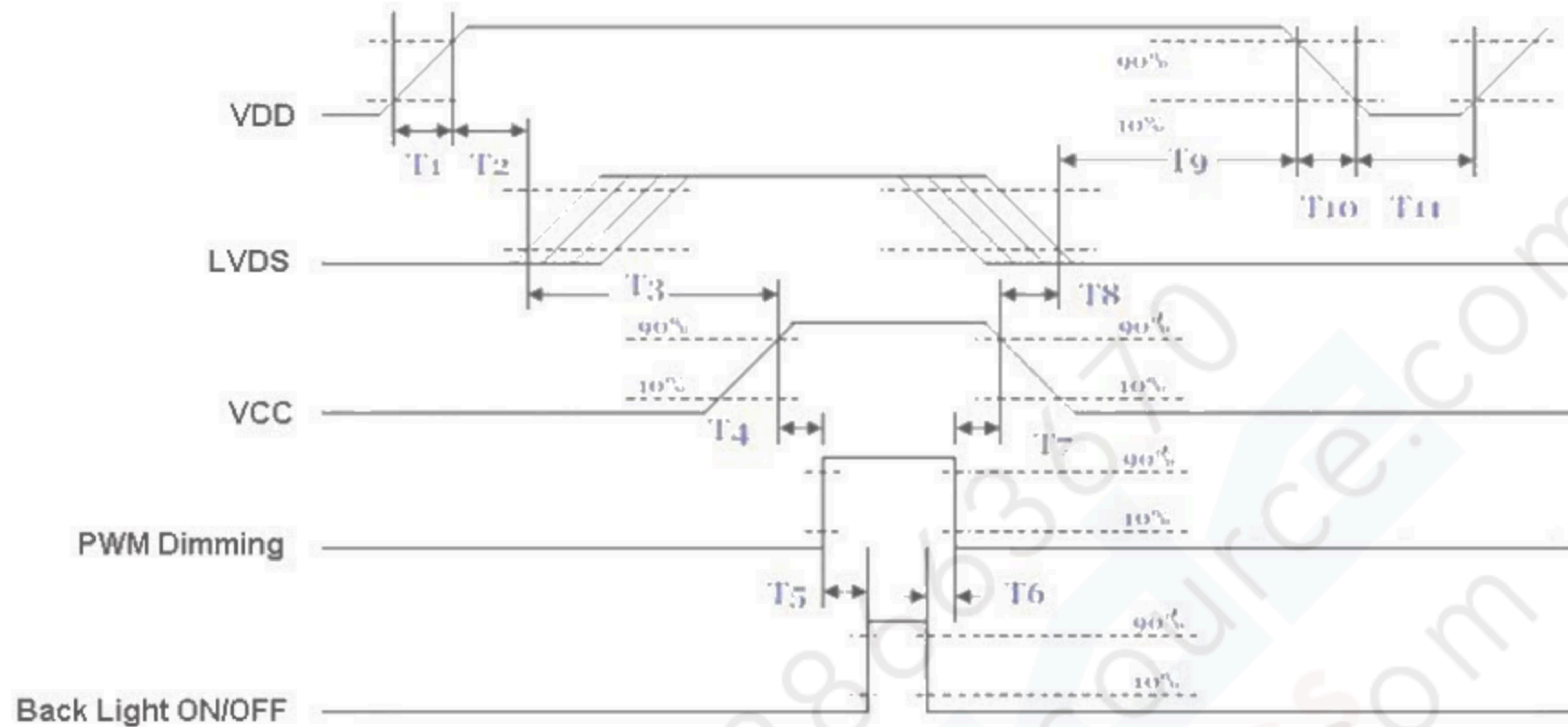
Power ON/OFF sequence timing
