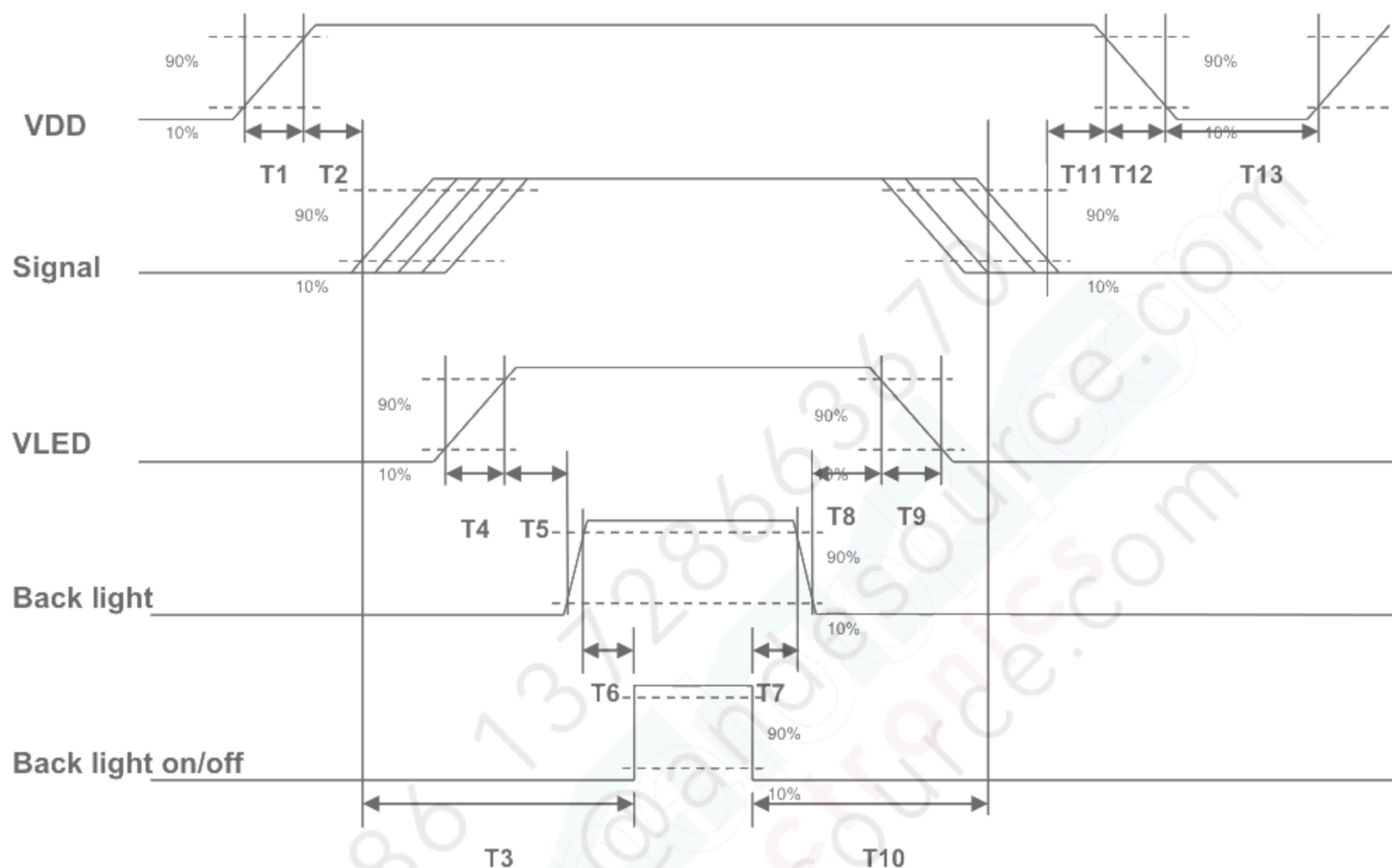
Power Sequence Timing
