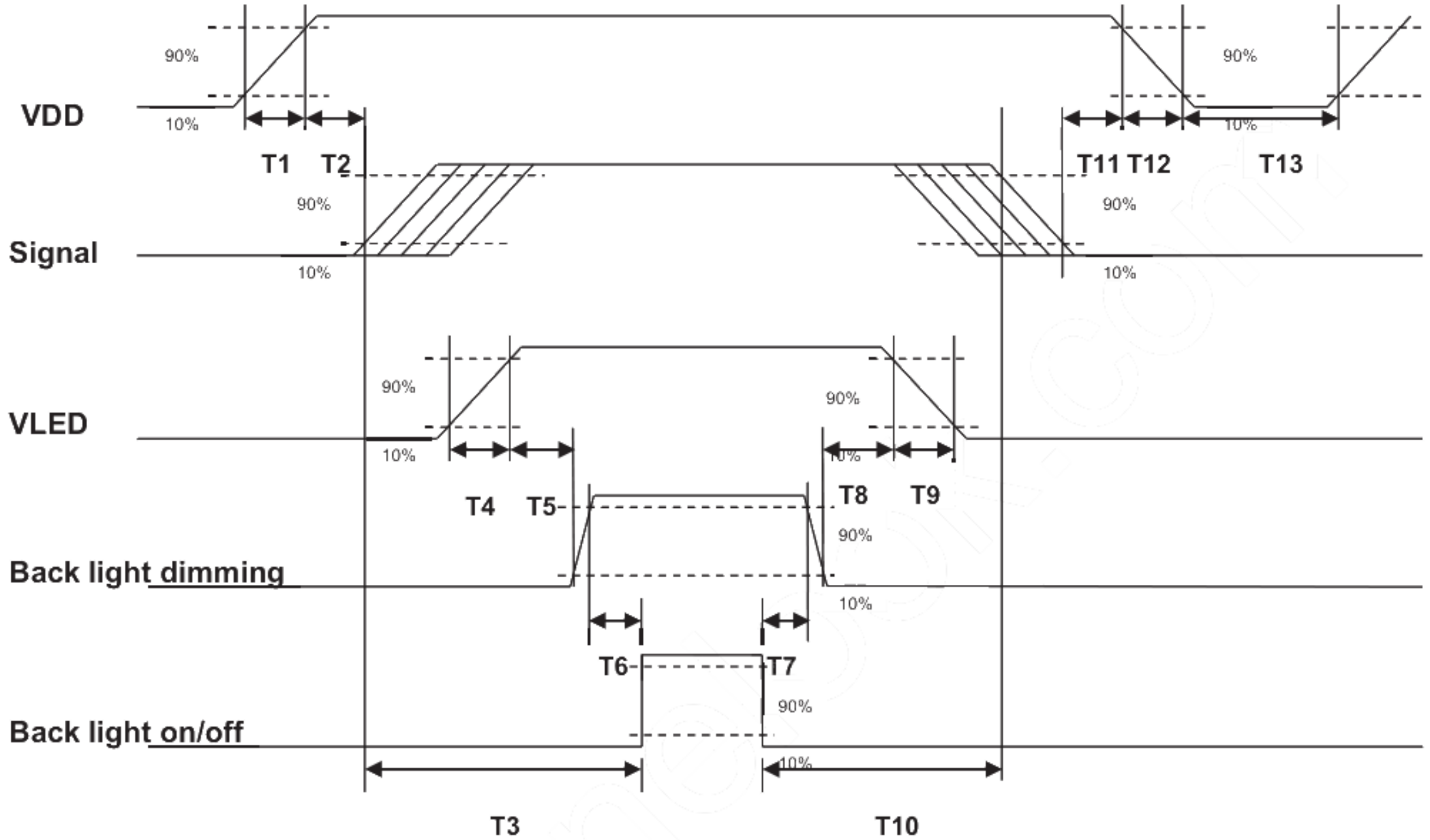
Power Sequence Timing
