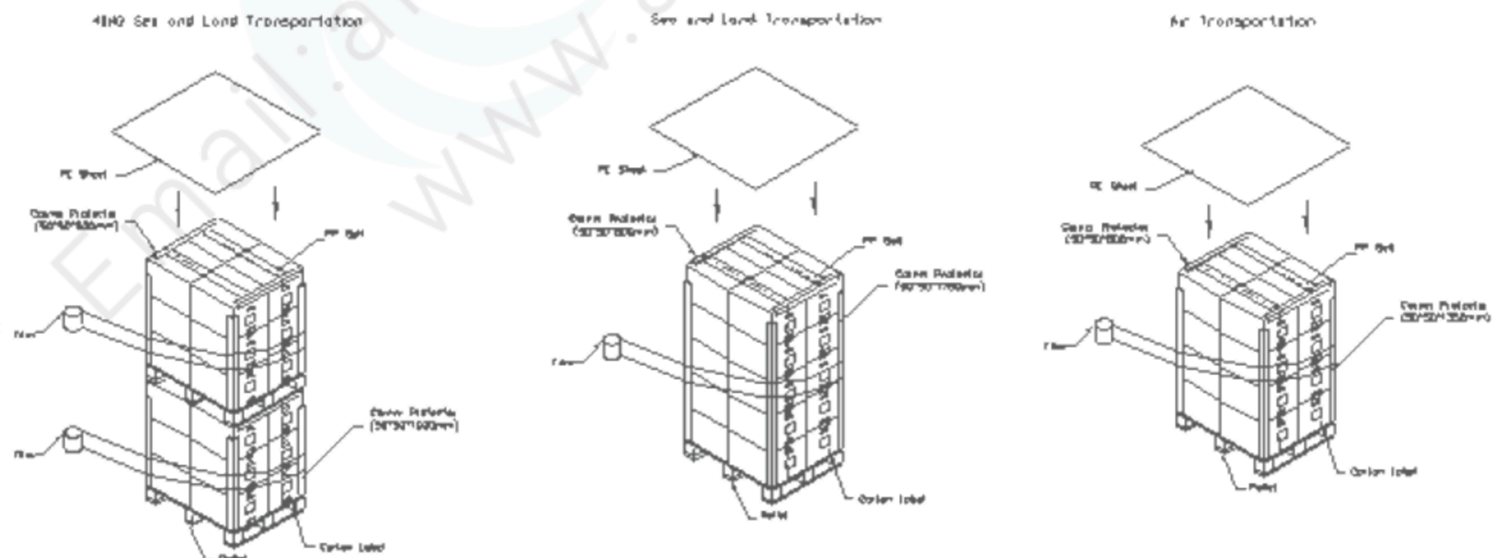
Figure. 9-2 Packing method
