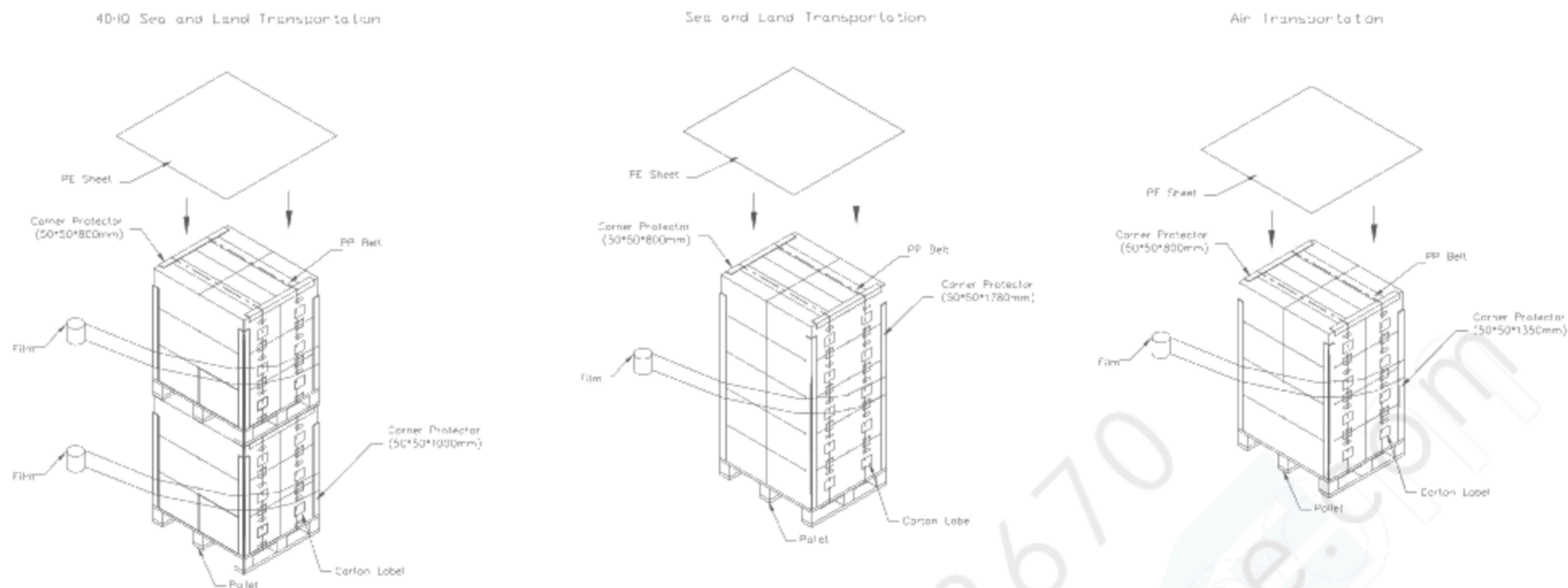
Figure. 9-2 Packing method
