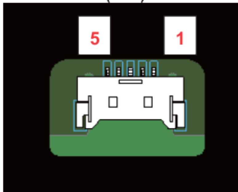
Touch Connector (CN3):
