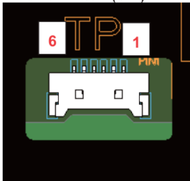
Touch Connector (CN3):
