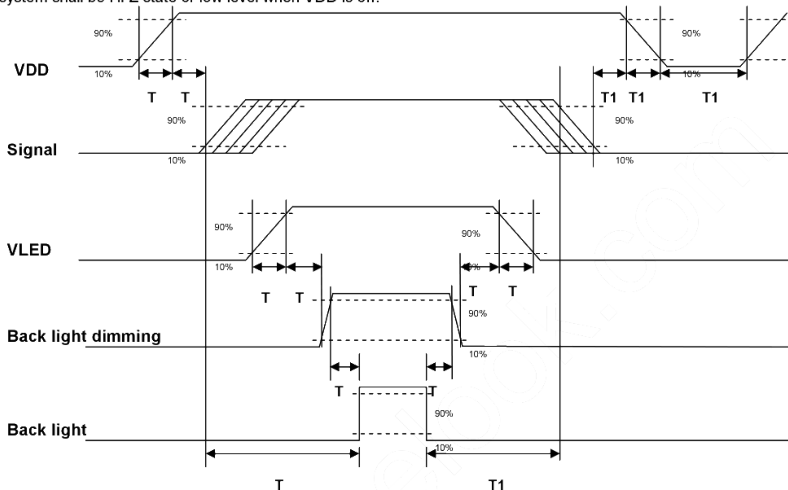
Power Sequence Timing
