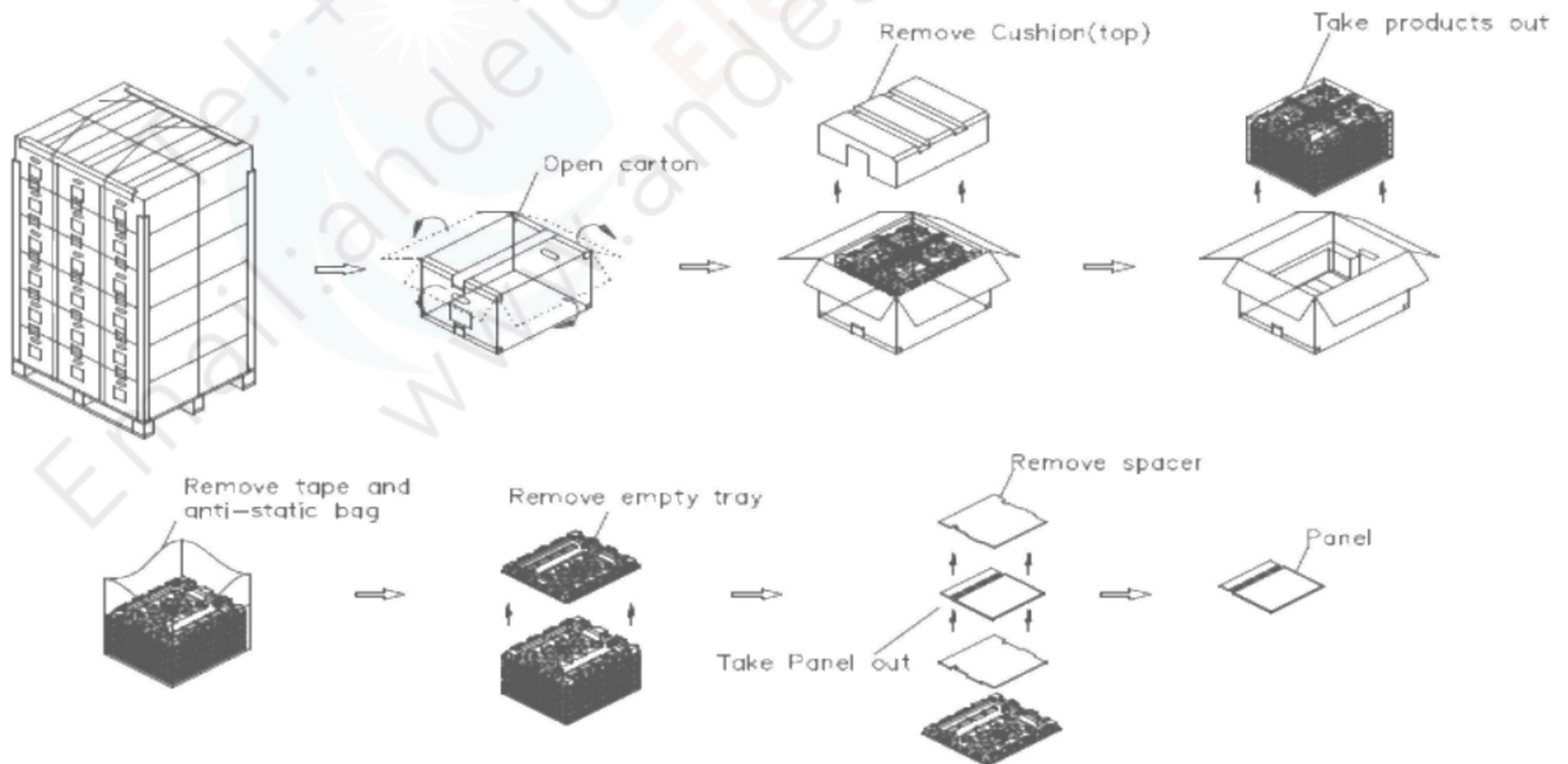
Figure. 7-3 UN-Packing
