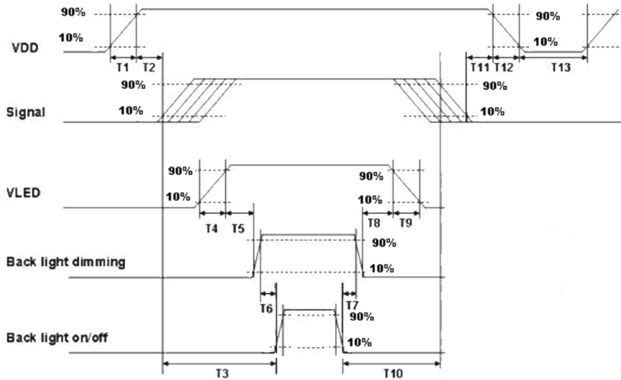
Power Sequence Timing
