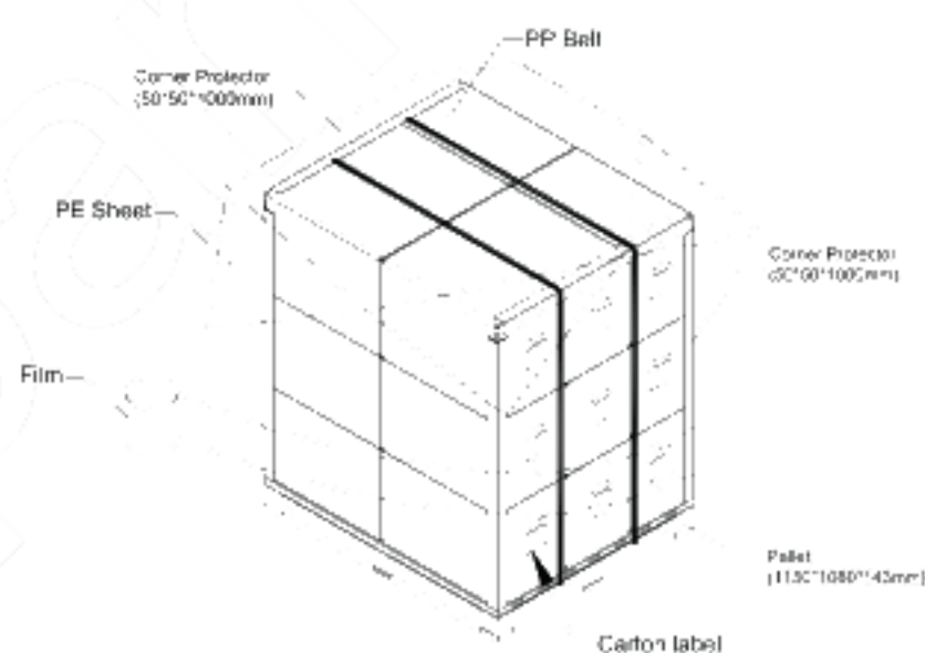
Figure. 7-2 Packing method
