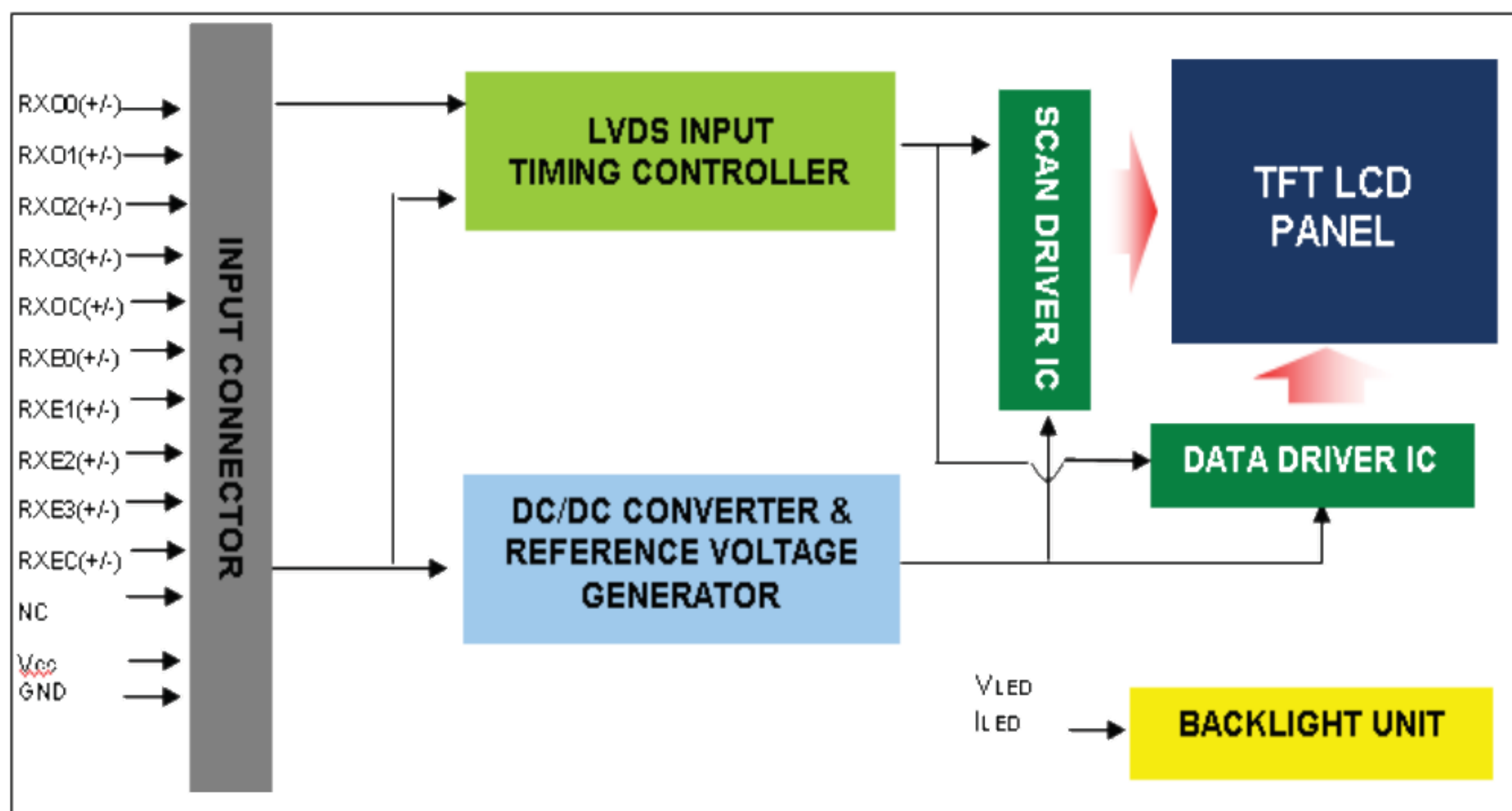
Fig. 4-1 Module Function Block Diagram
