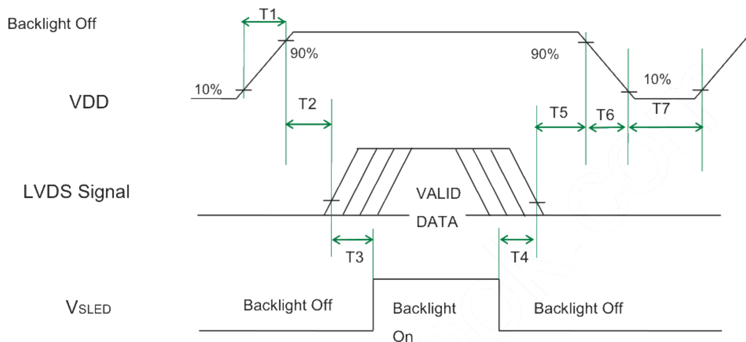
Power Sequence Timing
