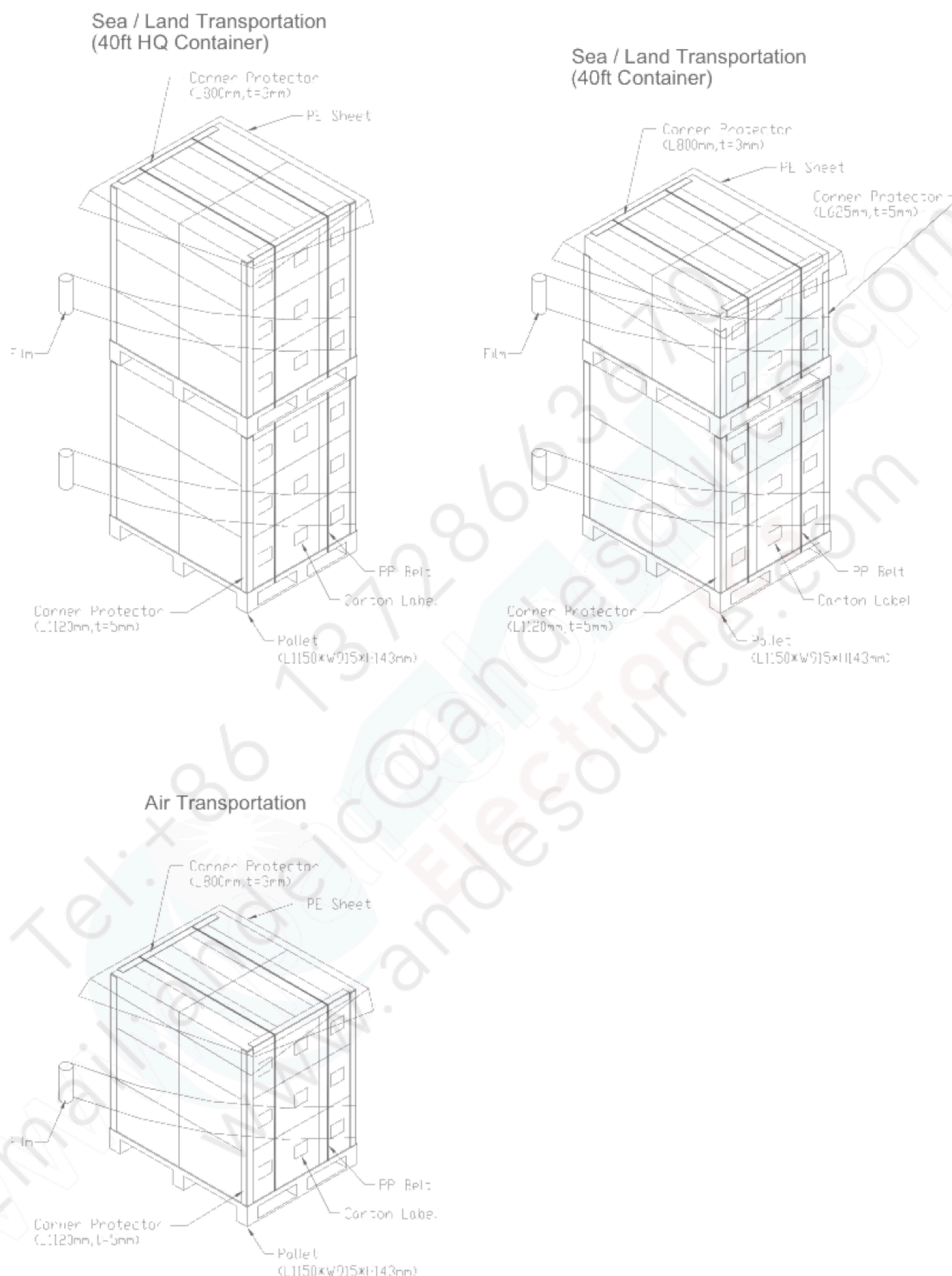
Figure. 8-2 Packing method
