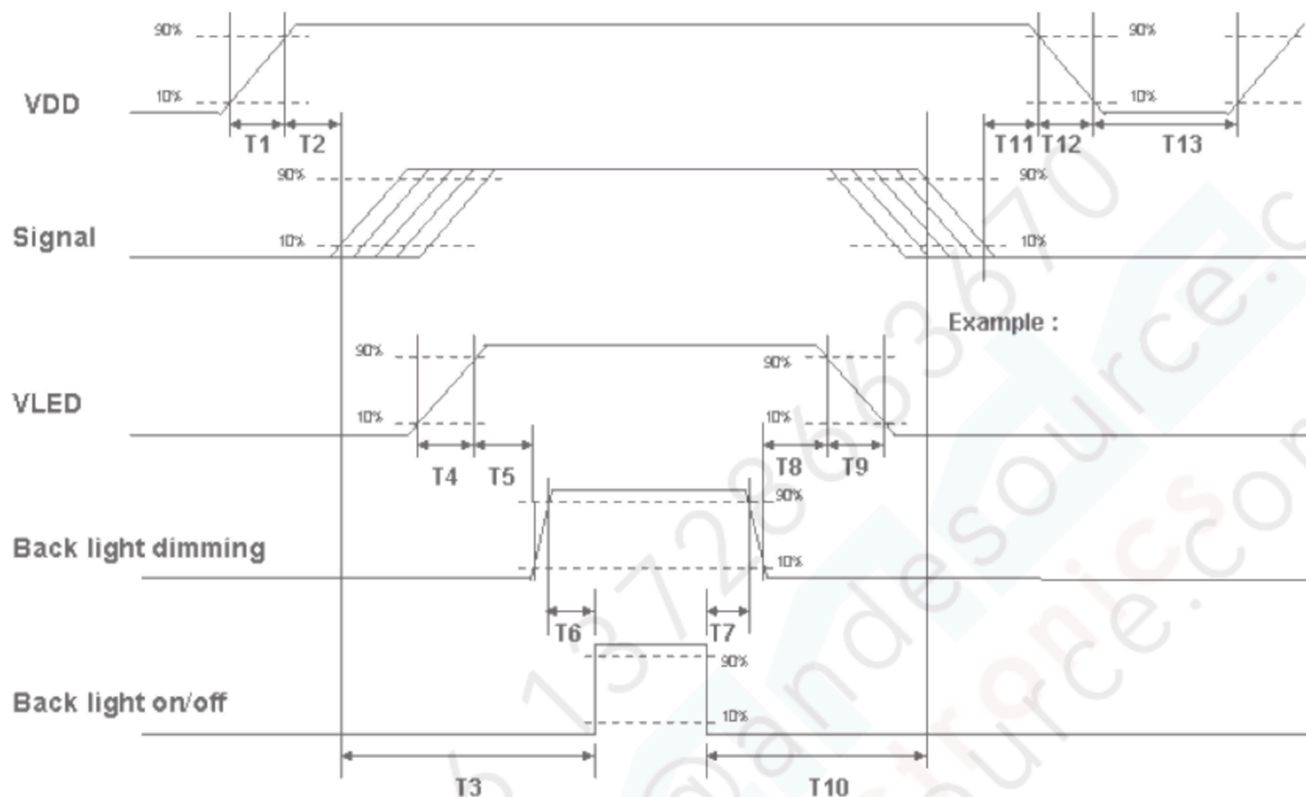
Power ON/OFF sequence timing
