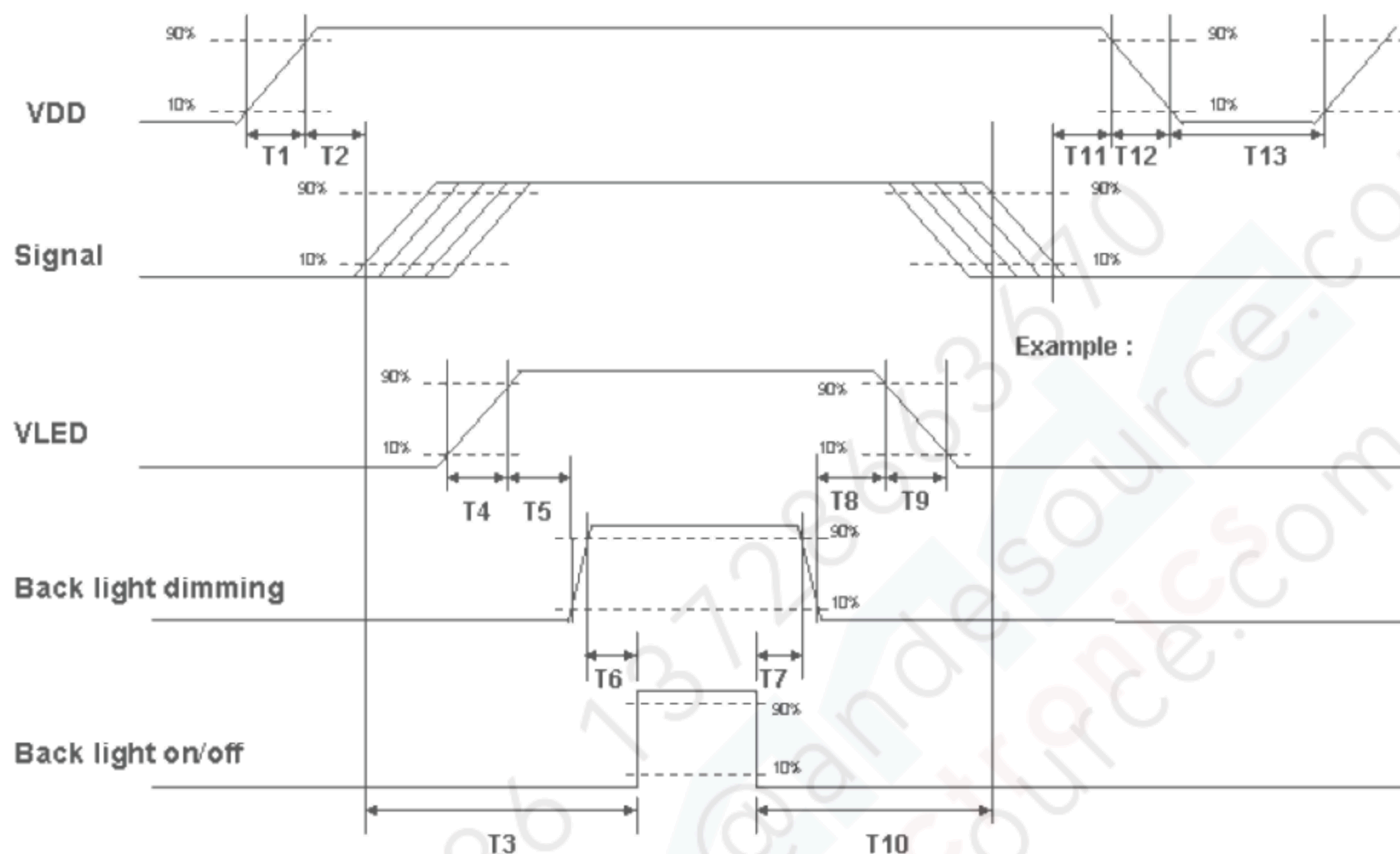
Power ON/OFF sequence timing
