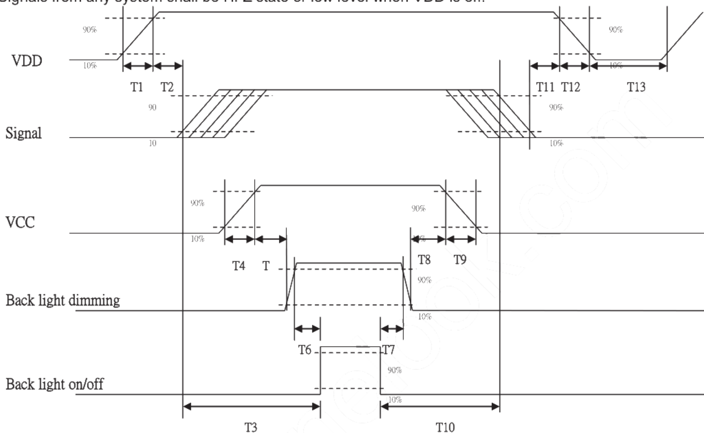
Power ON/OFF sequence timing
