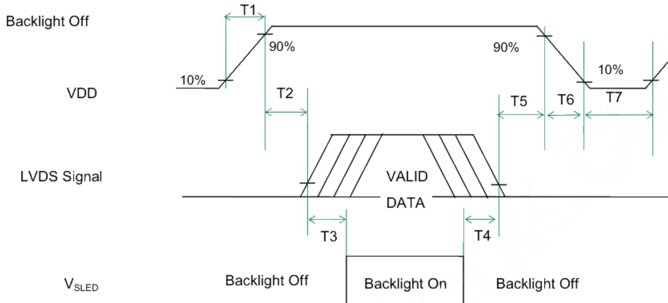
Power Sequence Timing
