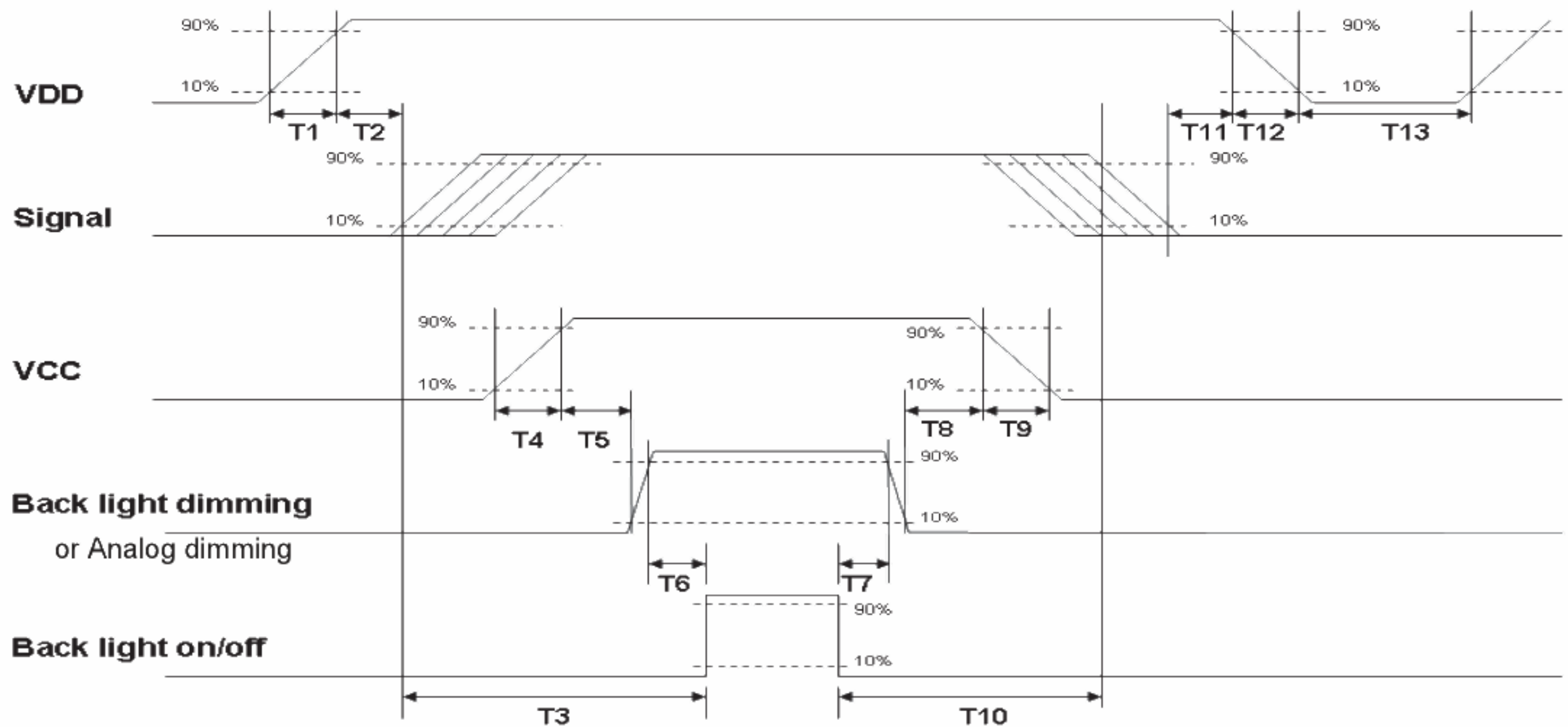
Power ON/OFF sequence timing
