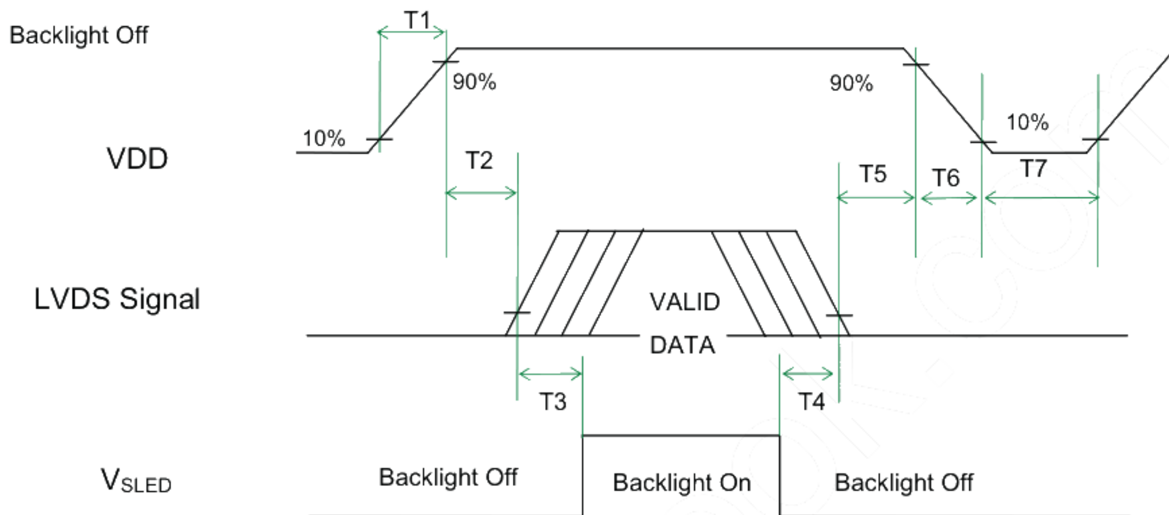
Power Sequence Timing
