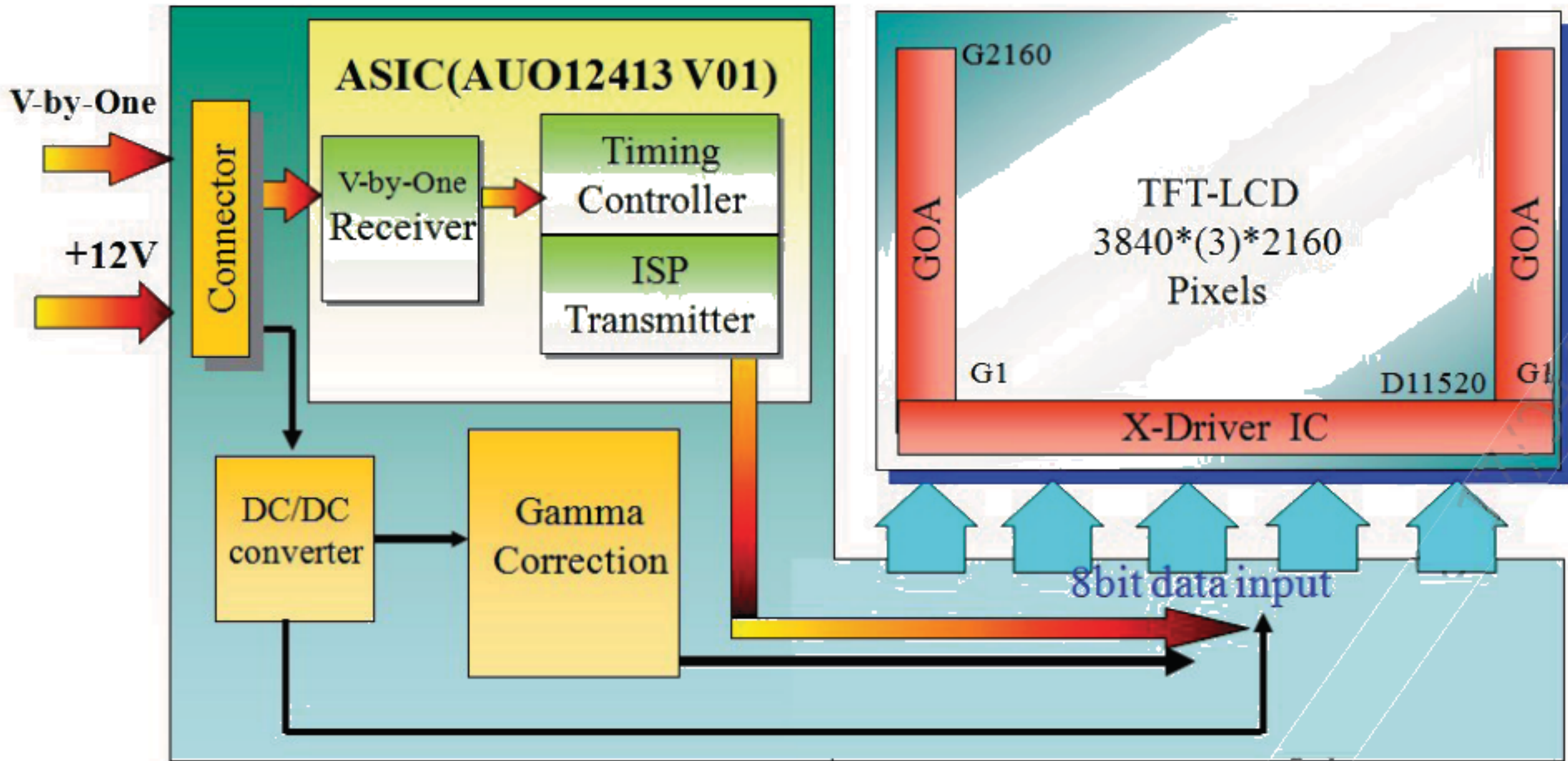
X PCB
