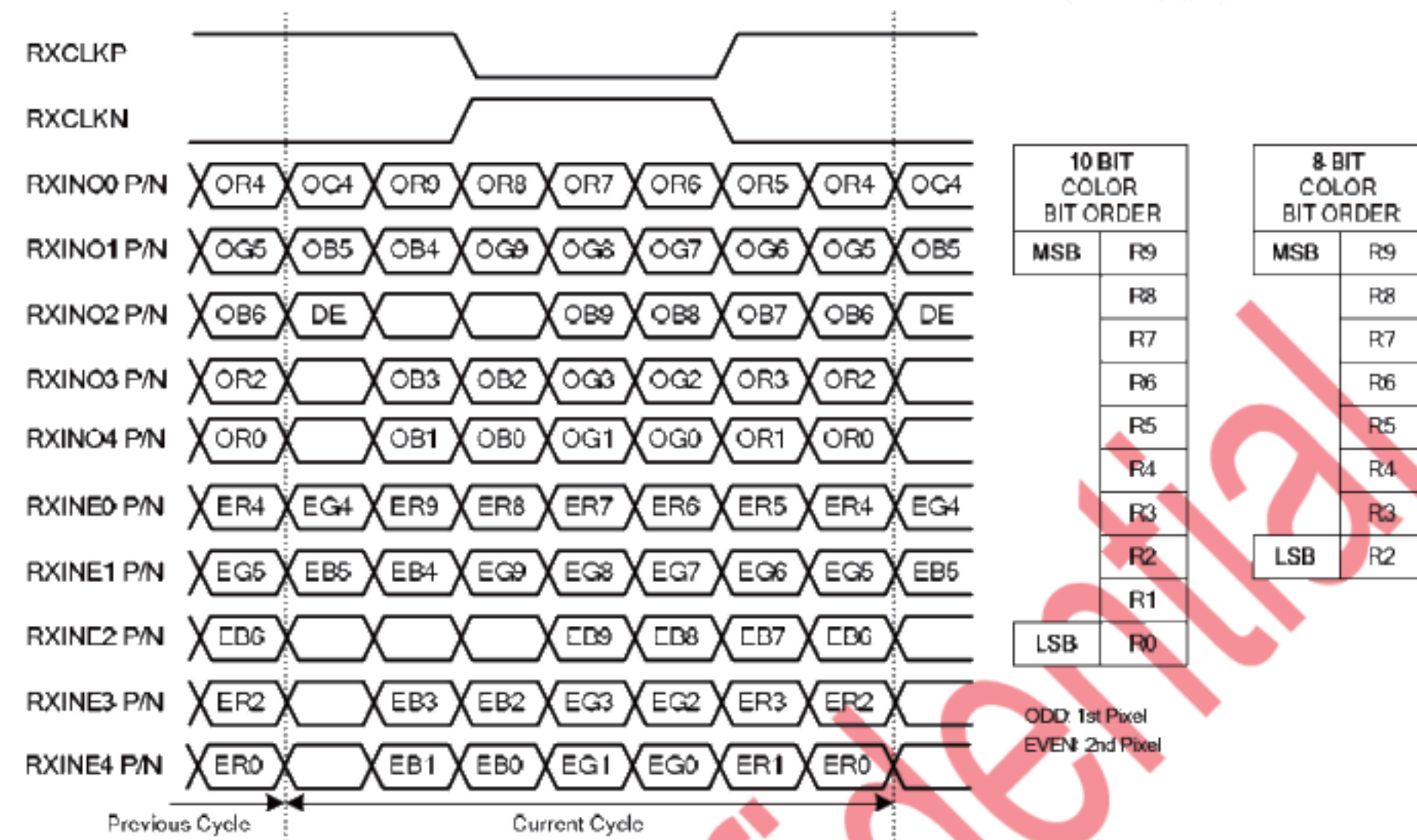
Data Mapping of JEIDA Format
