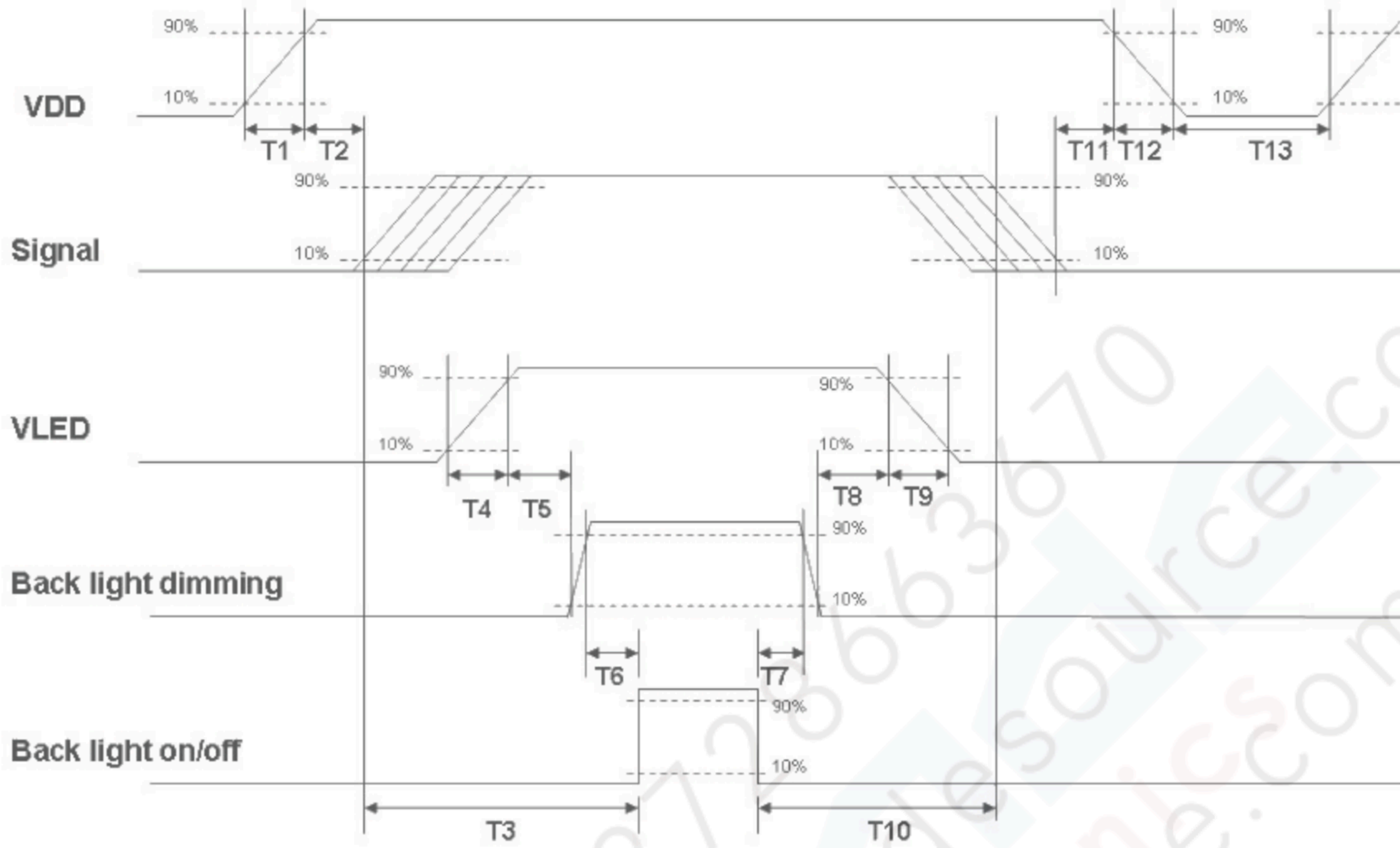
Power sequence timing
