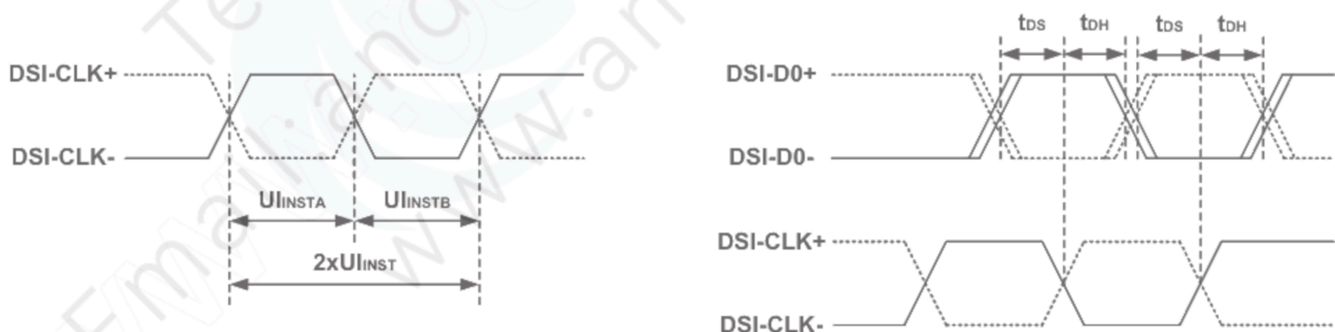
DSI clock channel timing
