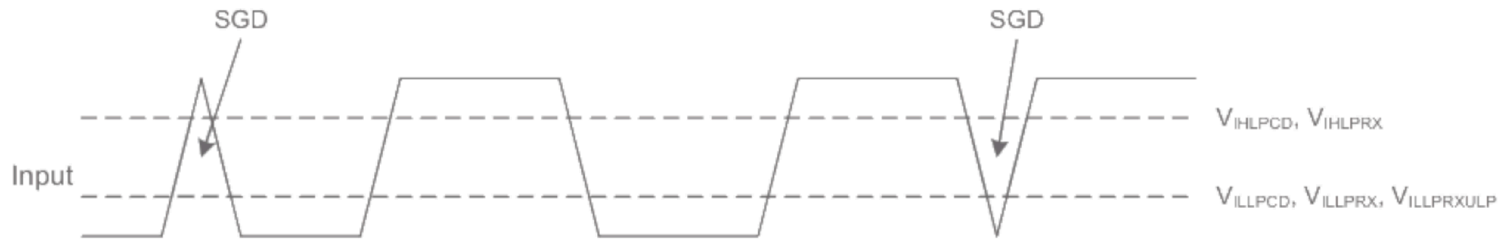
Spike/Glitch rejection-DSI
