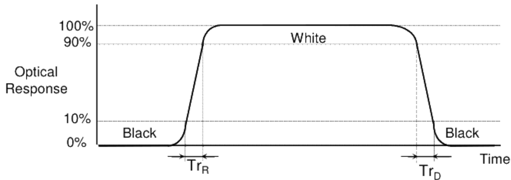
FIG. 5 Response Time
