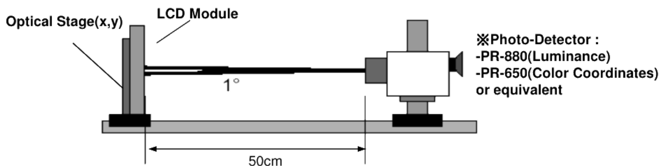
FIG. 3 Electro-optical Characteristic Measurement Equipment and Method
