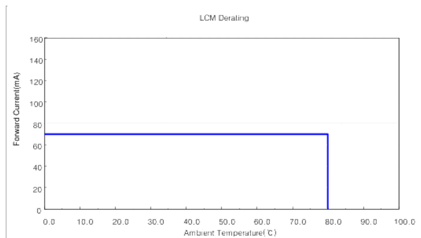
Ambient Temperature vs. Allowable Forward Current
