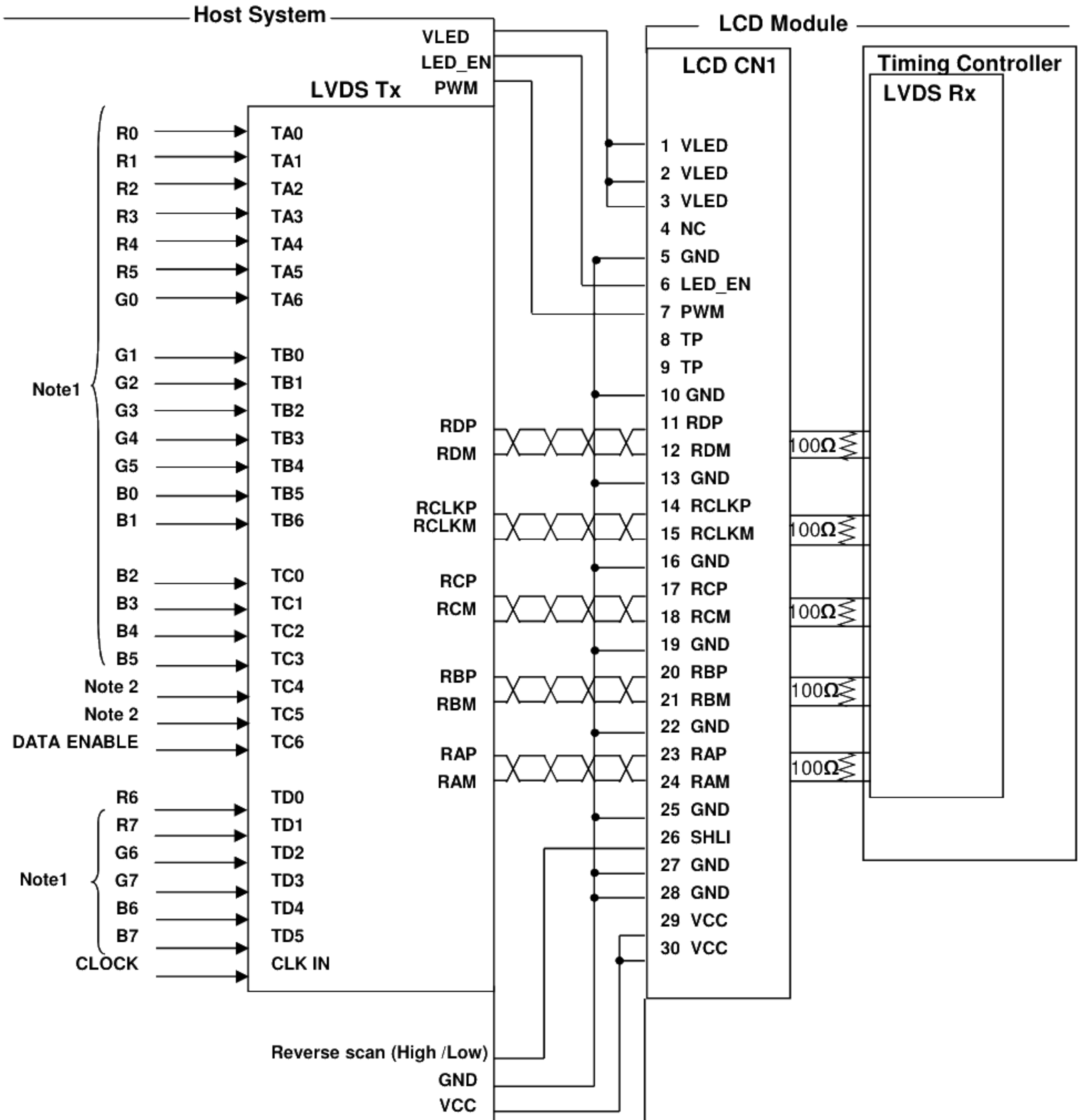
Fig 1. REQUIRED SIGNAL ASSIGNMENT FOR LVDS TRANSMITTER(THC63LVDM83R)
