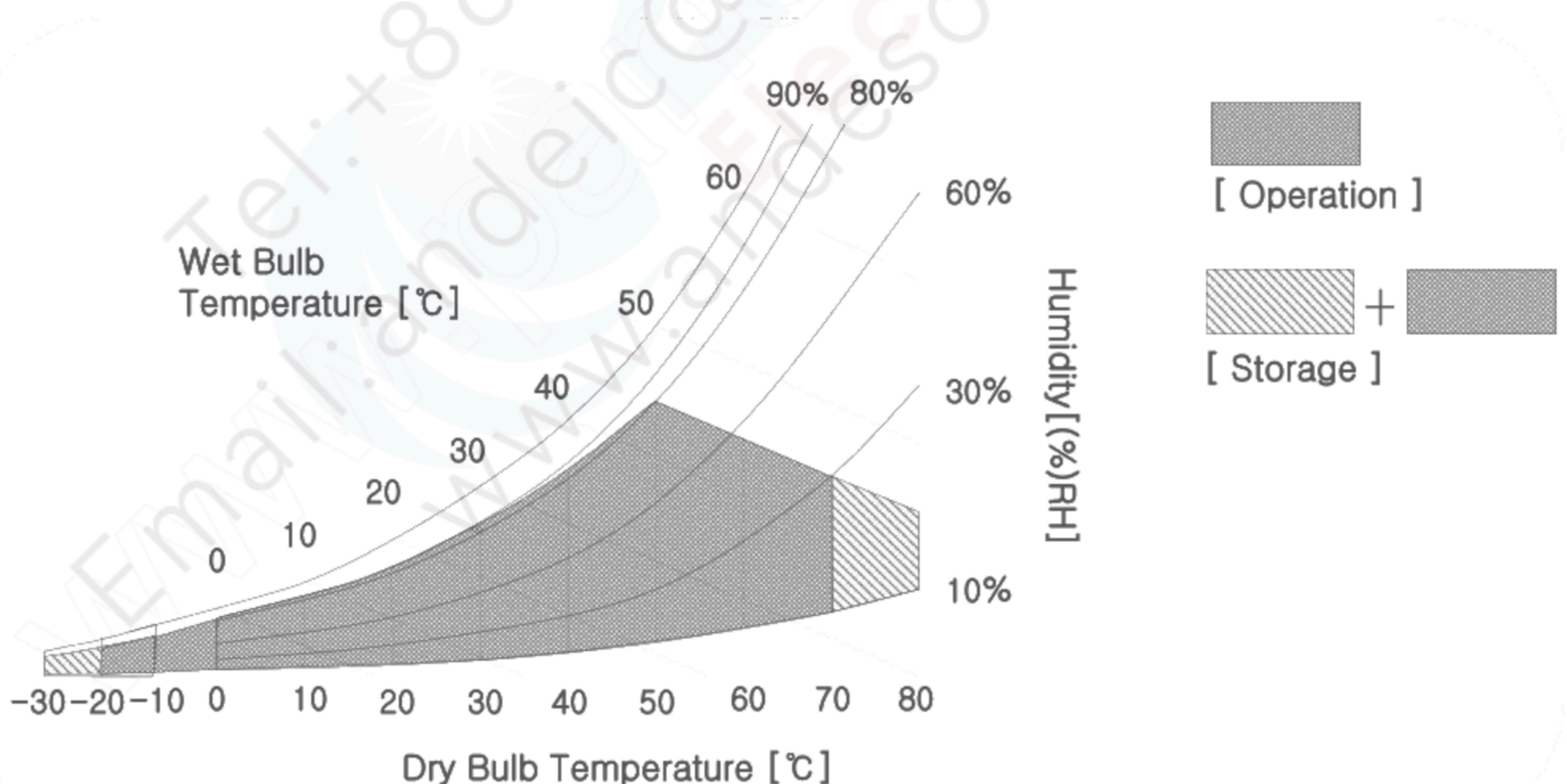
FIG.2 Temperature and relative humidity
