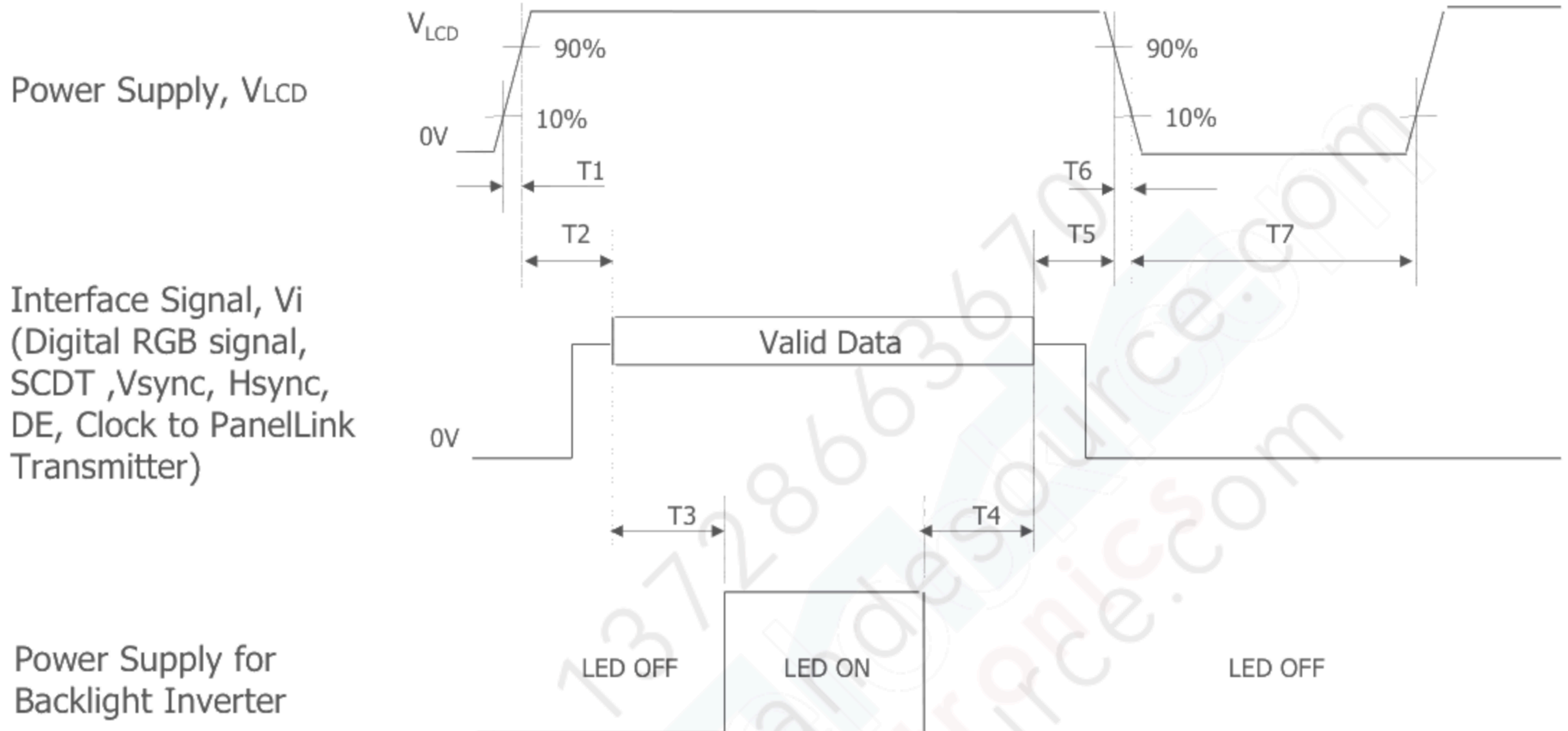
FIG.5 Power sequence
