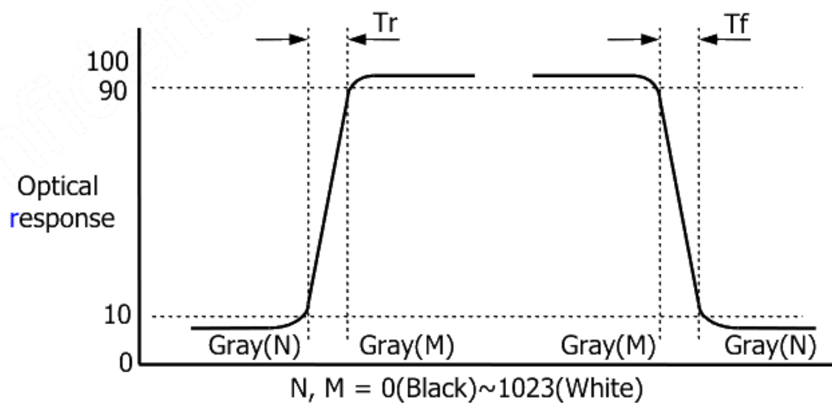
[FIG. 9] Response Time
