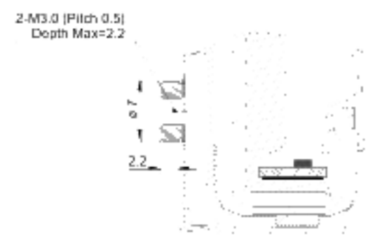
SECTION F-F SCALE 2/1
