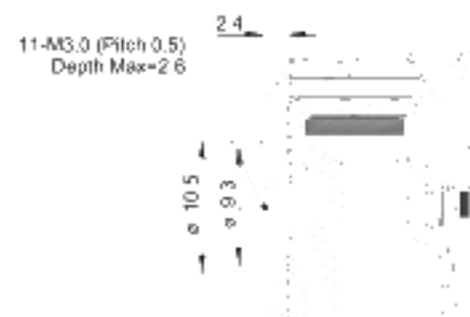
SECTION C-C SCALE 2/1
