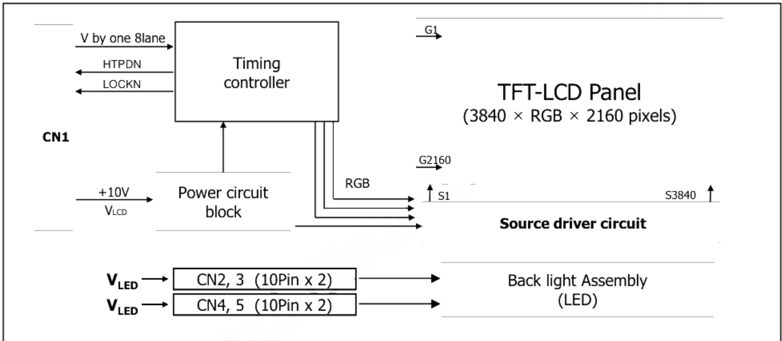
[FIG. 1] Block diagram
