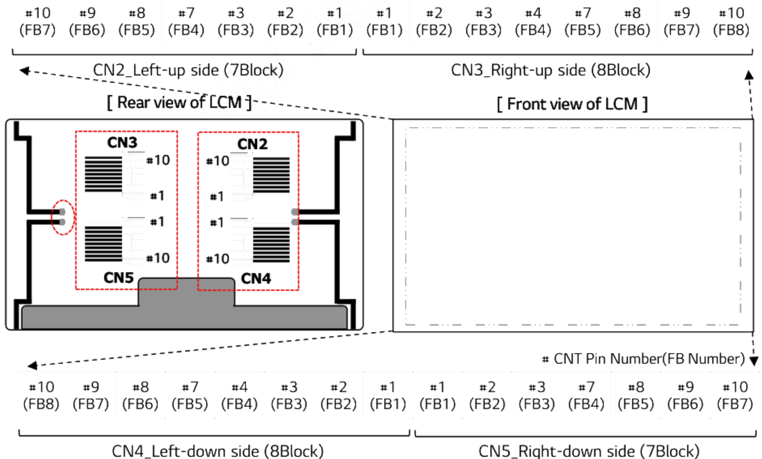
[FIG. 5] Backlight connector view
