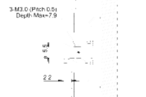
SECTION E-E SCALE 2/1
