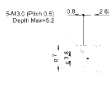
SECTION D-D SCALE 2/1
