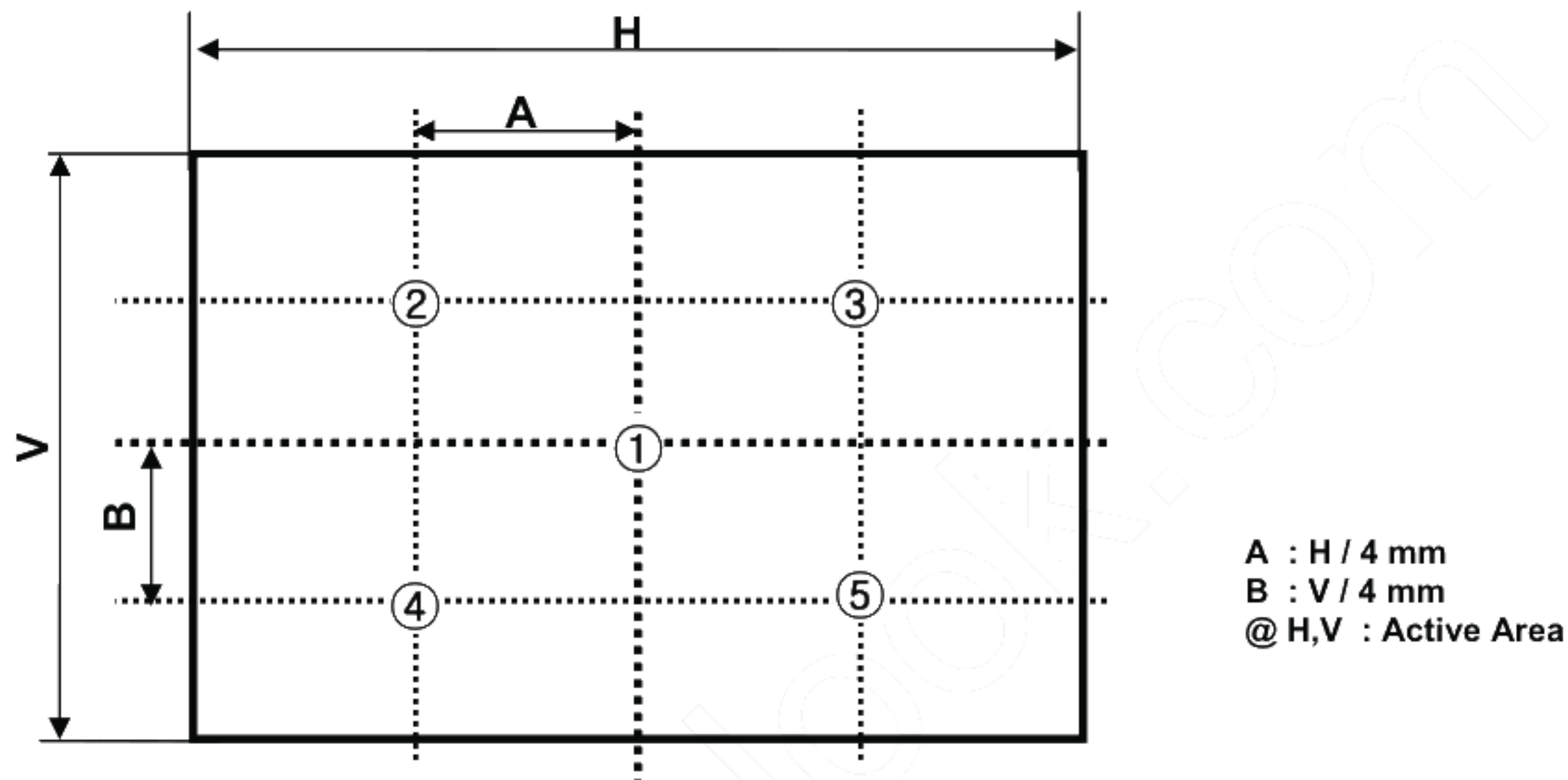
FIG. 2 5 Points for Luminance Measure
