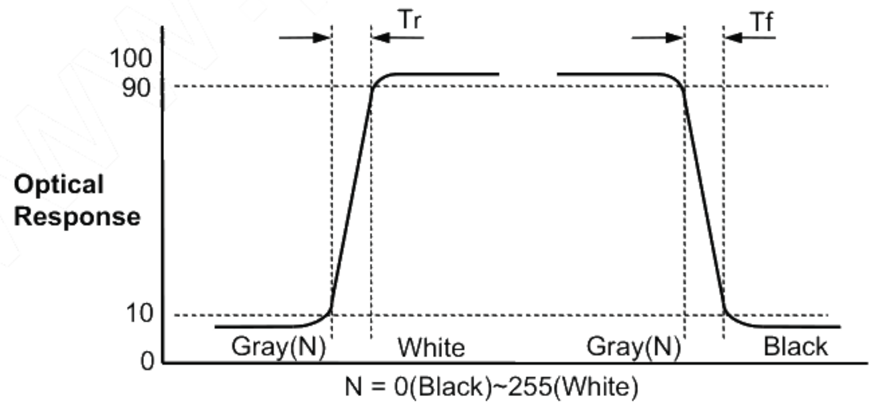
FIG. 3 Response Time
