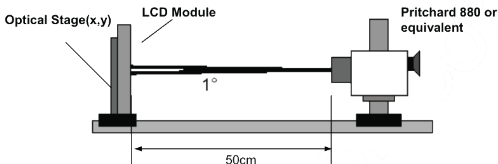
FIG. 1 Optical Characteristic Measurement Equipment and Method
