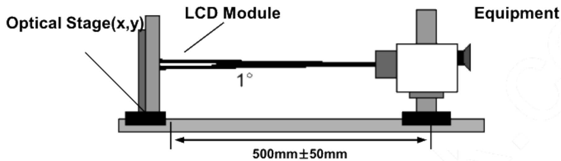
FIG. 2 Optical Characteristic Measurement Equipment and Method
