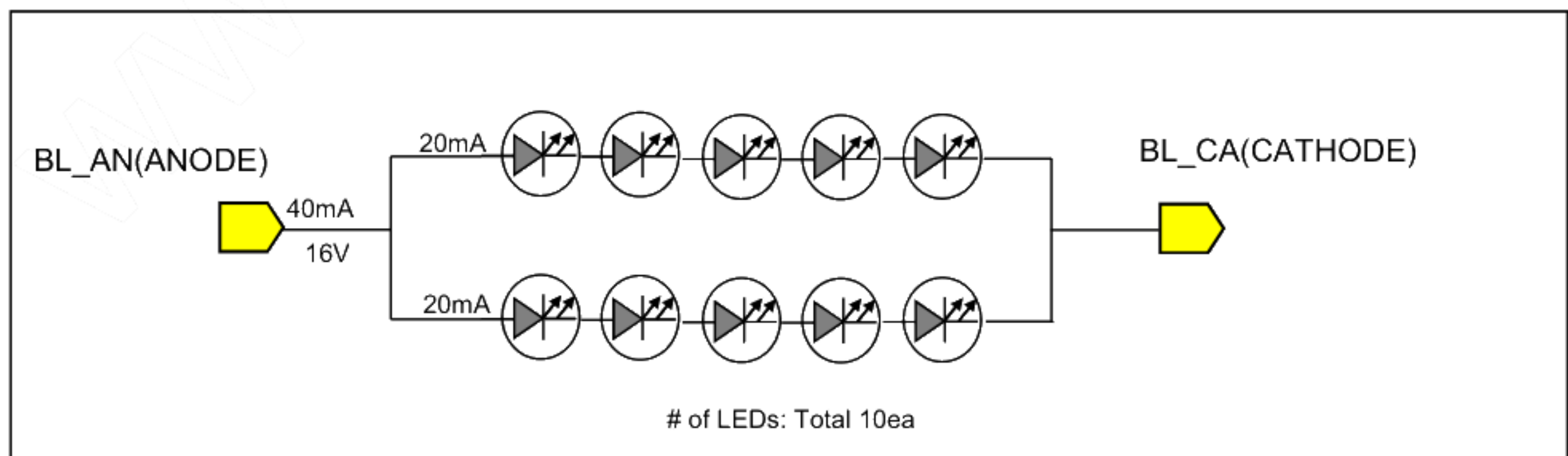
Fig 1. LED configuration
