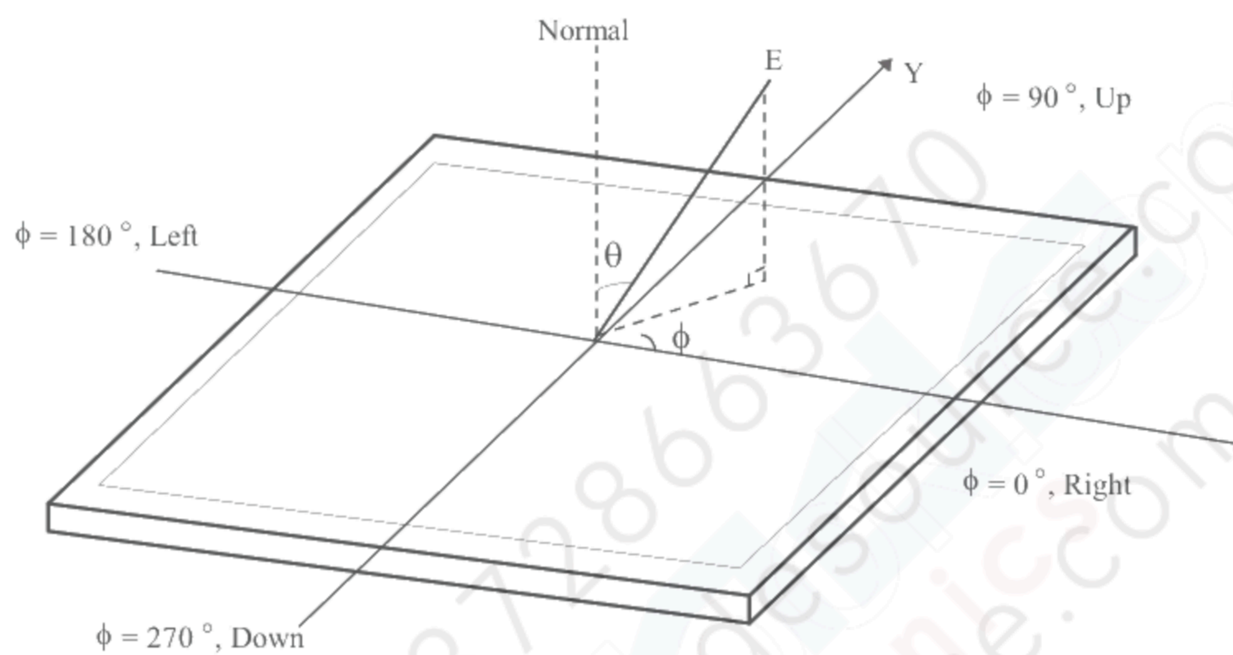
FIG. 5 Viewing Angle
