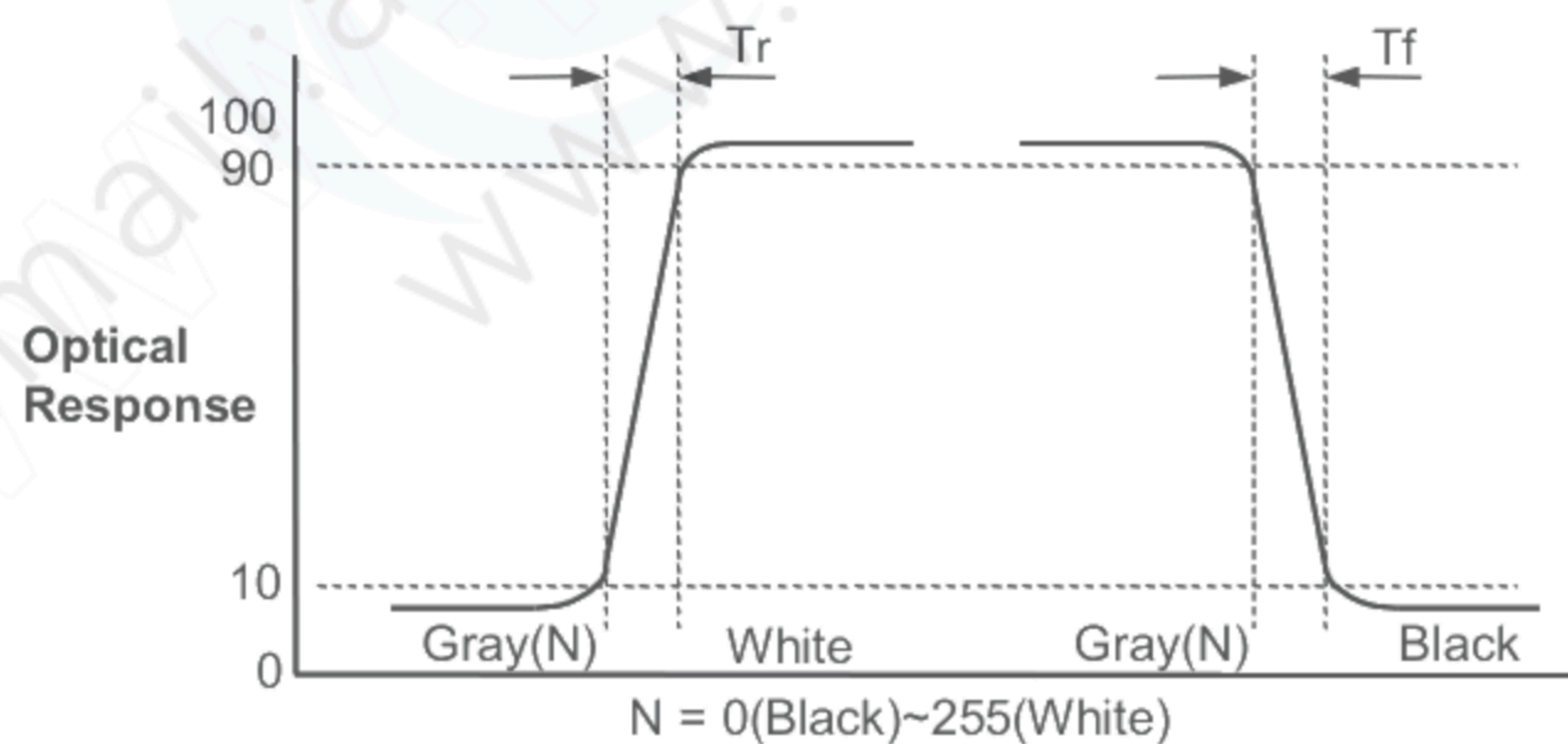
FIG. 4 Response Time
