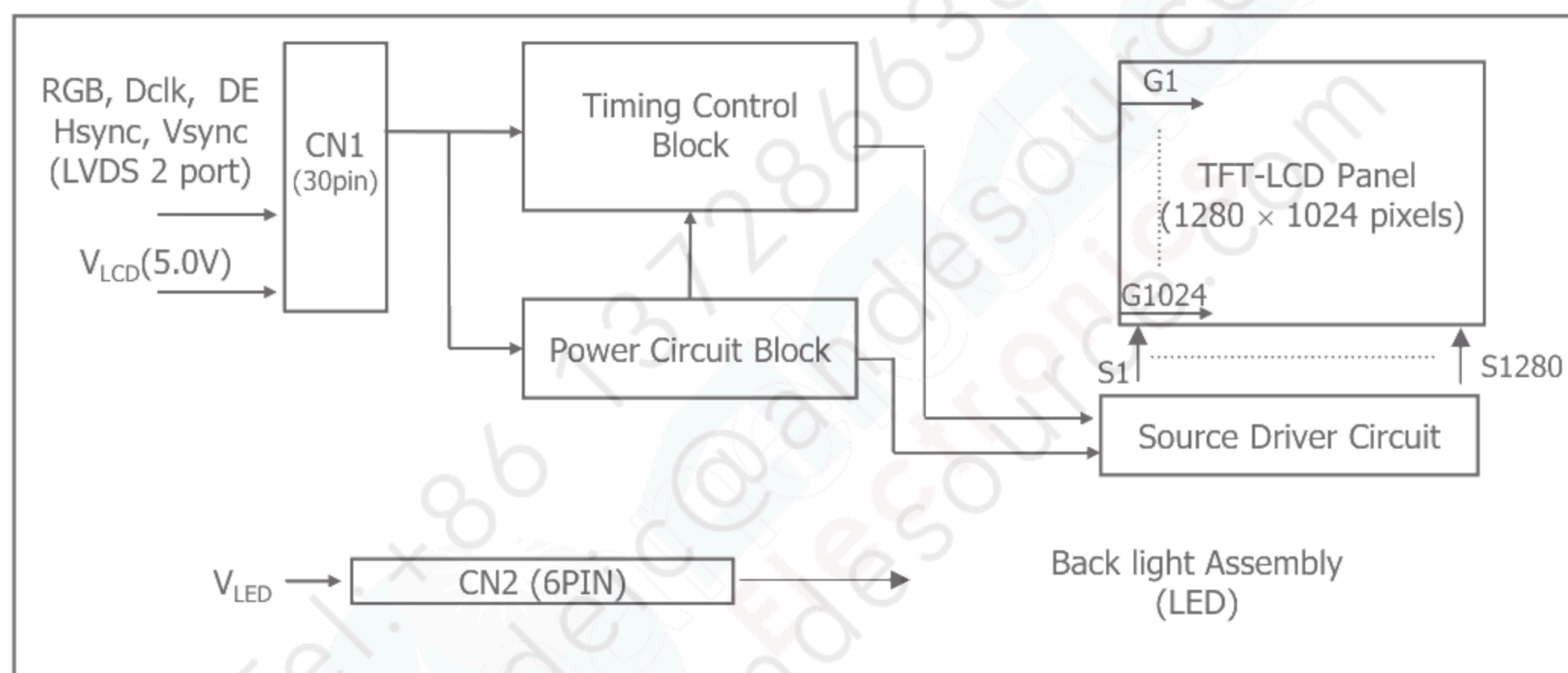
Figure 1. Block diagram
