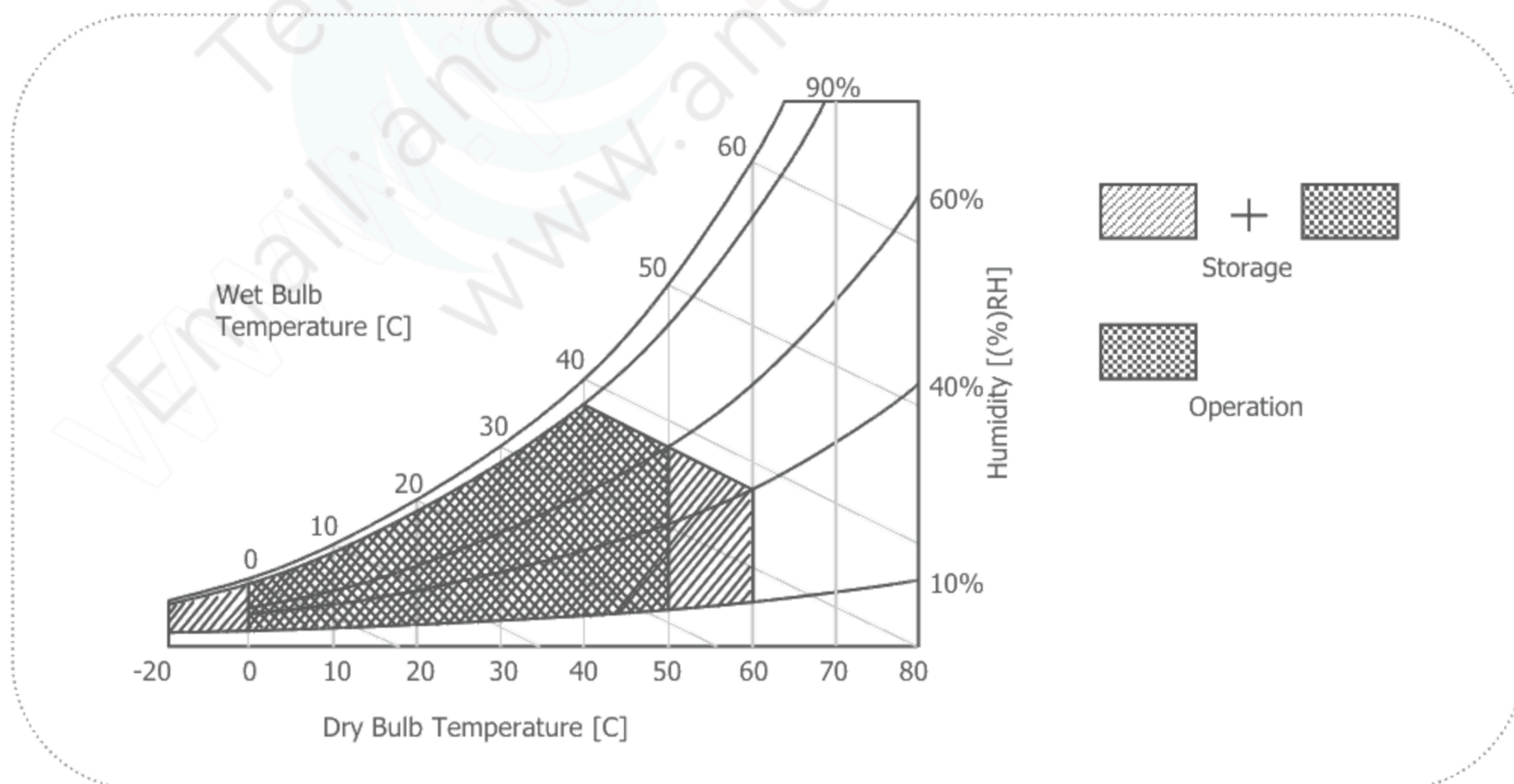
FIG.2 Temperature and relative humidity
