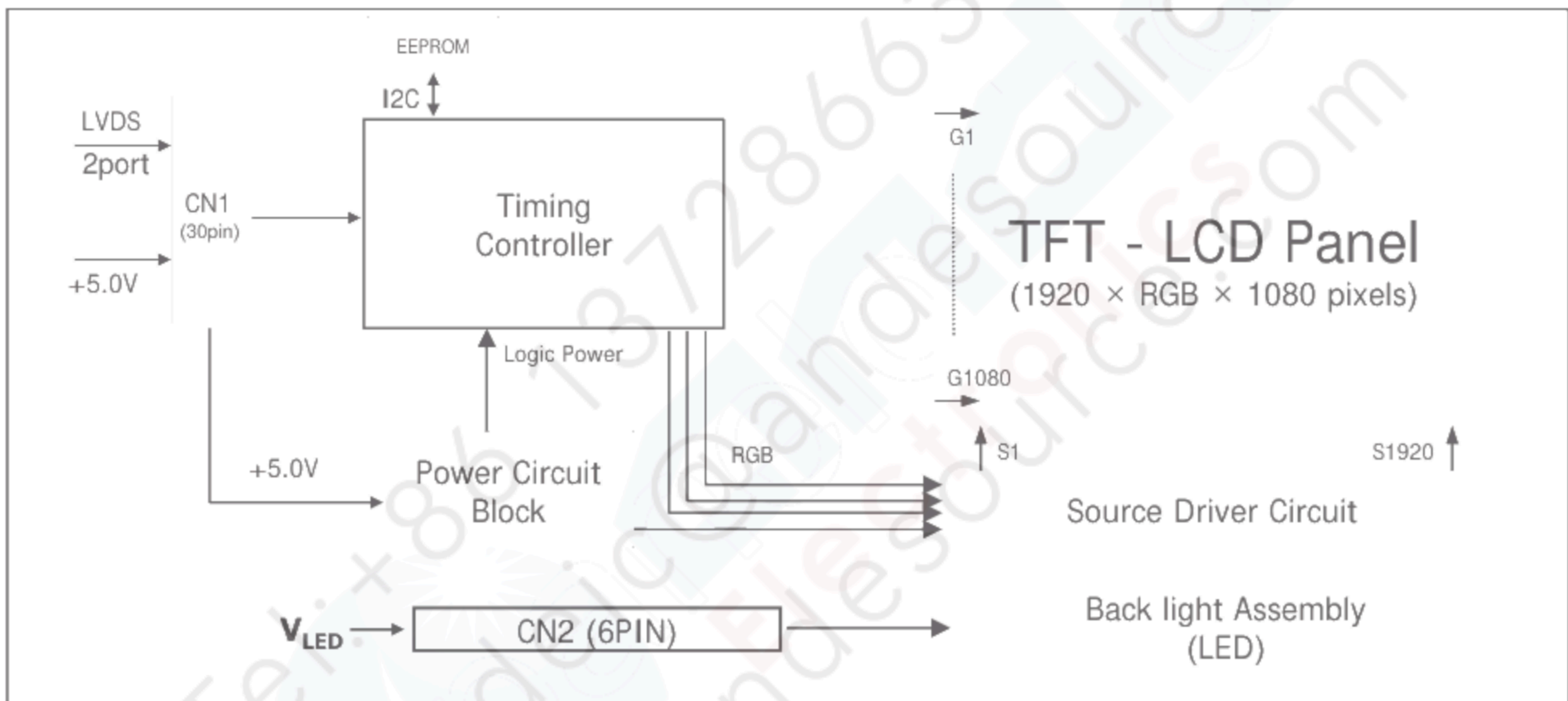
[ Figure 1 ] Block diagram
