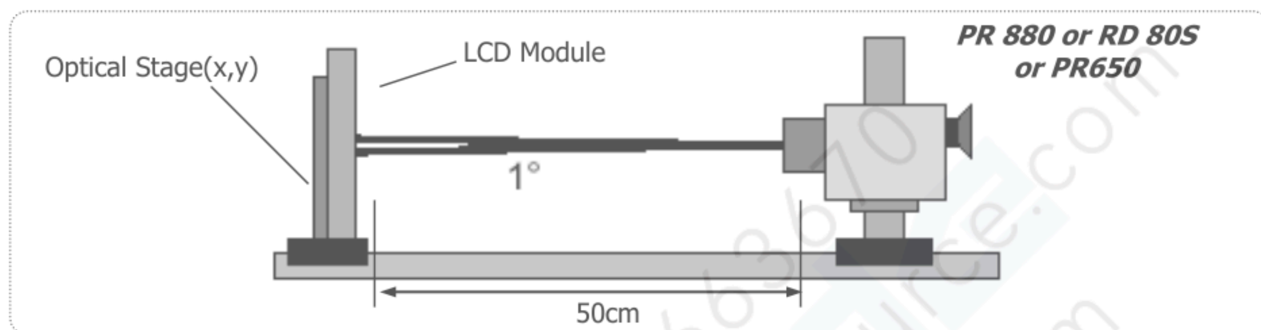
FIG.8 Optical Characteristic Measurement Equipment and Method
