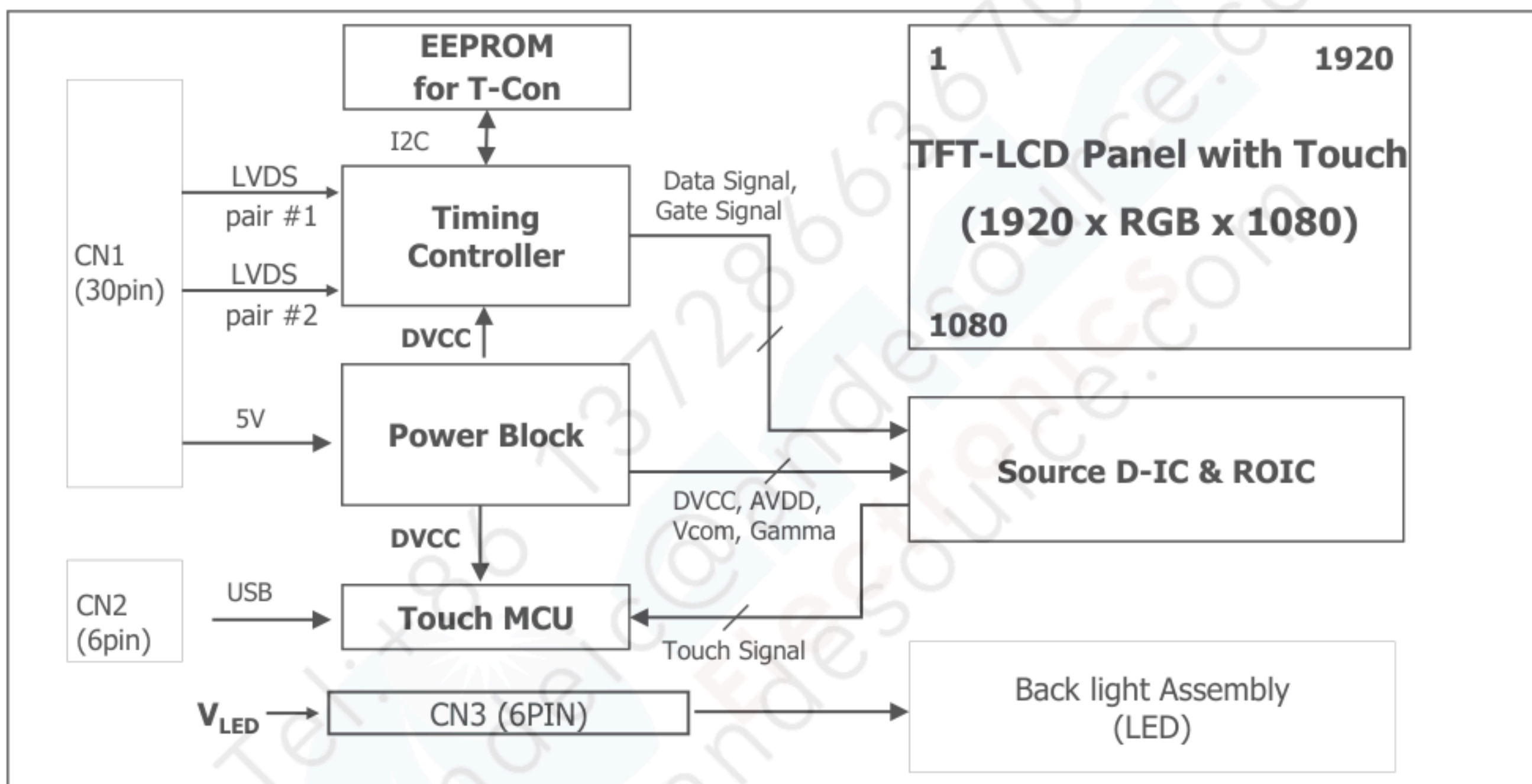
[ FIG. 1 ] Block diagram
