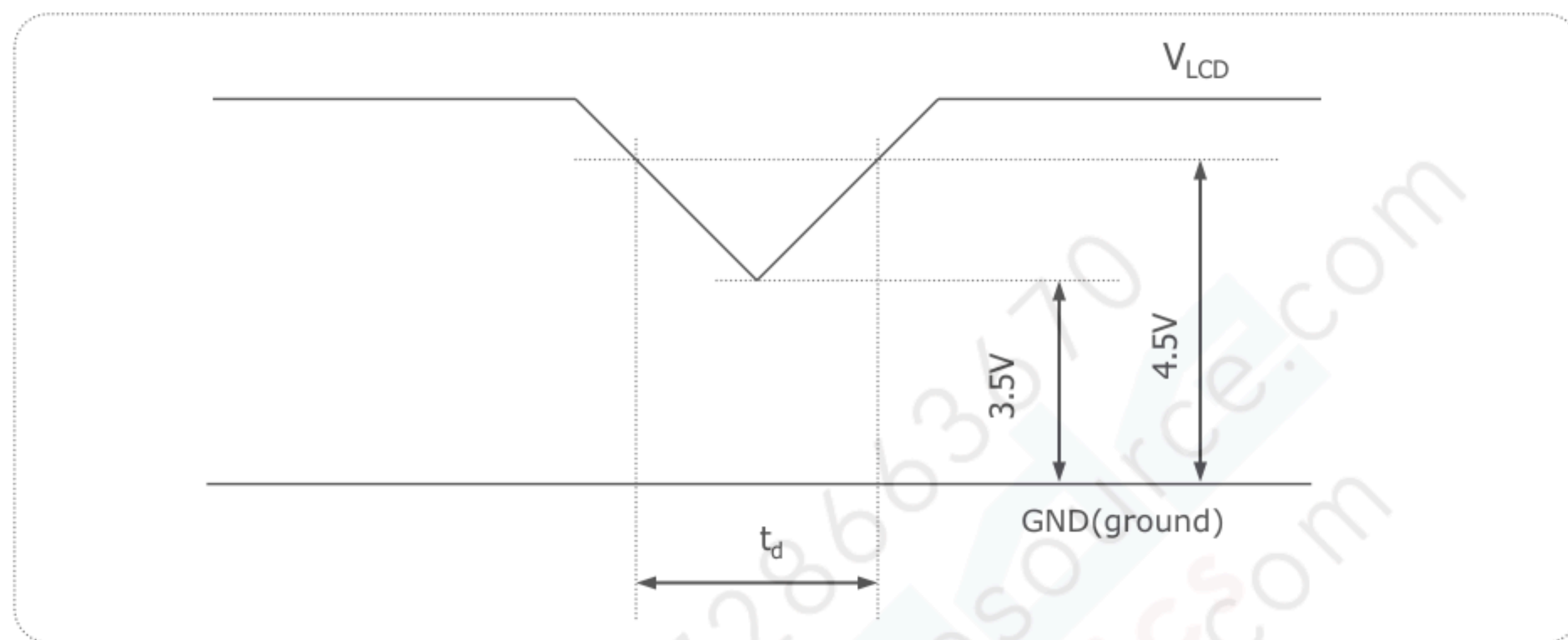
[FIG. 7] Power dip condition
