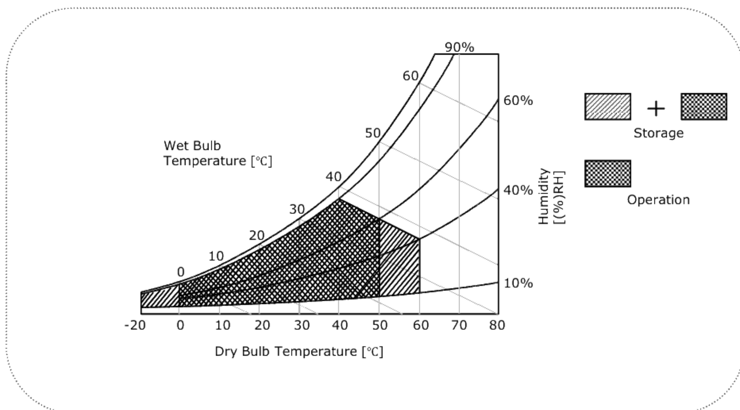
FIG. 2 Temperature and relative humidity
