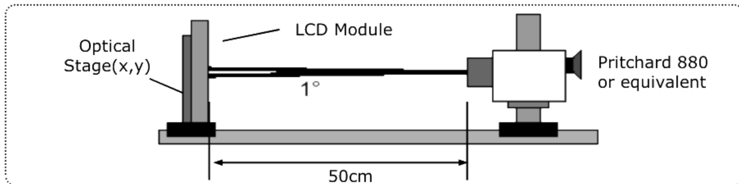
FIG. 7 Optical characteristic measurement equipment and method
