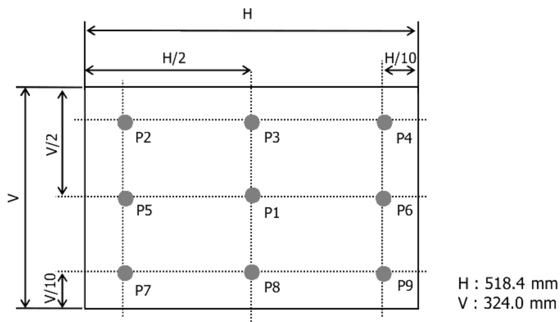
FIG. 8 Measure Point for Luminance
