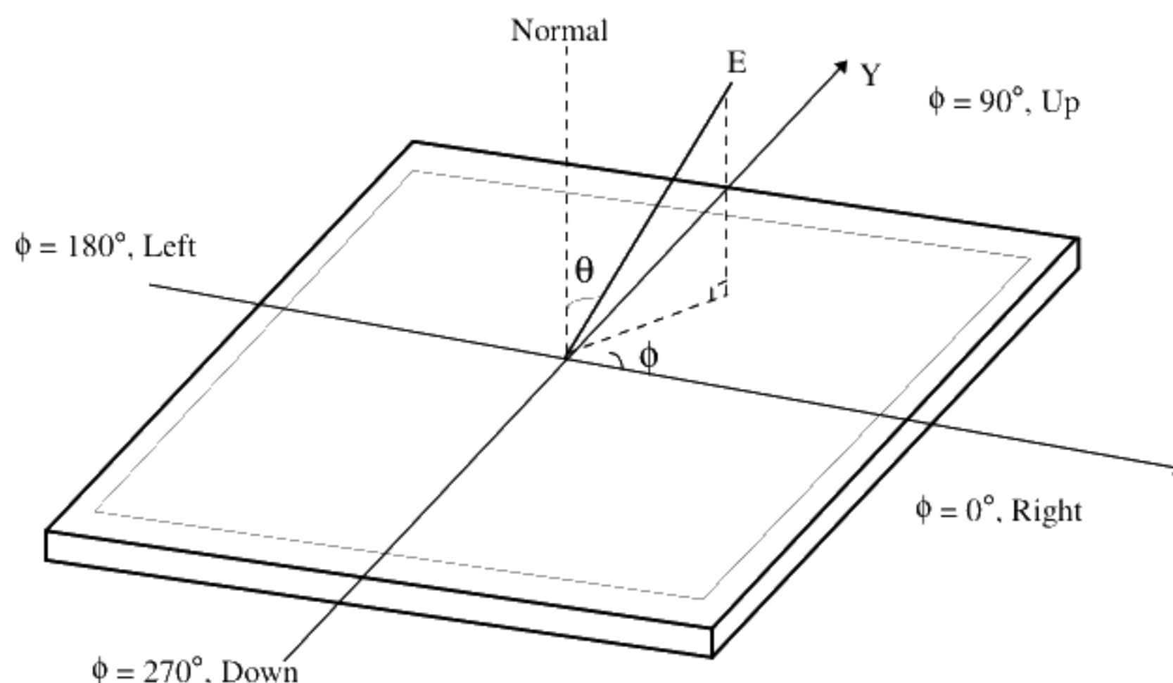
FIG. 10 Viewing angle
