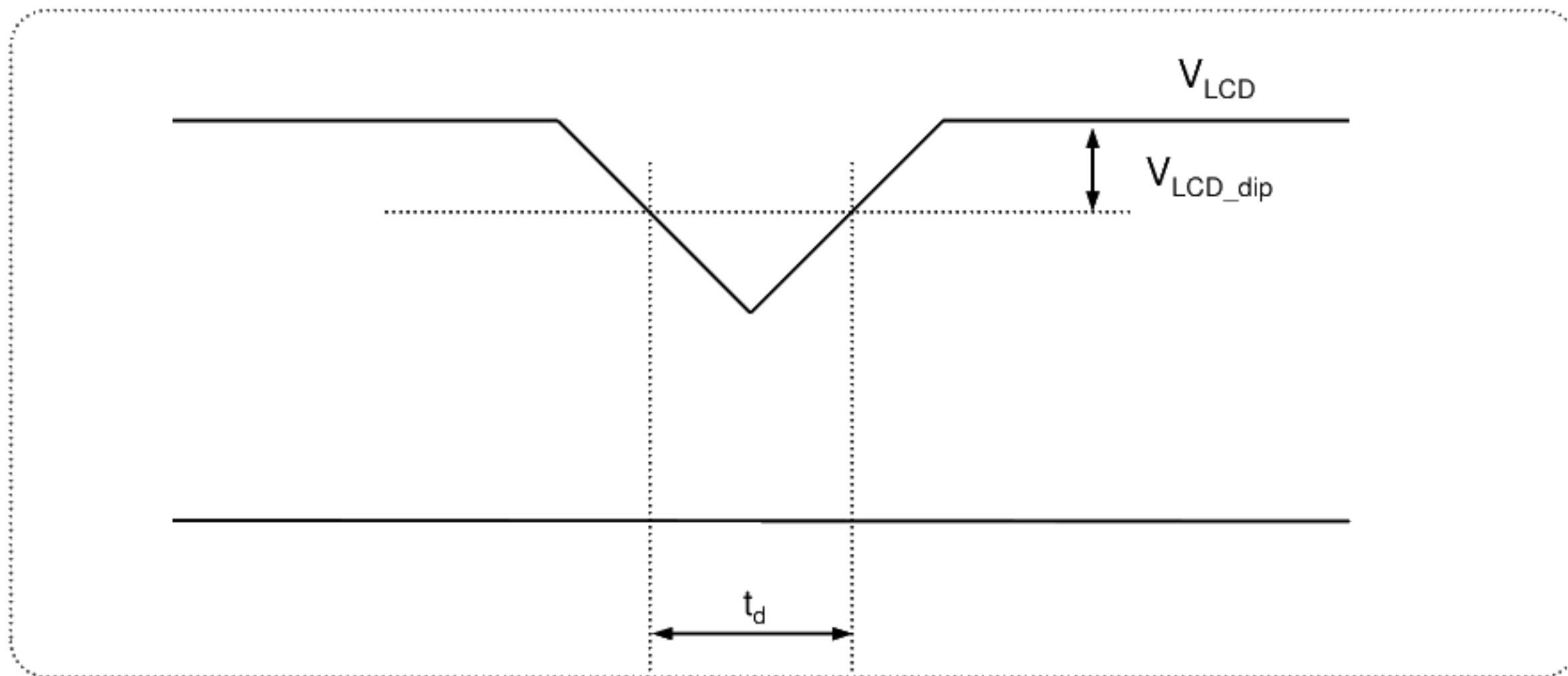
FIG. 6 Power dip condition
