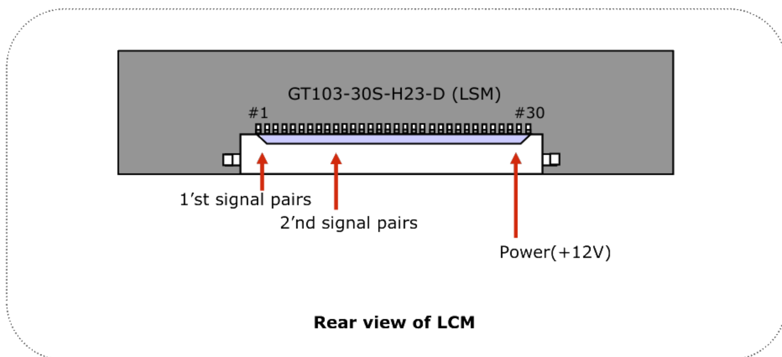
FIG. 4 Connector diagram
