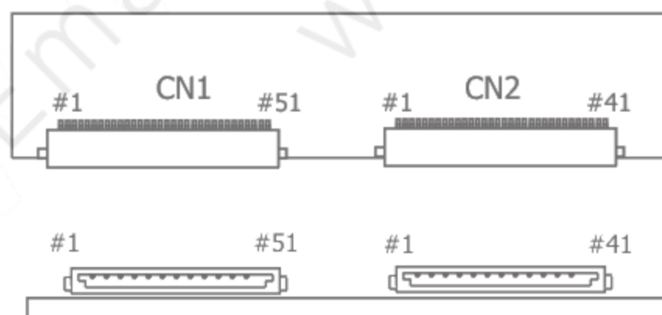
Rear view of LCM
