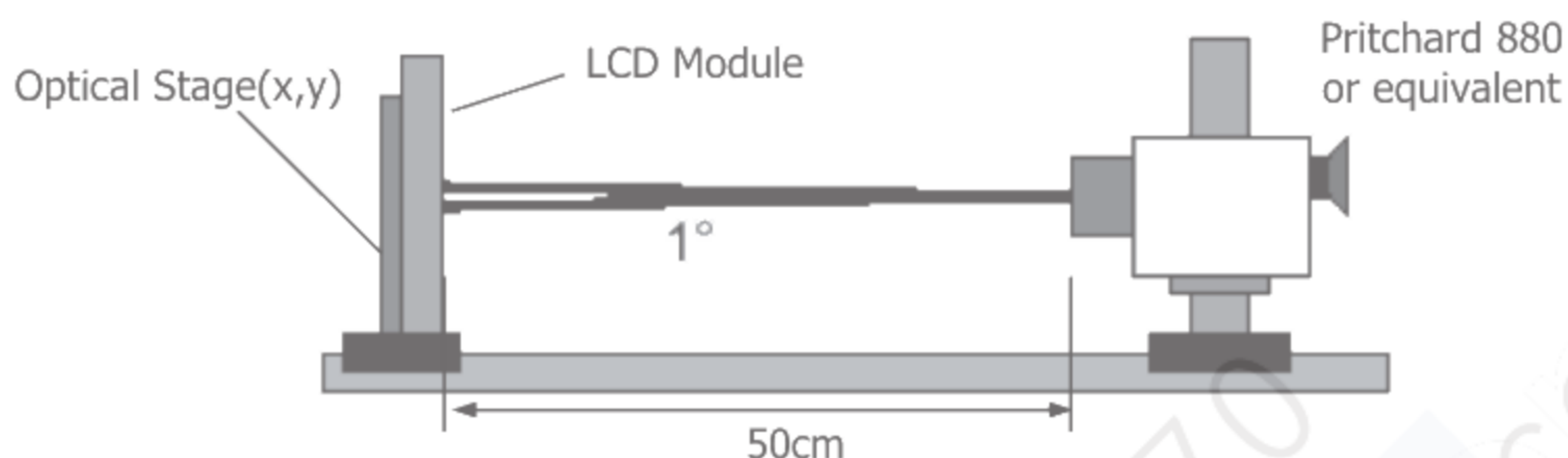
FIG. 2 Optical Characteristic Measurement Equipment and Method
