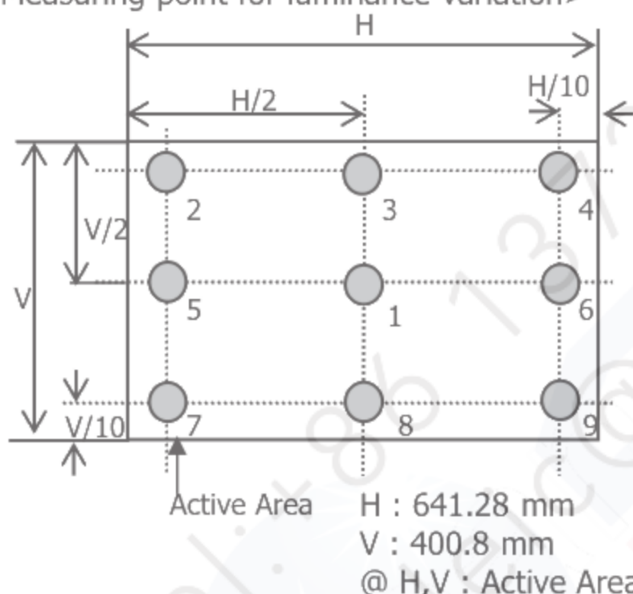
FIG. 3 Measure Point for Luminance
