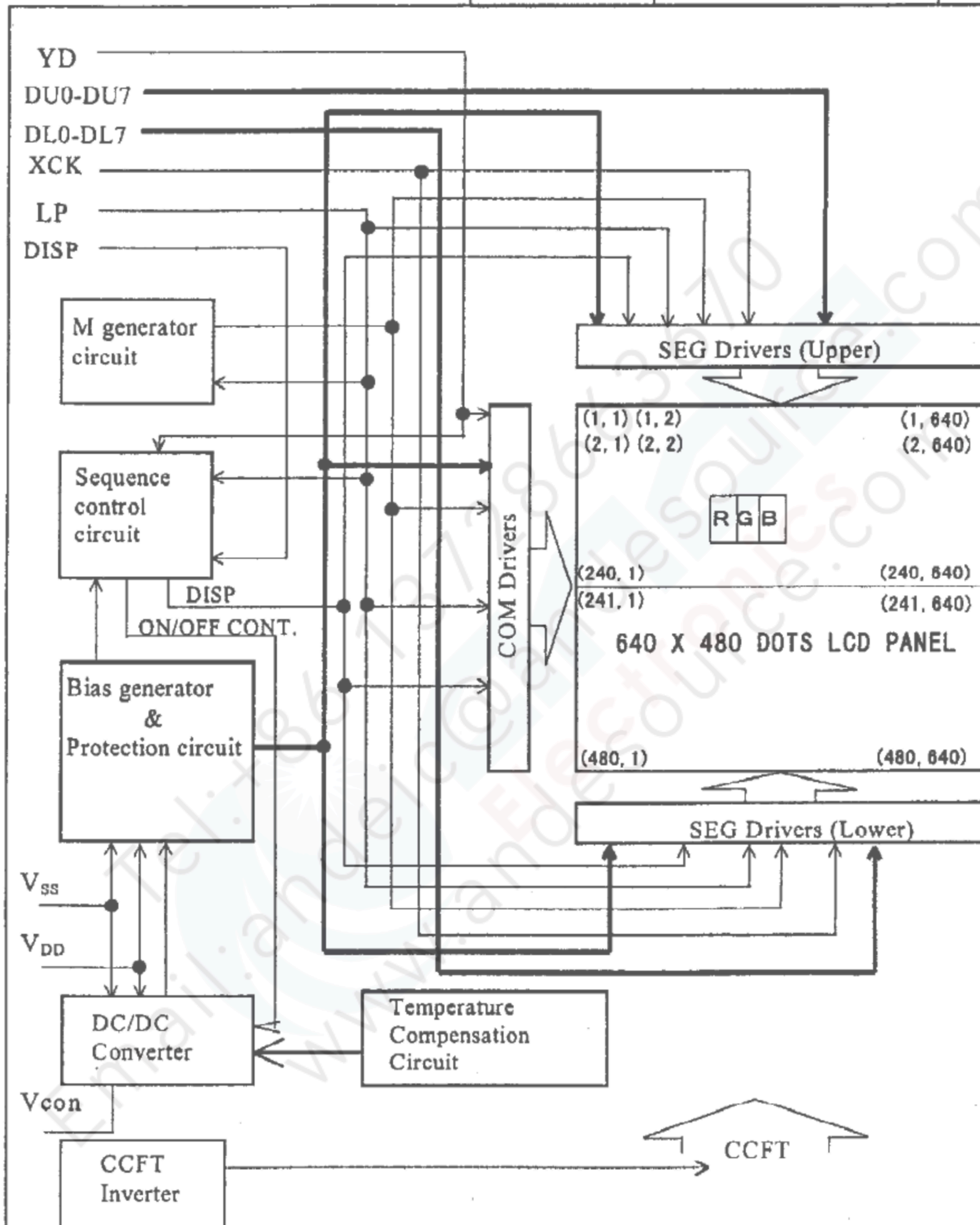
Fig. 10 Circuit block diagram
