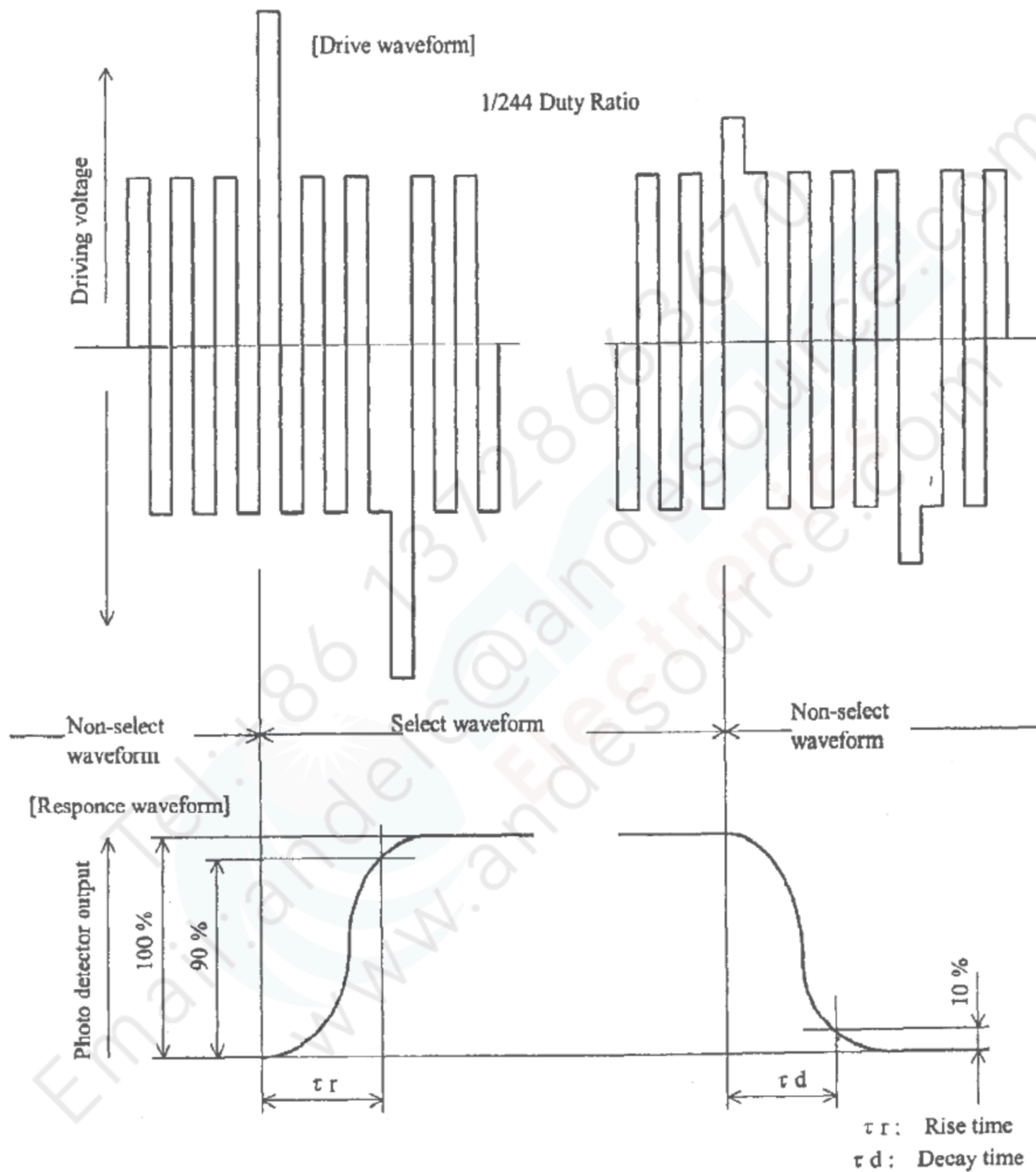
Fig.9 Definition of Response time
