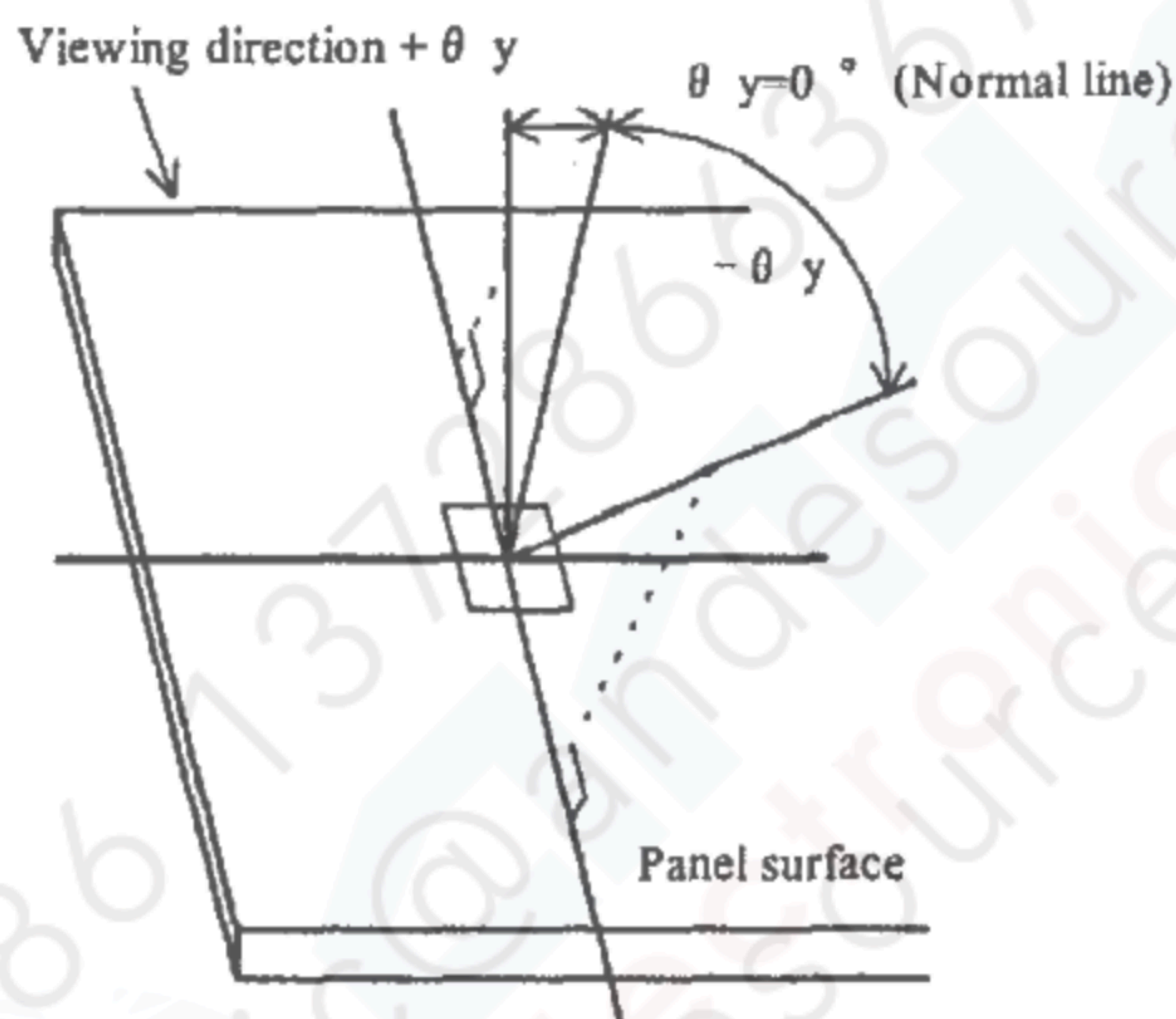
Fig.1 Definition of viewing angle
