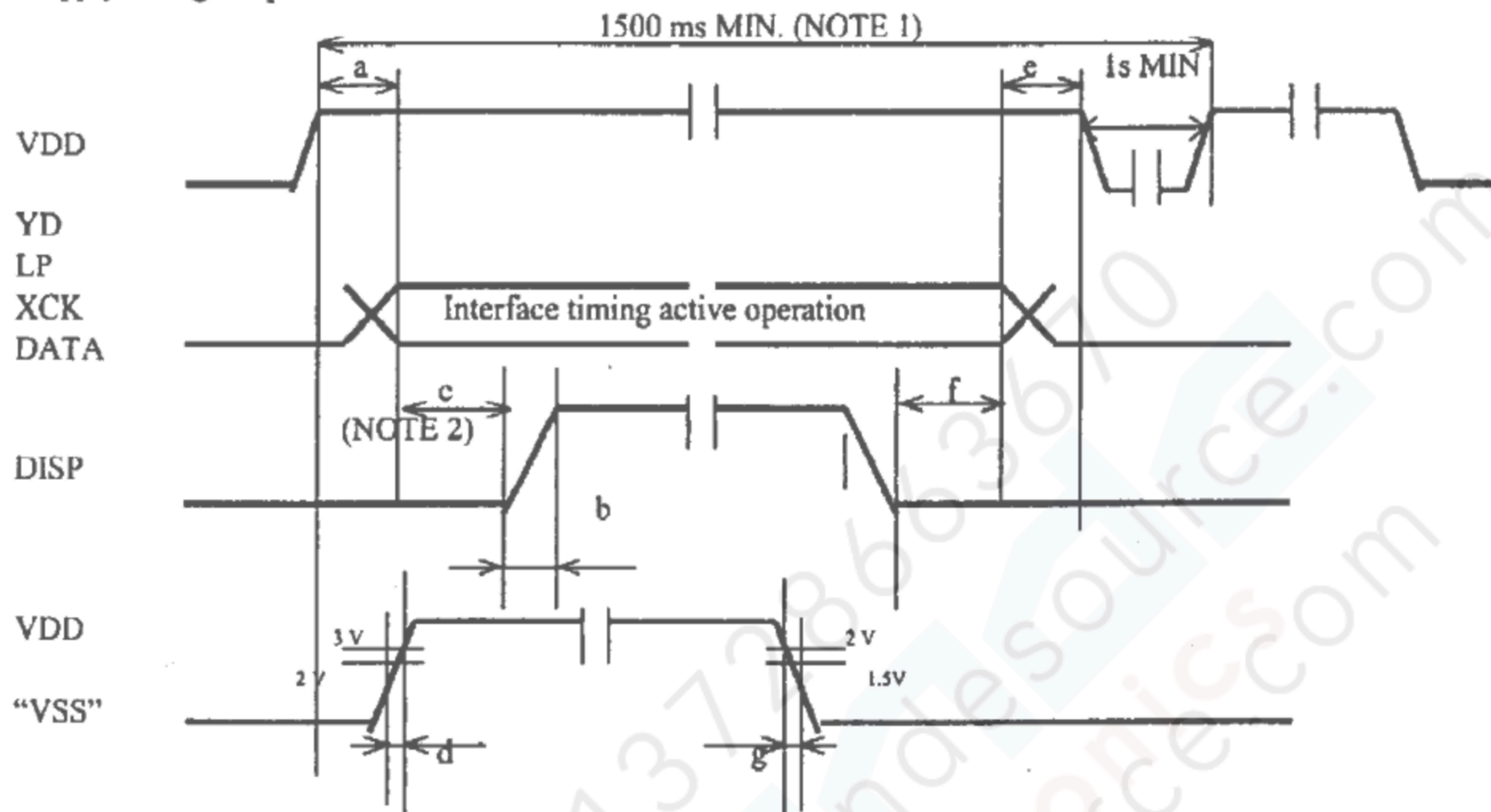
Fig.12 Supply voltage sequence condition
