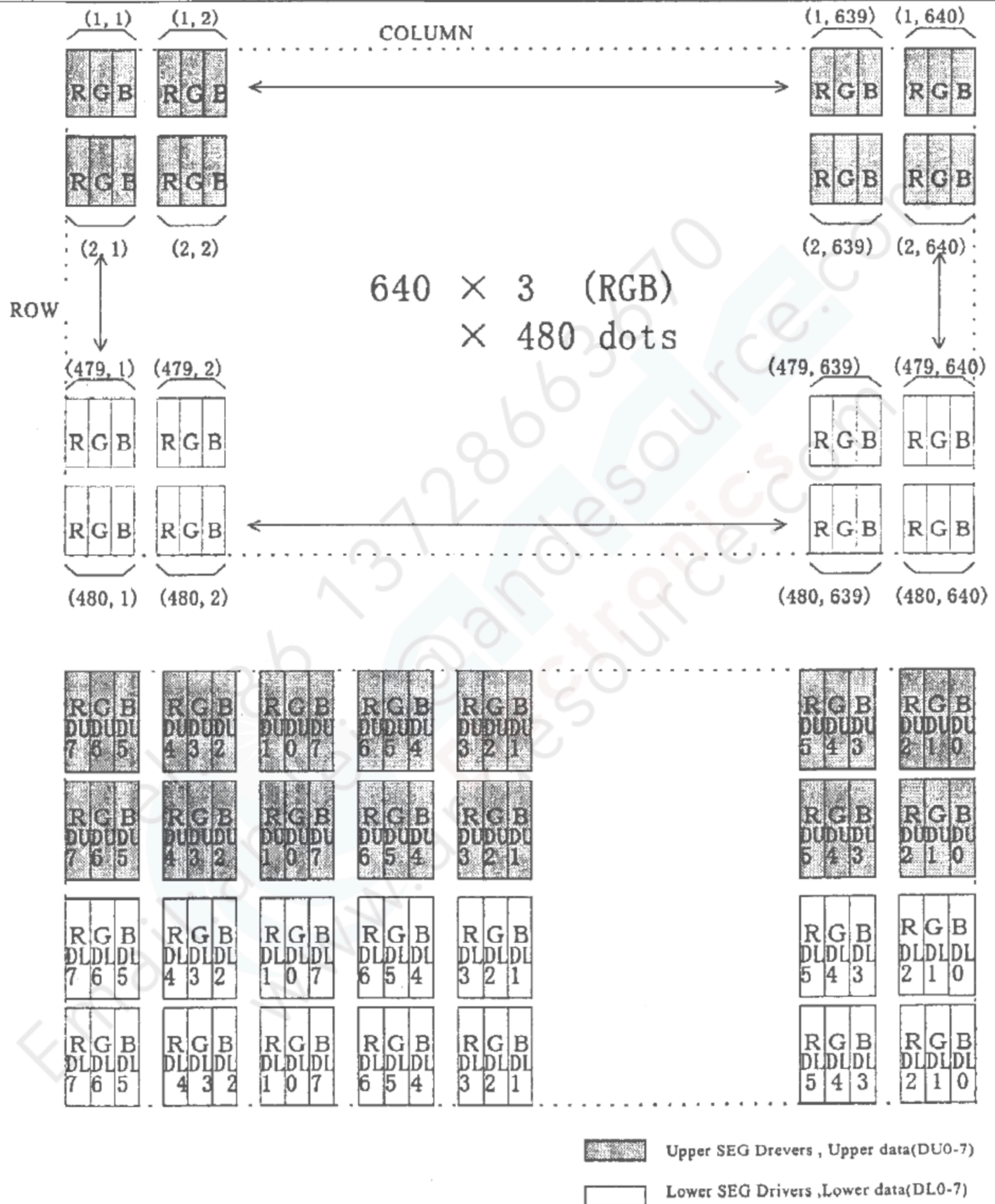
Fig.2 Dot chart of display area
