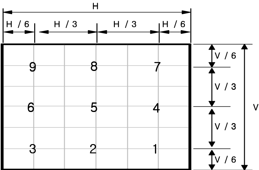
The spot locations for luminance measurement
