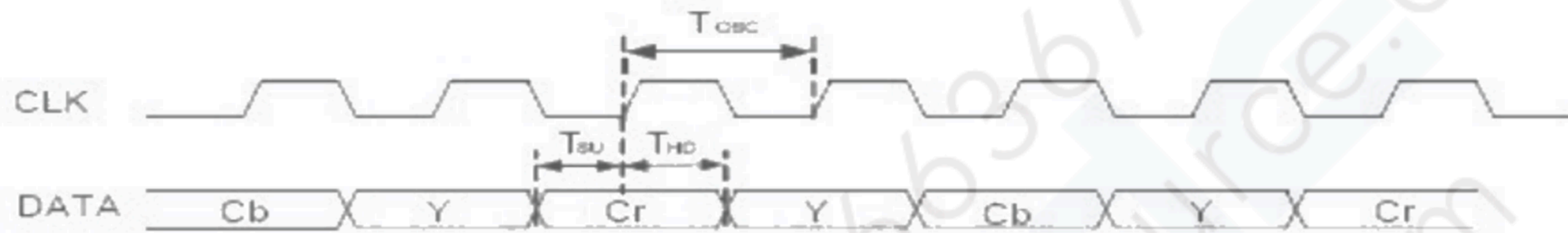
Figure2 CLK and DATA waveforms in CCIR656
