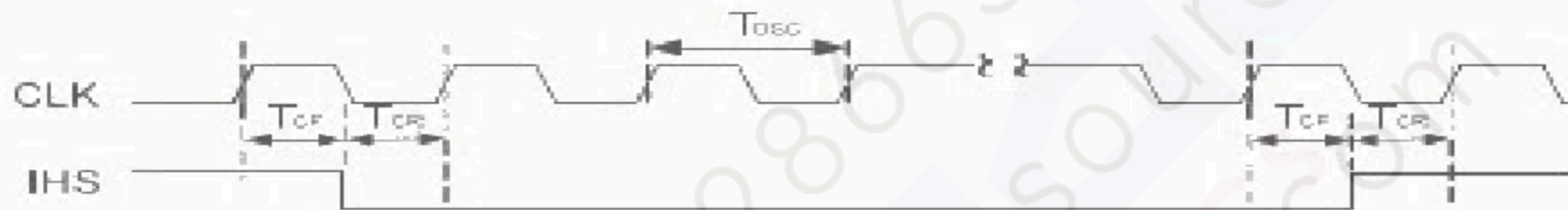
Figure6 CLK and IHS timing waveform
