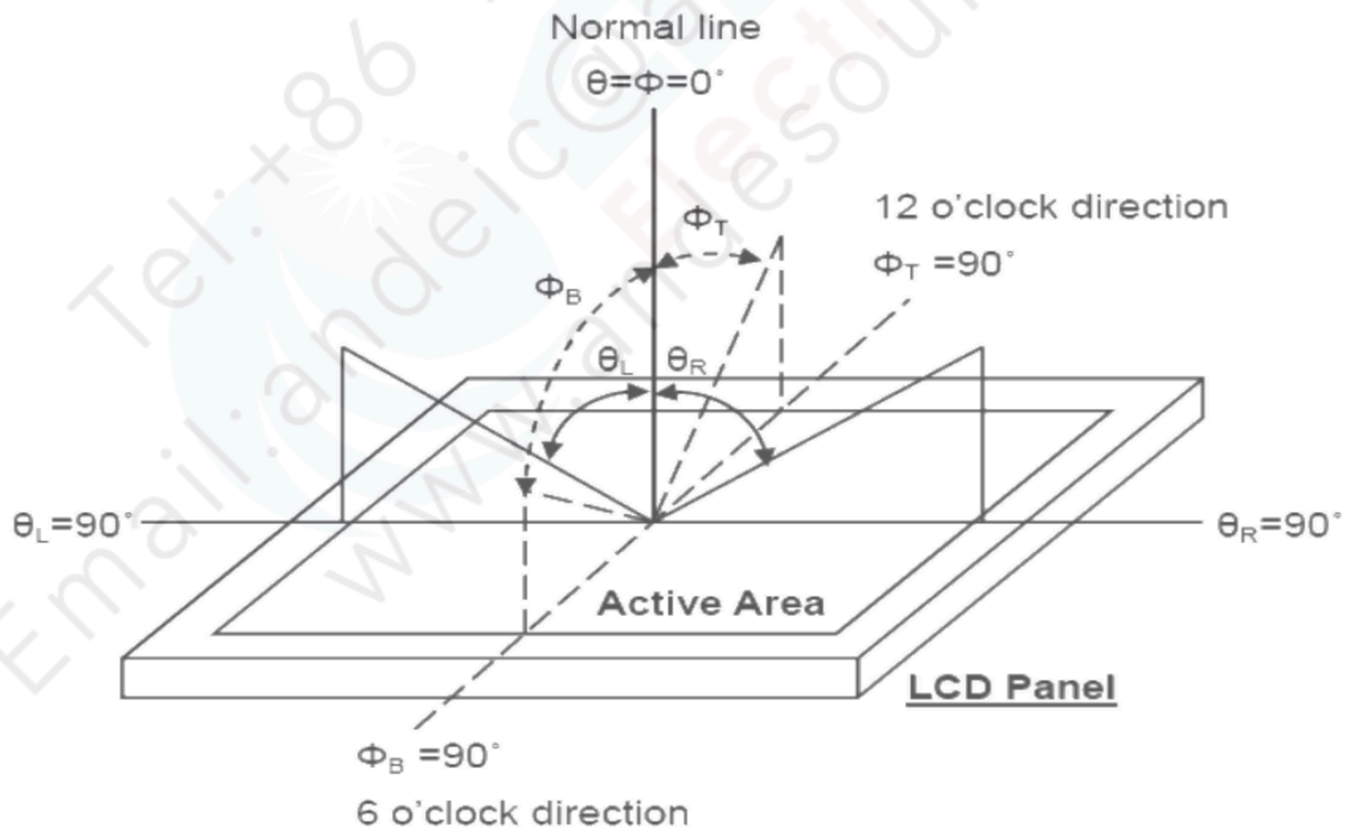
Fig. 8-1 Definition of viewing angle
