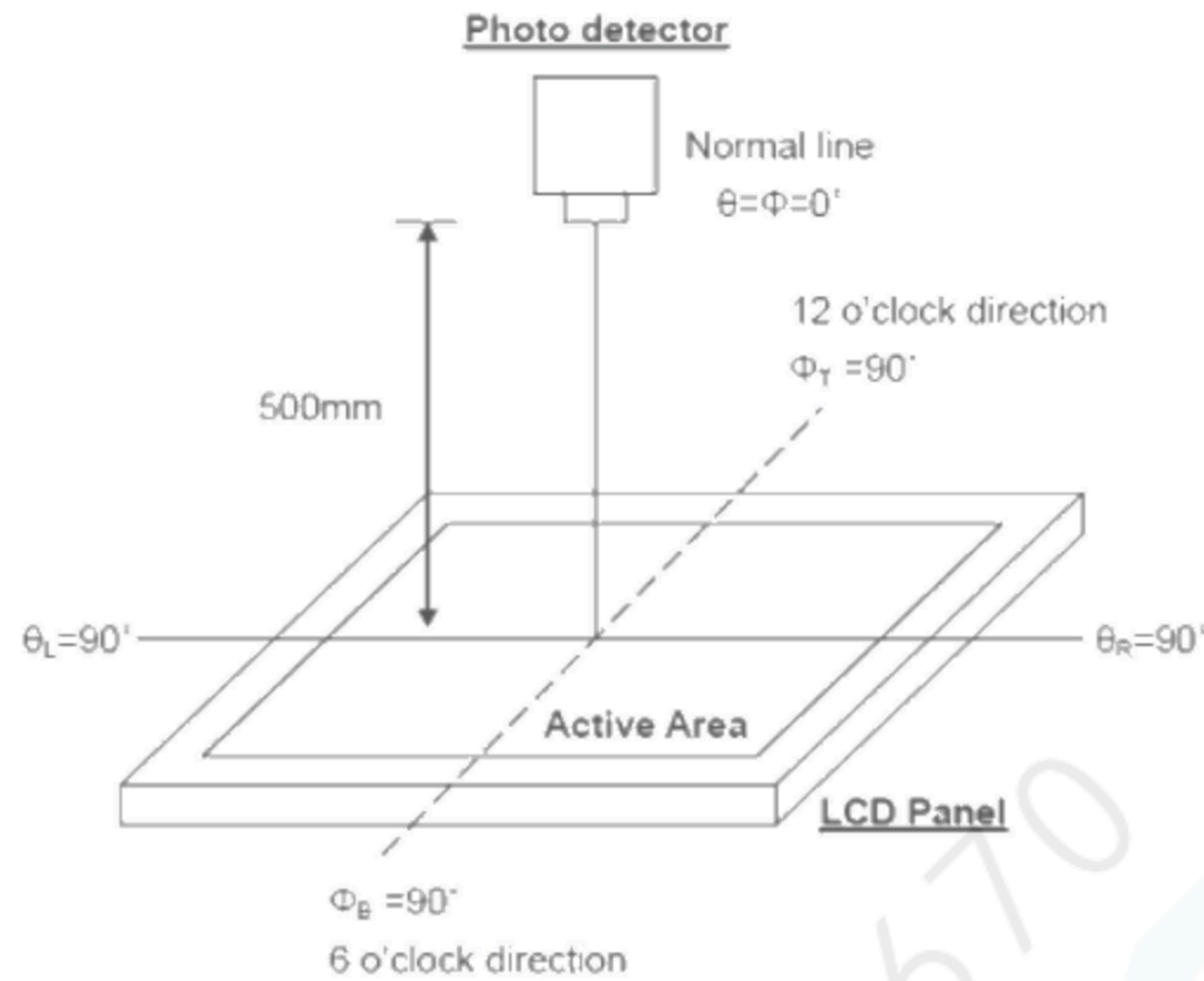
Fig. 8-2 Optical measurement system setup
