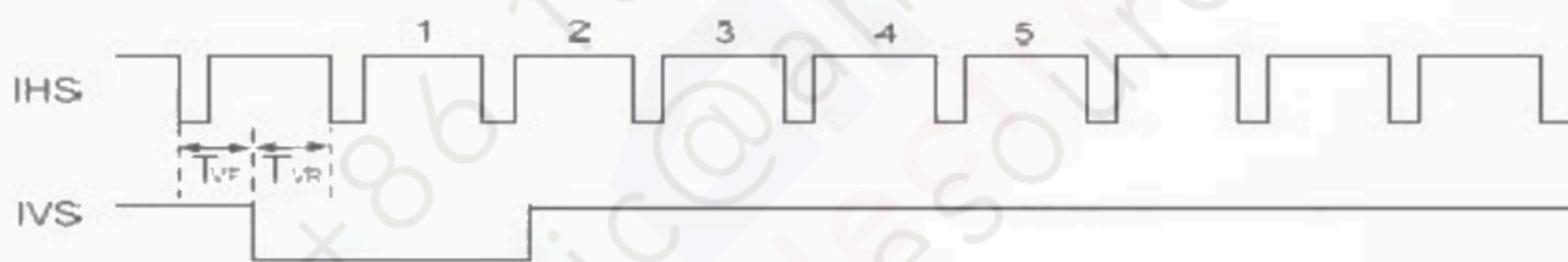
Figure7 IHS and IVS timing waveforms
