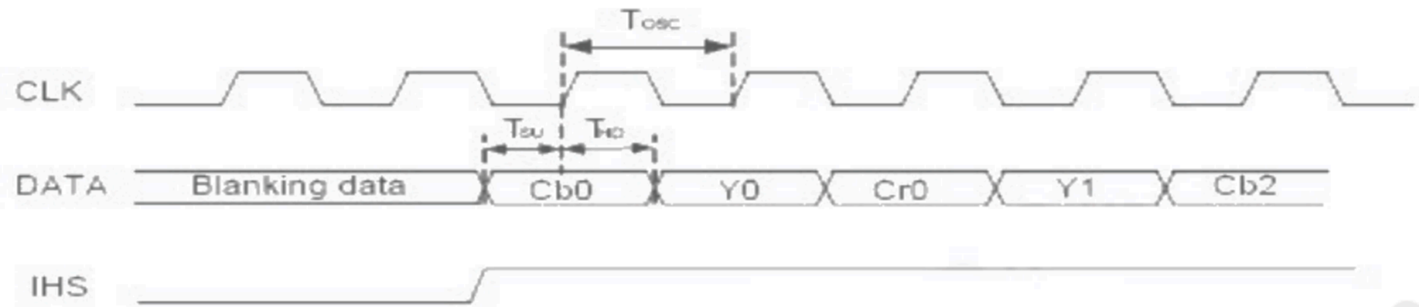
Figure1 CLK,DATA and HIS waveforms in CCIR601
