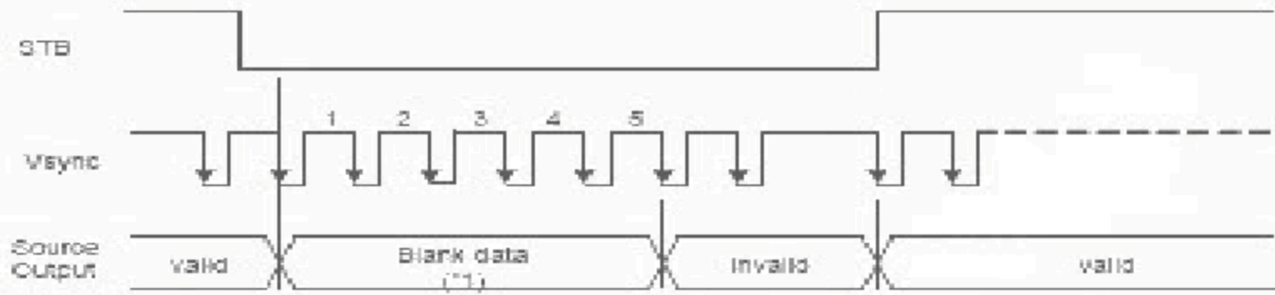
Figure5 Standby ON/OFF Control
