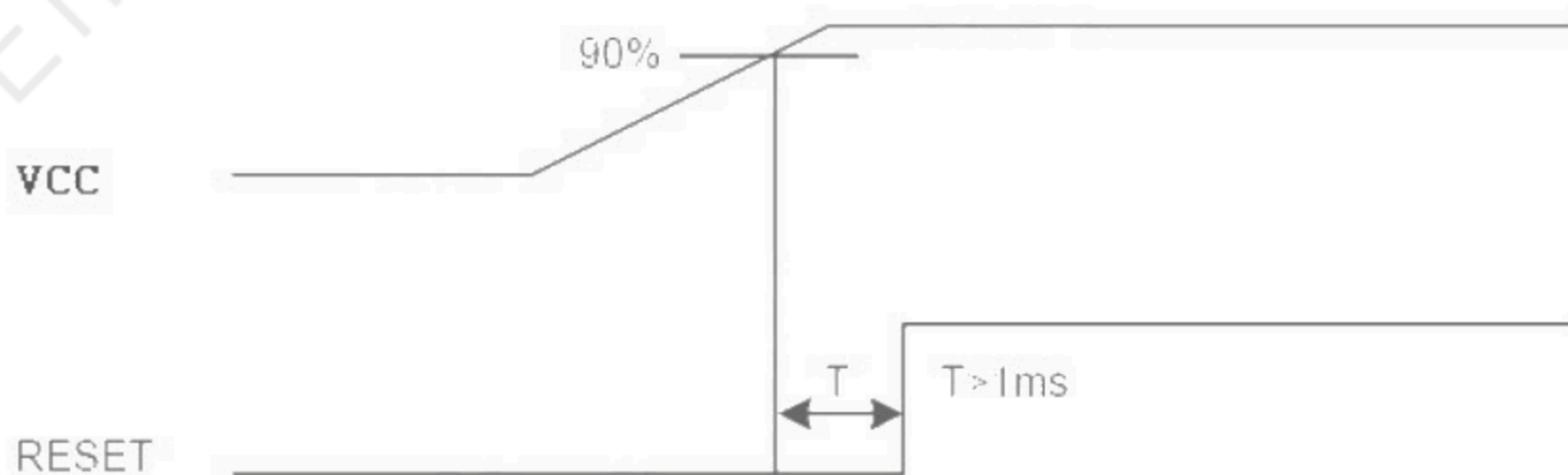
Reset timing
