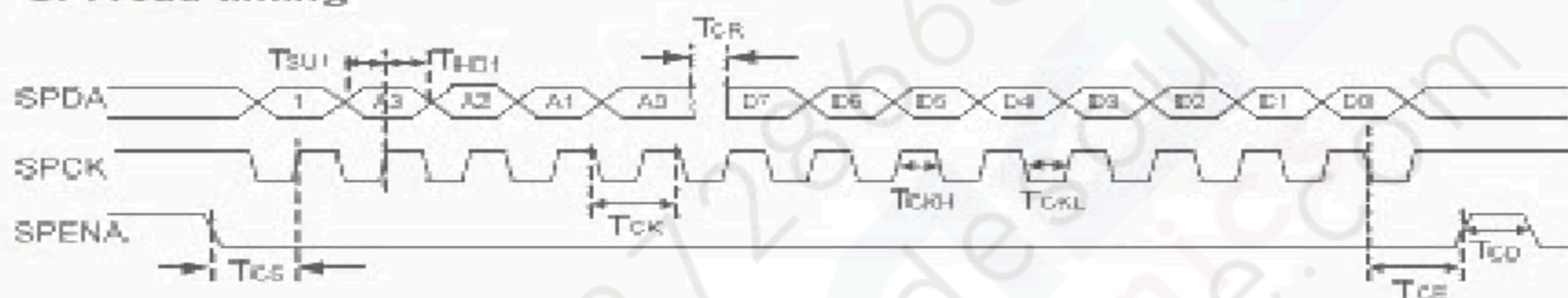
Figure8 SPI read timing
