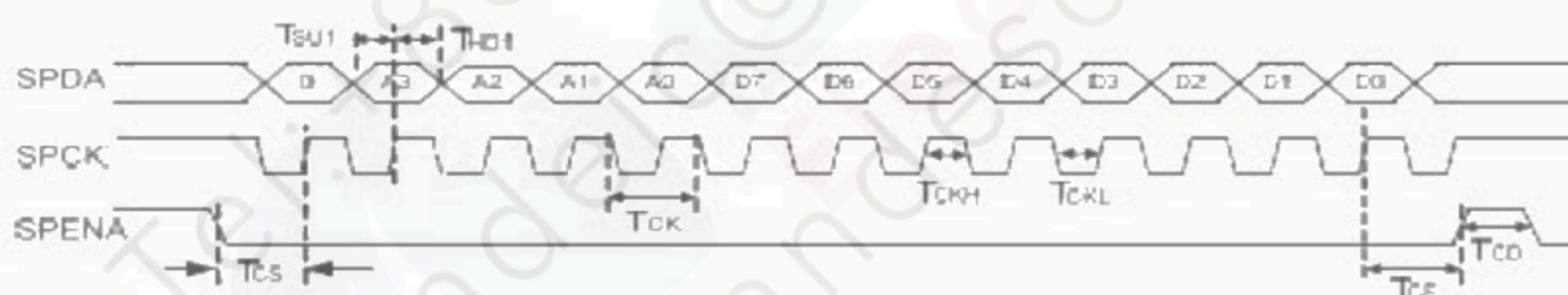
Figure9 SPI write timing
