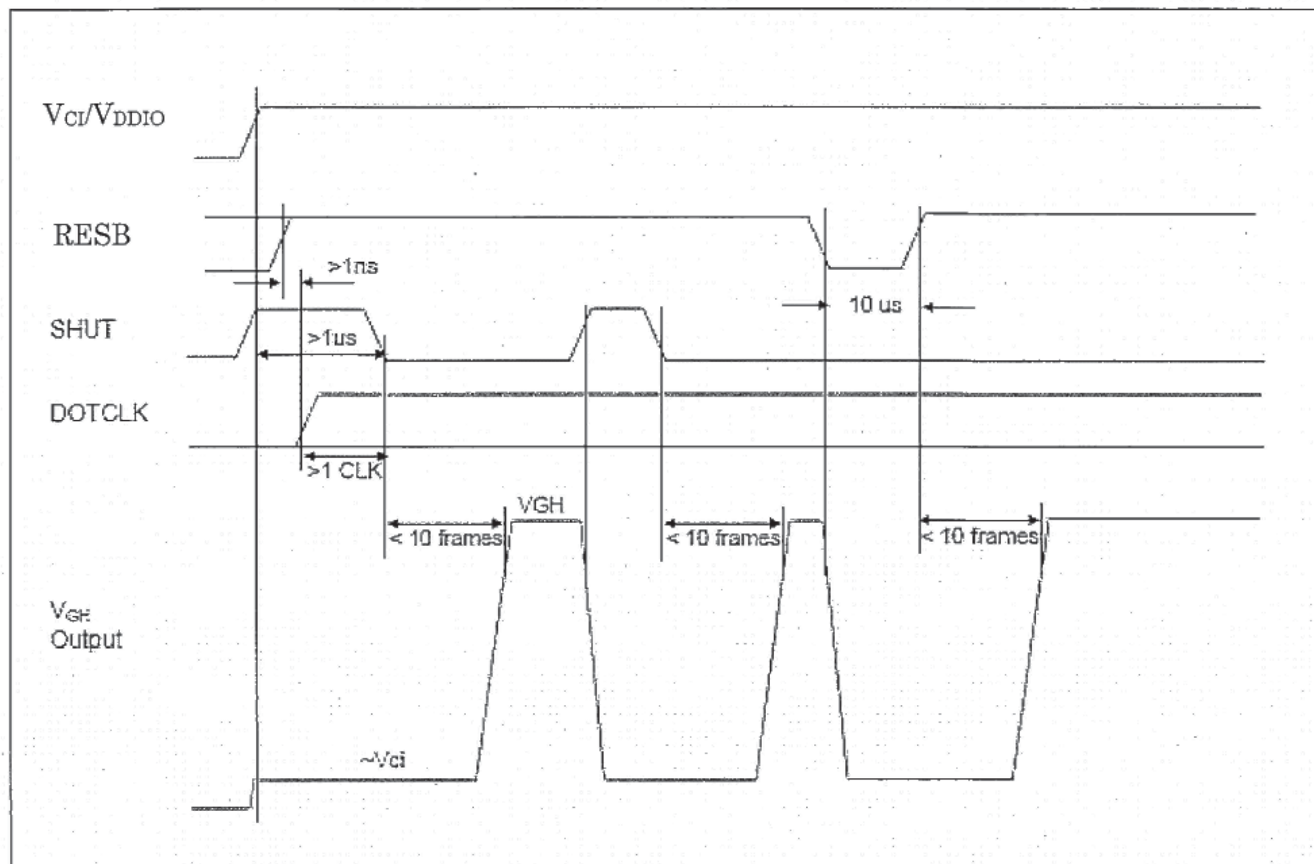
VGH Output against SHUT &amp; RESB
