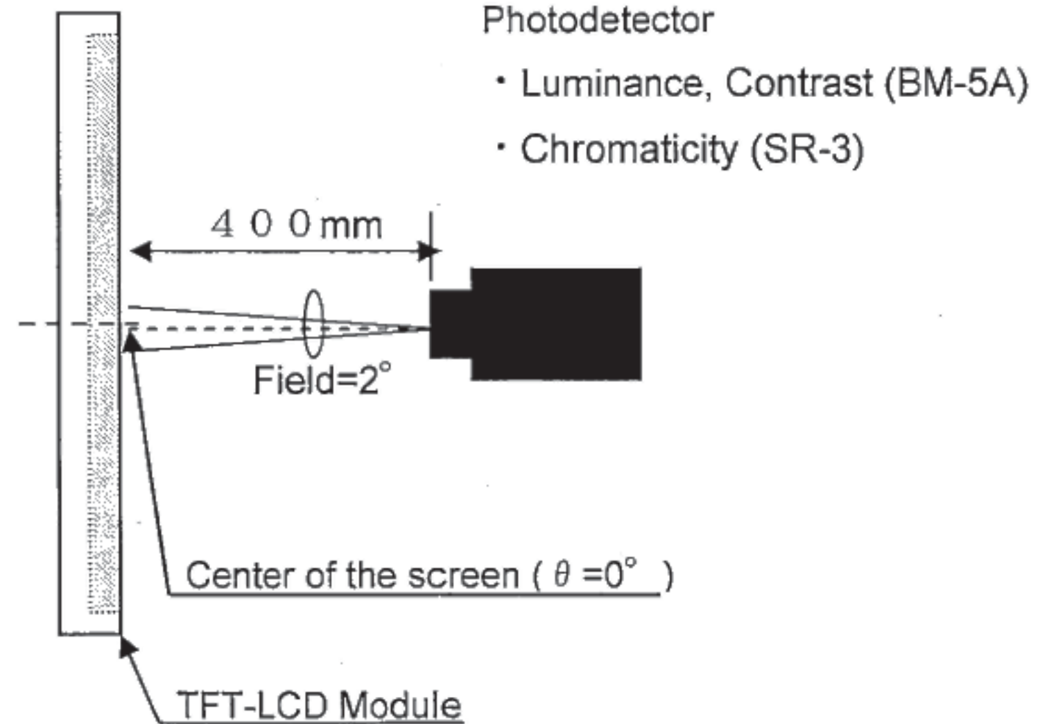
Fig.9-2 Measuring setup for Luminance, Chromaticity and Response time
