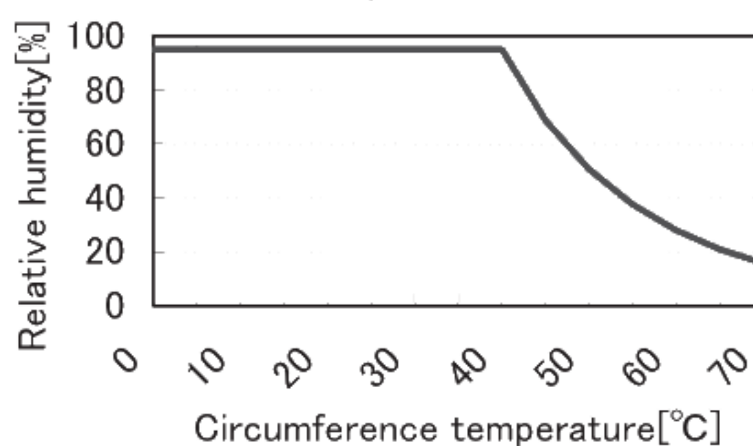
Humidity guarantee range (Wet-bulb temperature:39°C)
