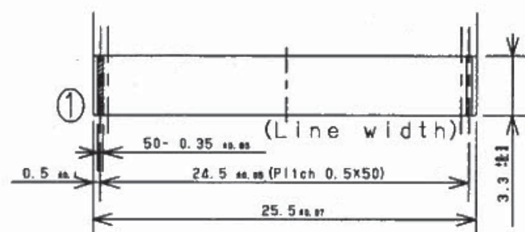
LCD FPC TERMINAL'S
