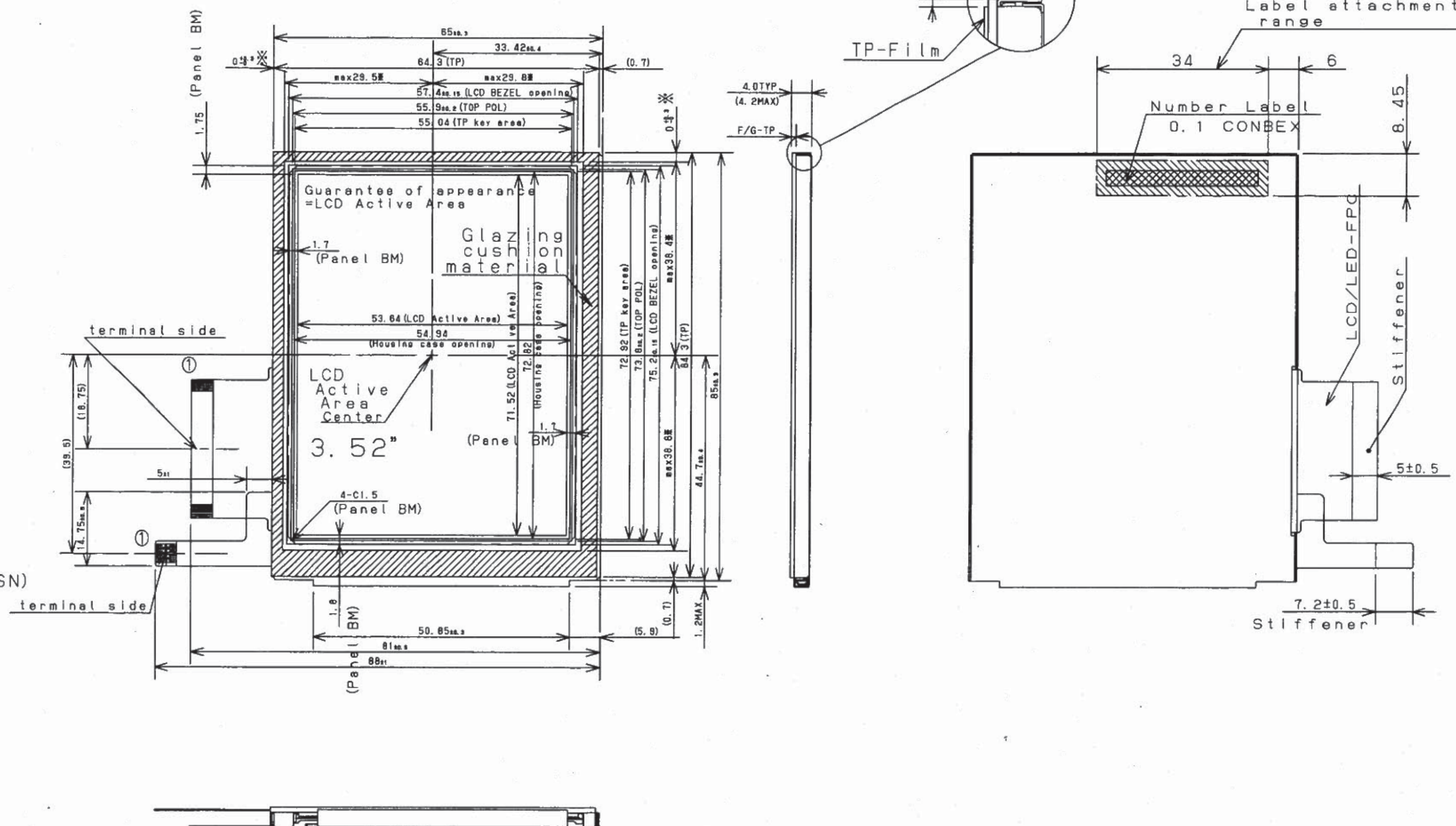
Fig.1 Outline Dimensions
