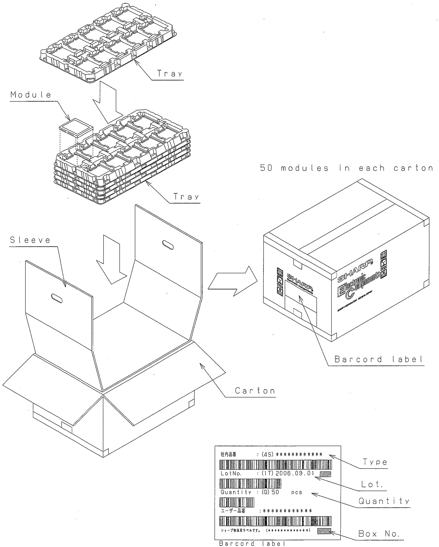
Fig.2 PACKING FORM
