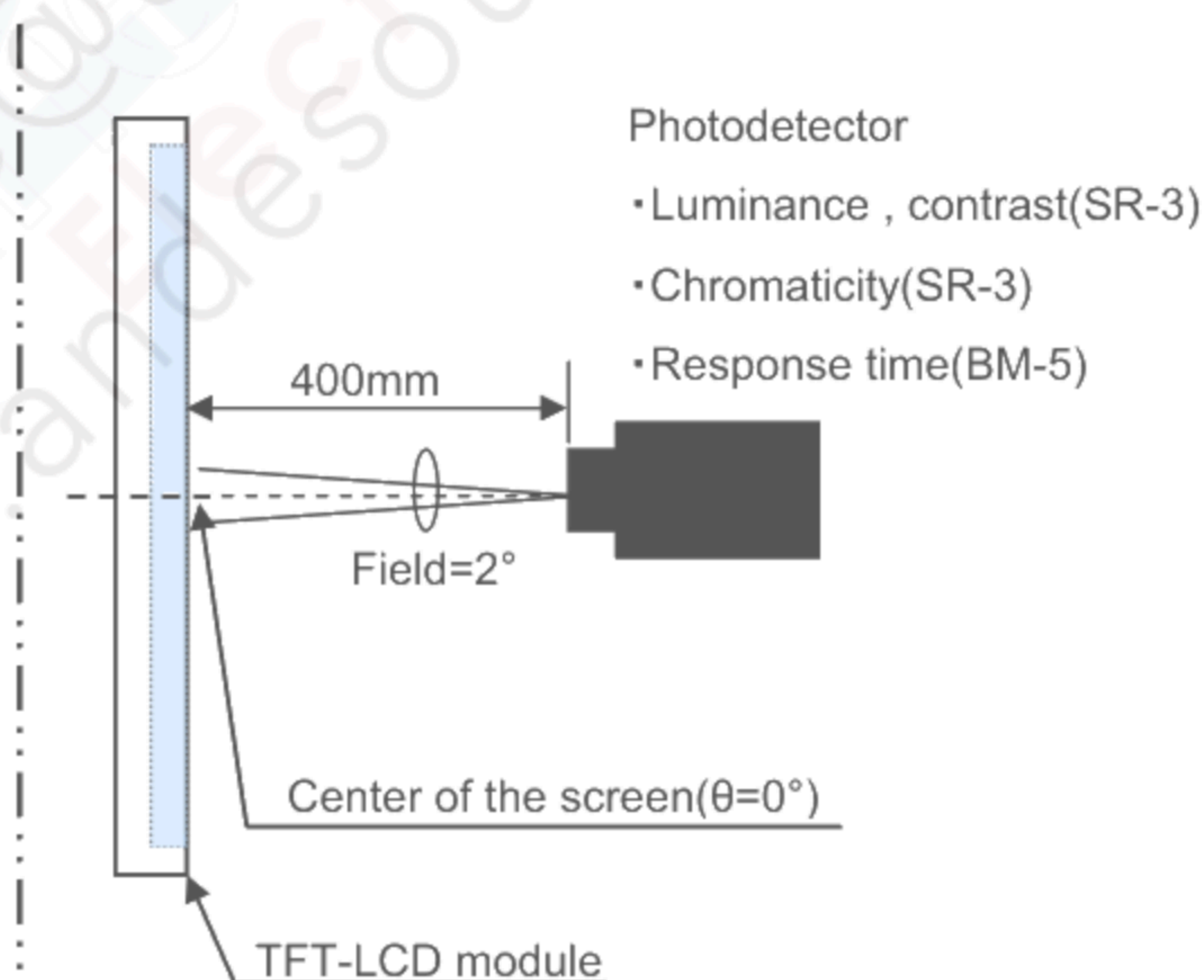
Fig.9-2 Luminance / Contrast/Chromaticity / Response time measurement method
