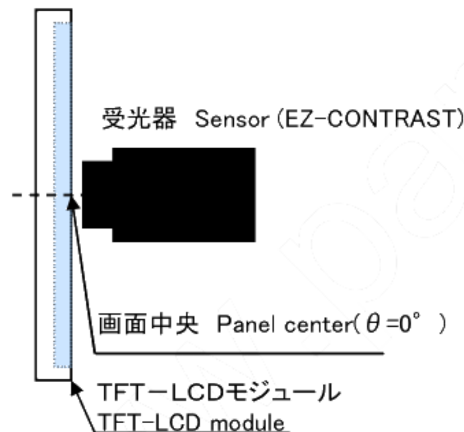
図9-1 視角範囲測定方法 Fig.9-1 Measuring setup for Viewing angle
