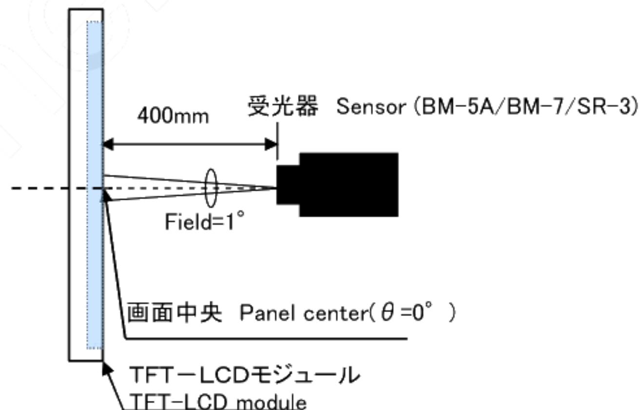
図9-2 輝度/色度/応答速度測定方法 (応答速度: BM-5A/7、輝度/色度/コントラスト: BM-5A、SR-3使用) Fig.9-2 Measuring setup for Luminance, Chromaticity and Response time (BM-5A/7 is used for Response time, BM-5A and SR-3 is used for Luminance, Contrast and Chromaticity)
