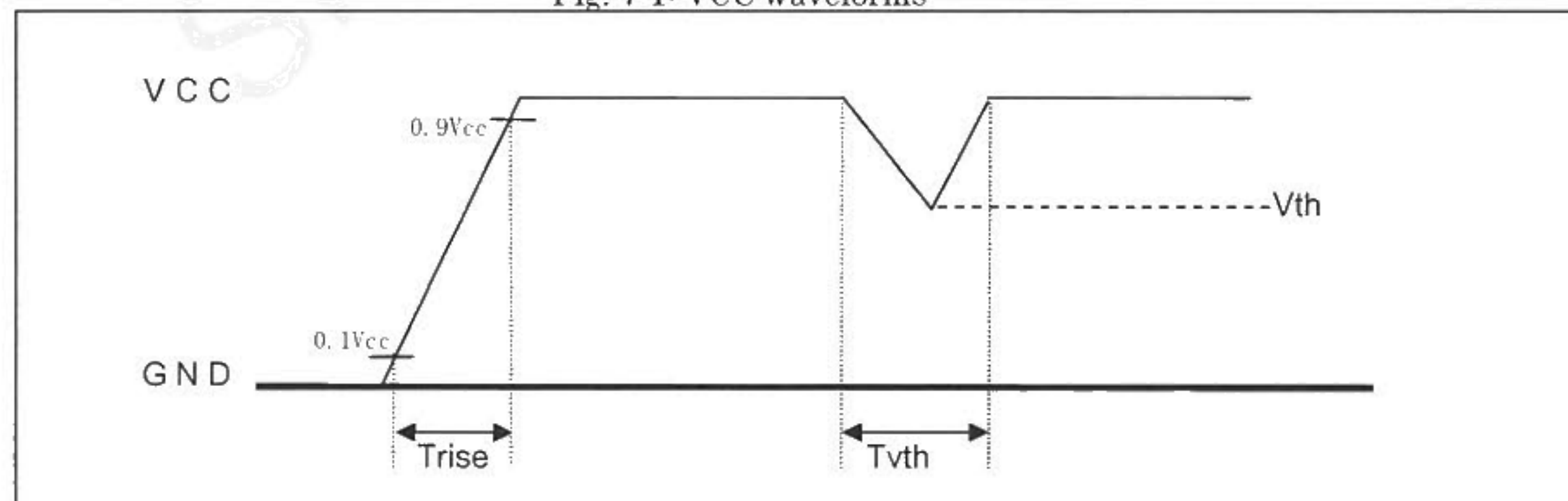
Fig. 7-1: VCC waveforms
