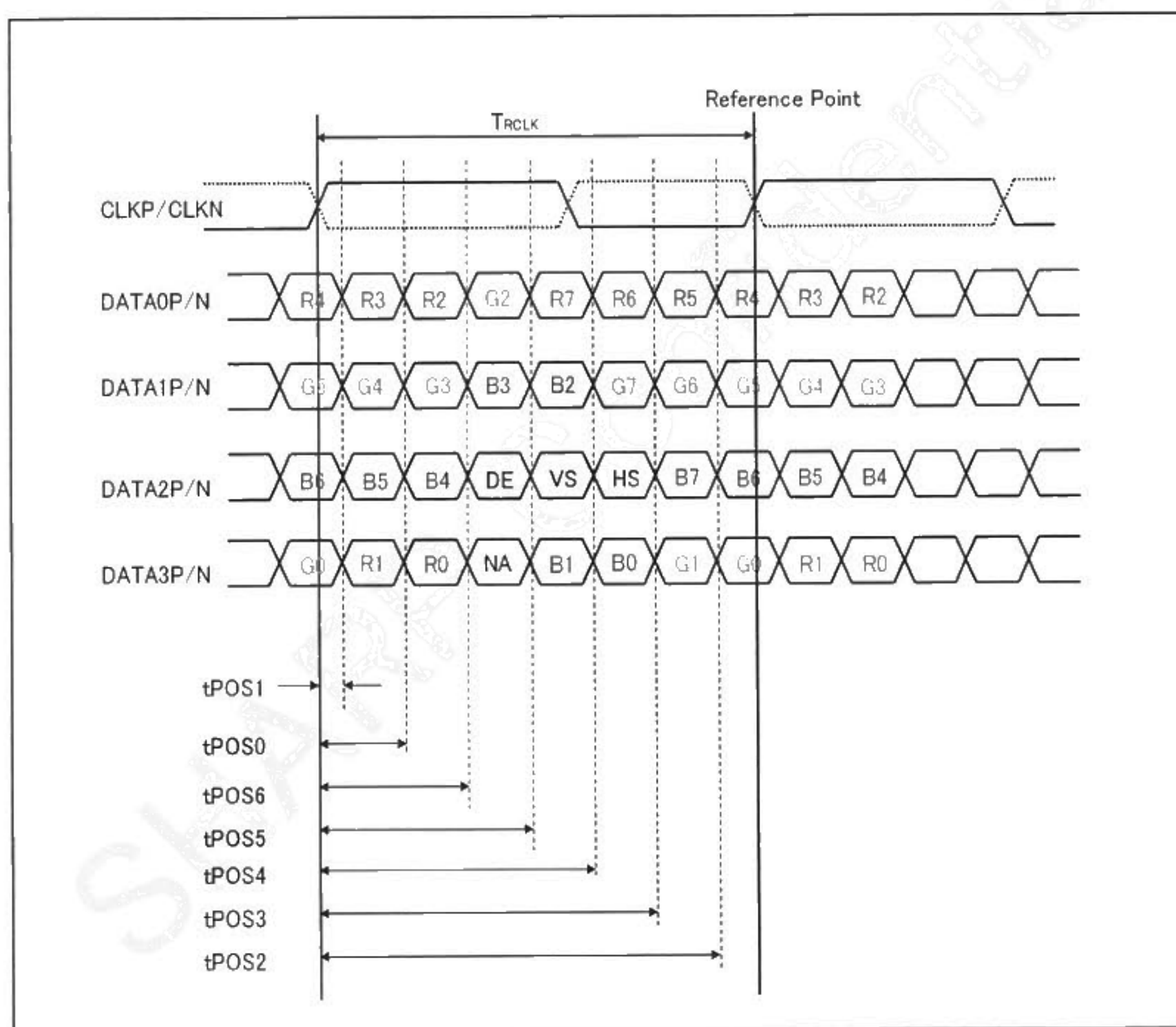
Fig.7-5 Data input signal timing chart
