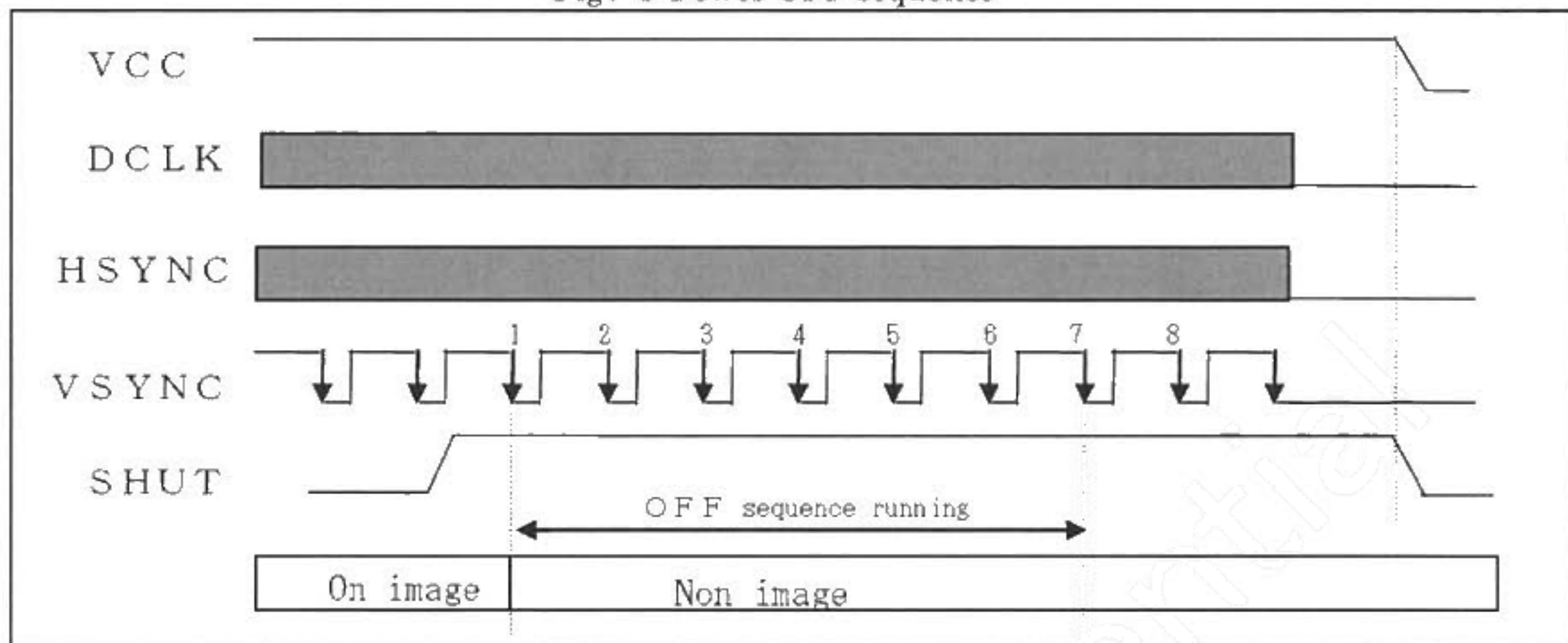
Fig7-4: Power OFF sequence
