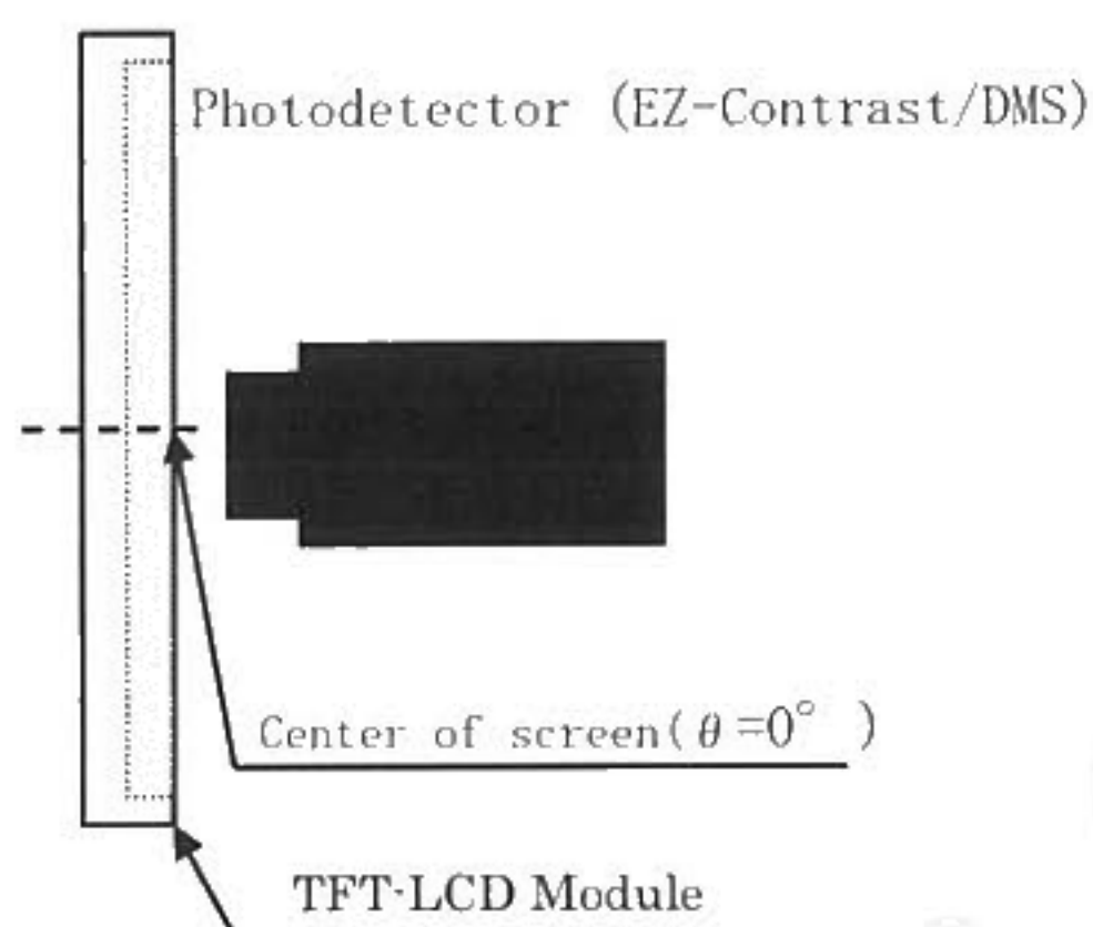
Fig11-1 Viewing angle / Range measurement method
