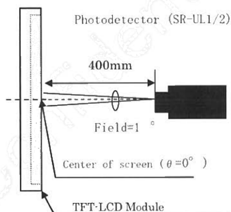
Fig11-2 Luminance / Chromaticity / Contrast measurement method
