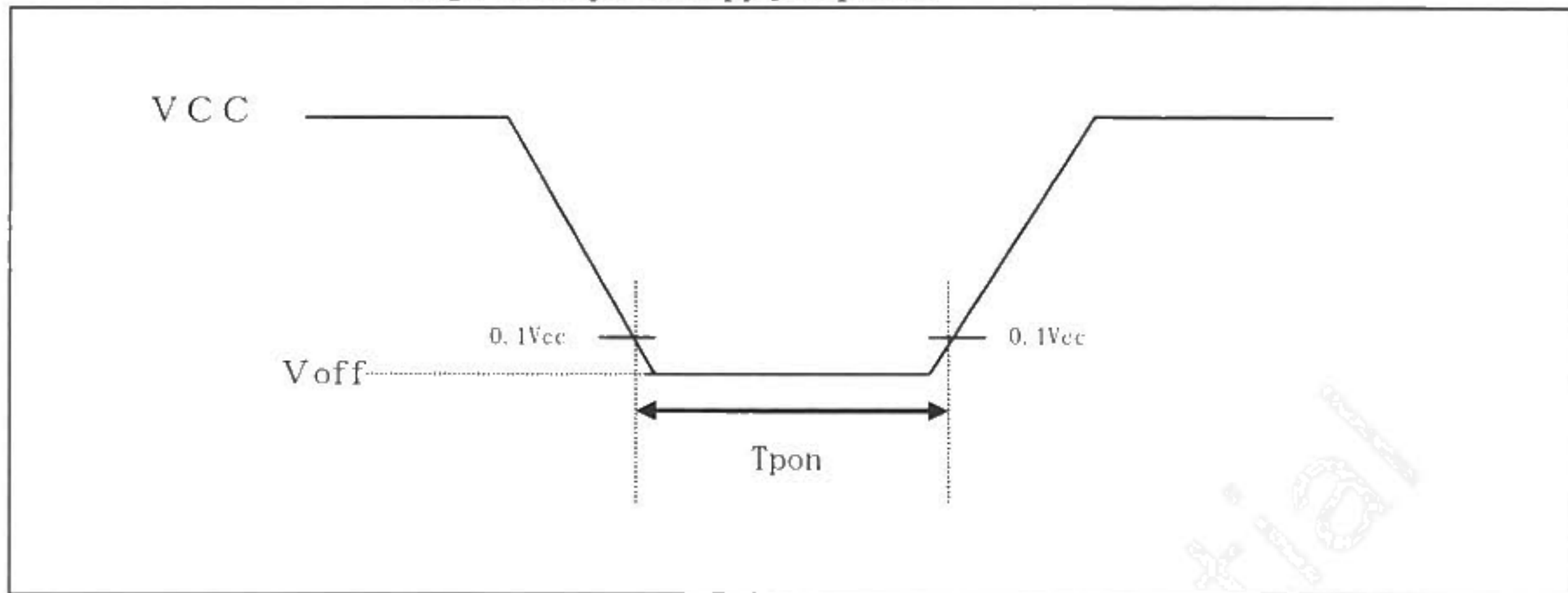
Fig.7-2: Re-power supply sequence
