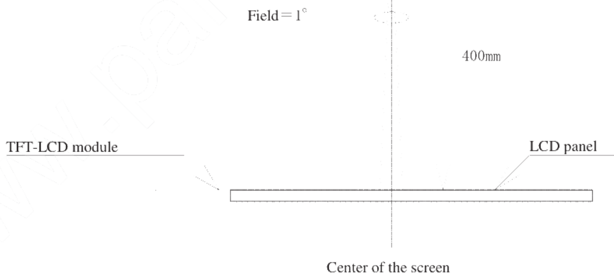
Fig.3 Optical characteristics measurement method
