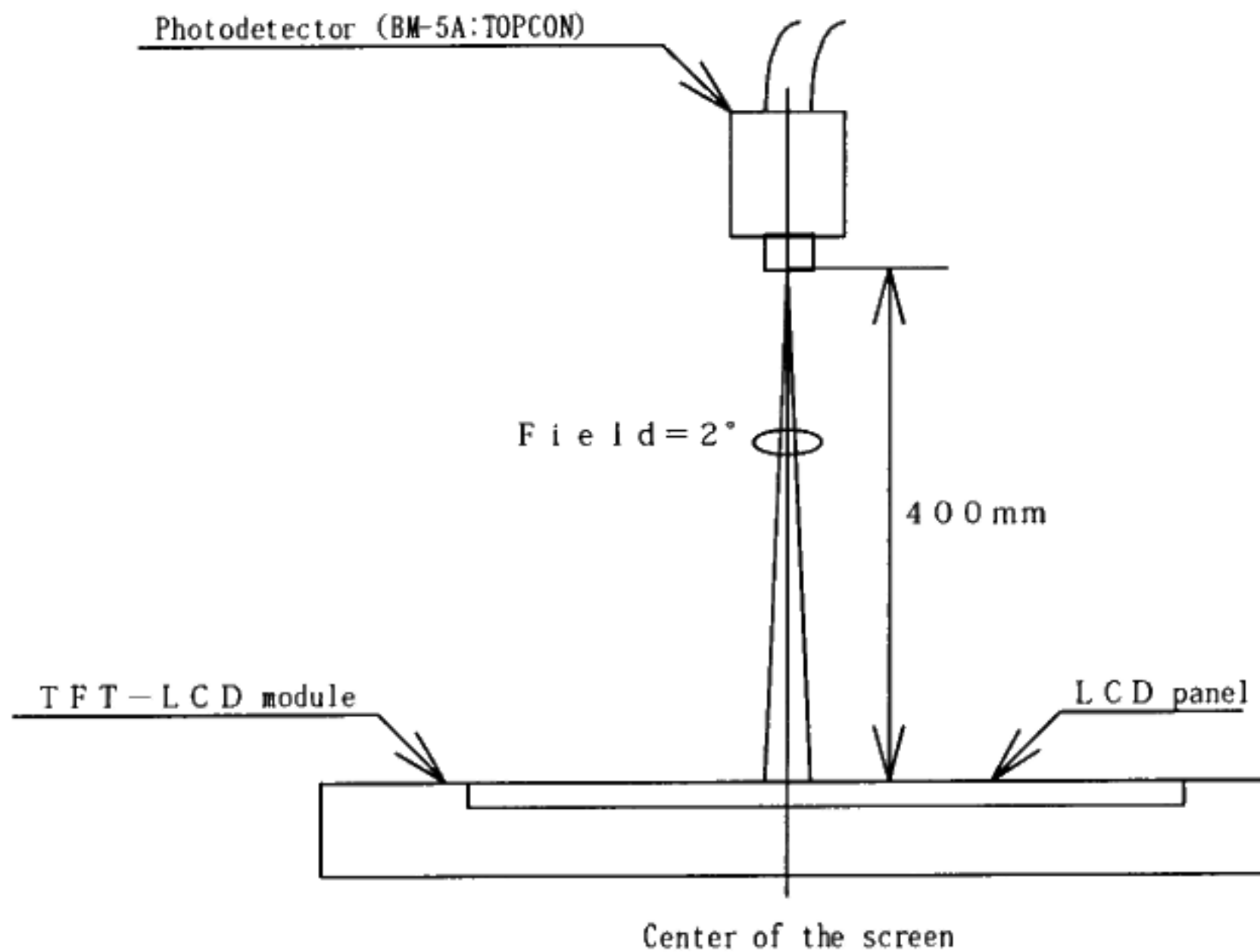
Fig.3 Optical characteristics measurement method
