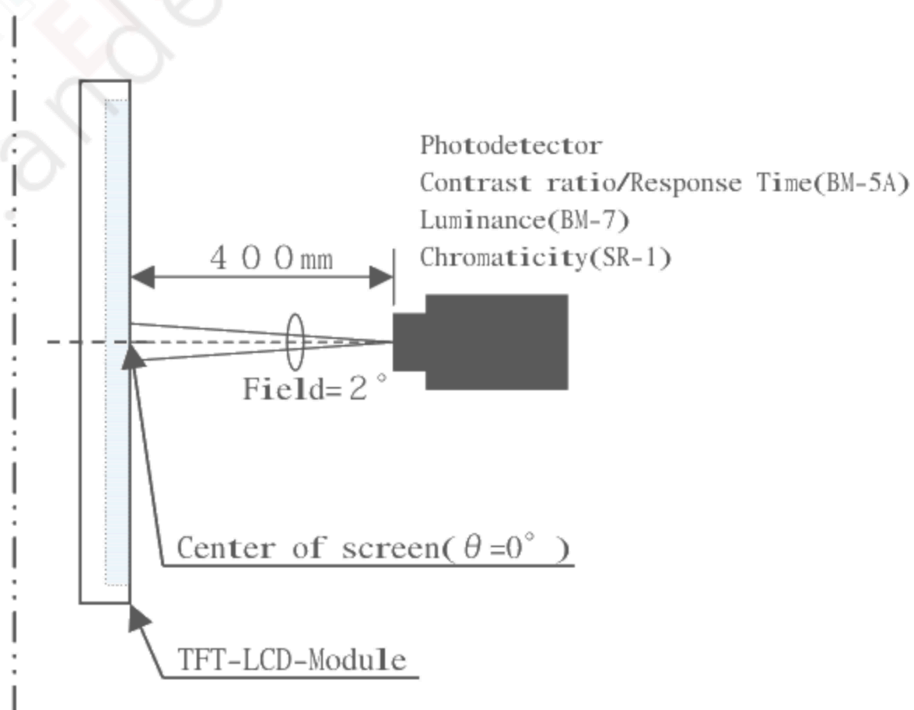
Fig2-2 Luminance/Contrast ratio/Response time/Chromaticity measurement method
