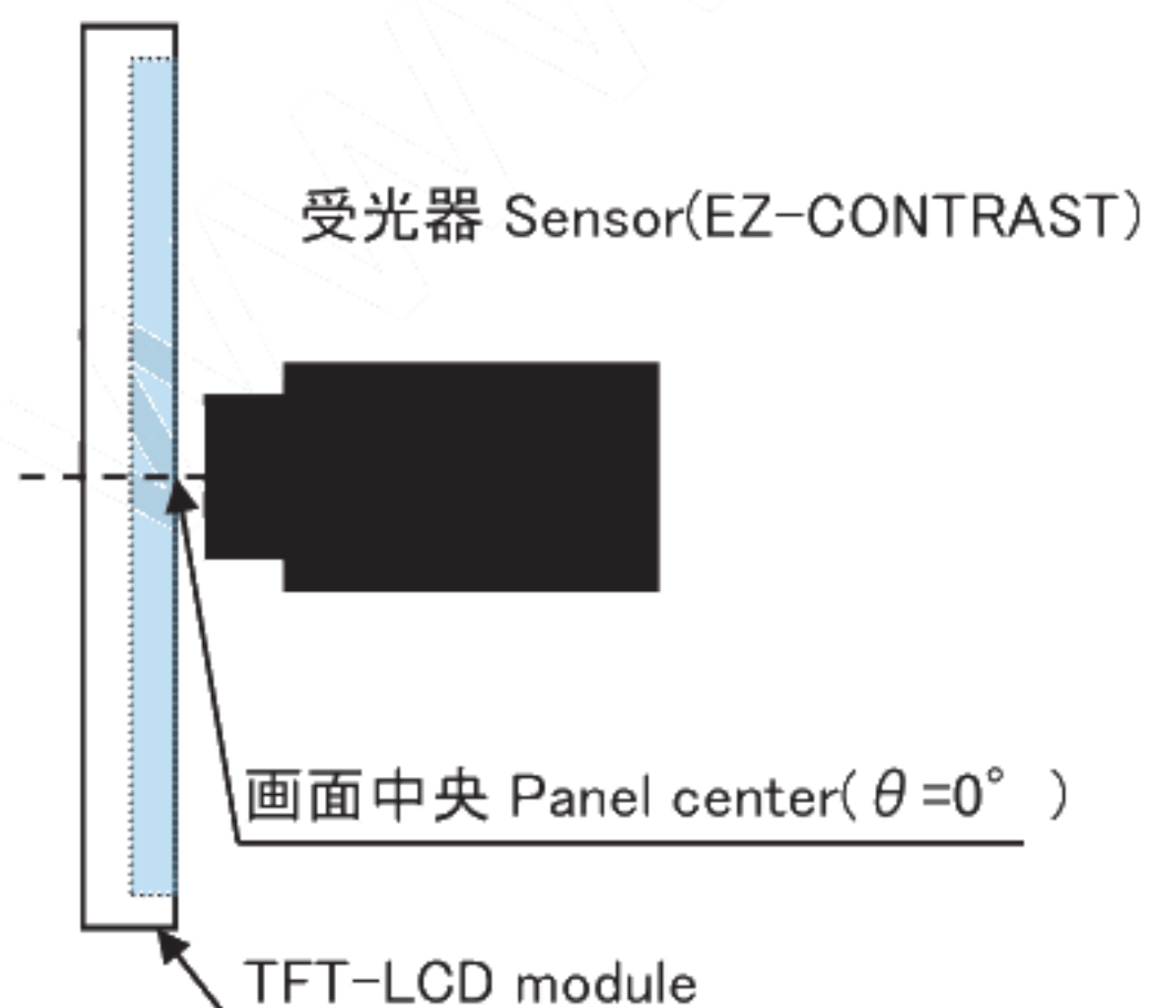
図2-1 視野角特性測定方法 Fig2-1 Measuring setup for Viewing angle
