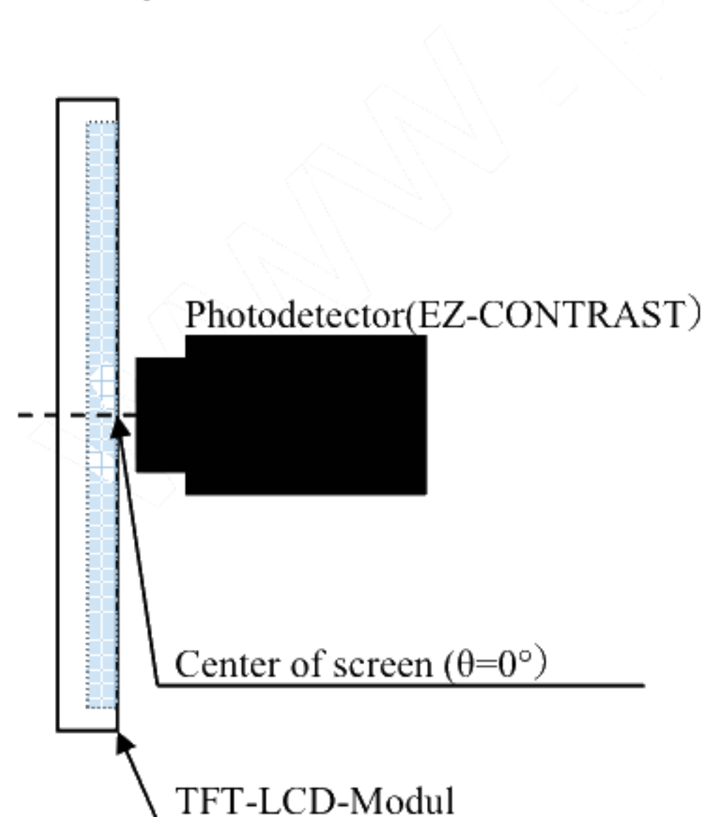
Fig2-1 Viewing angle measurement method
