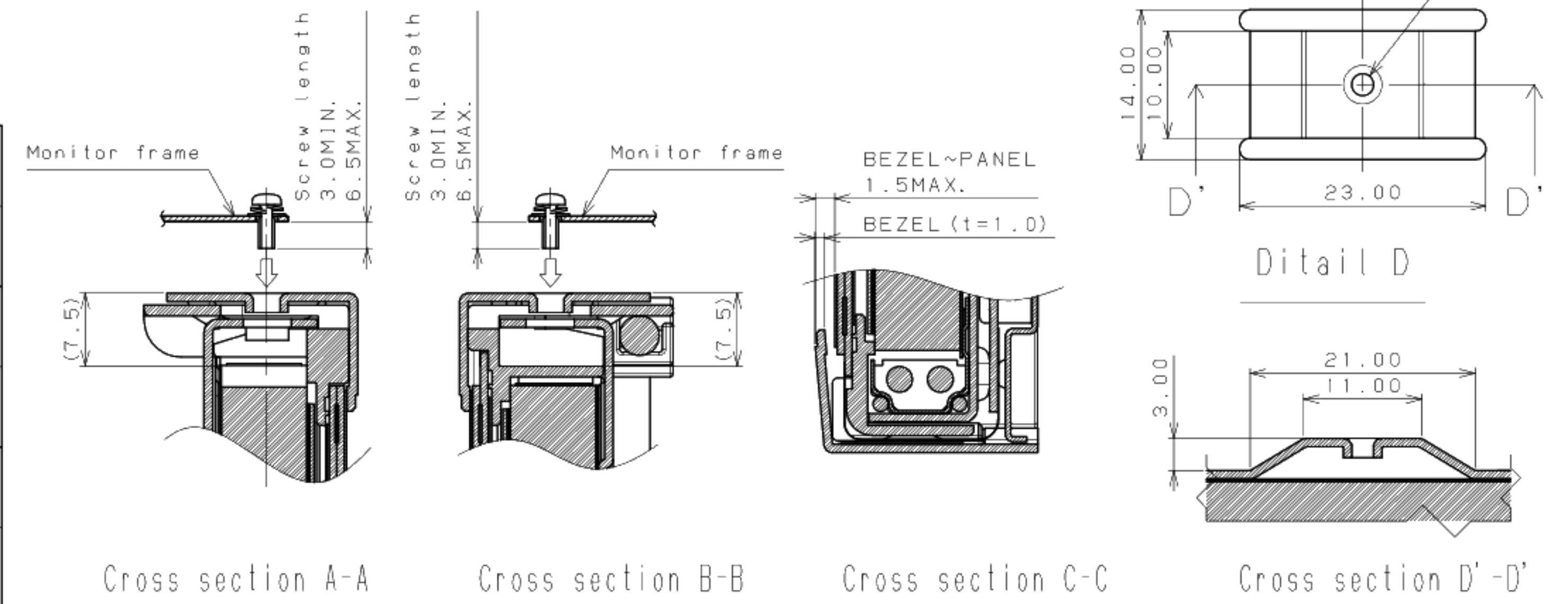
Fig.1:Outline dimensions (LQ190E1LW02)
