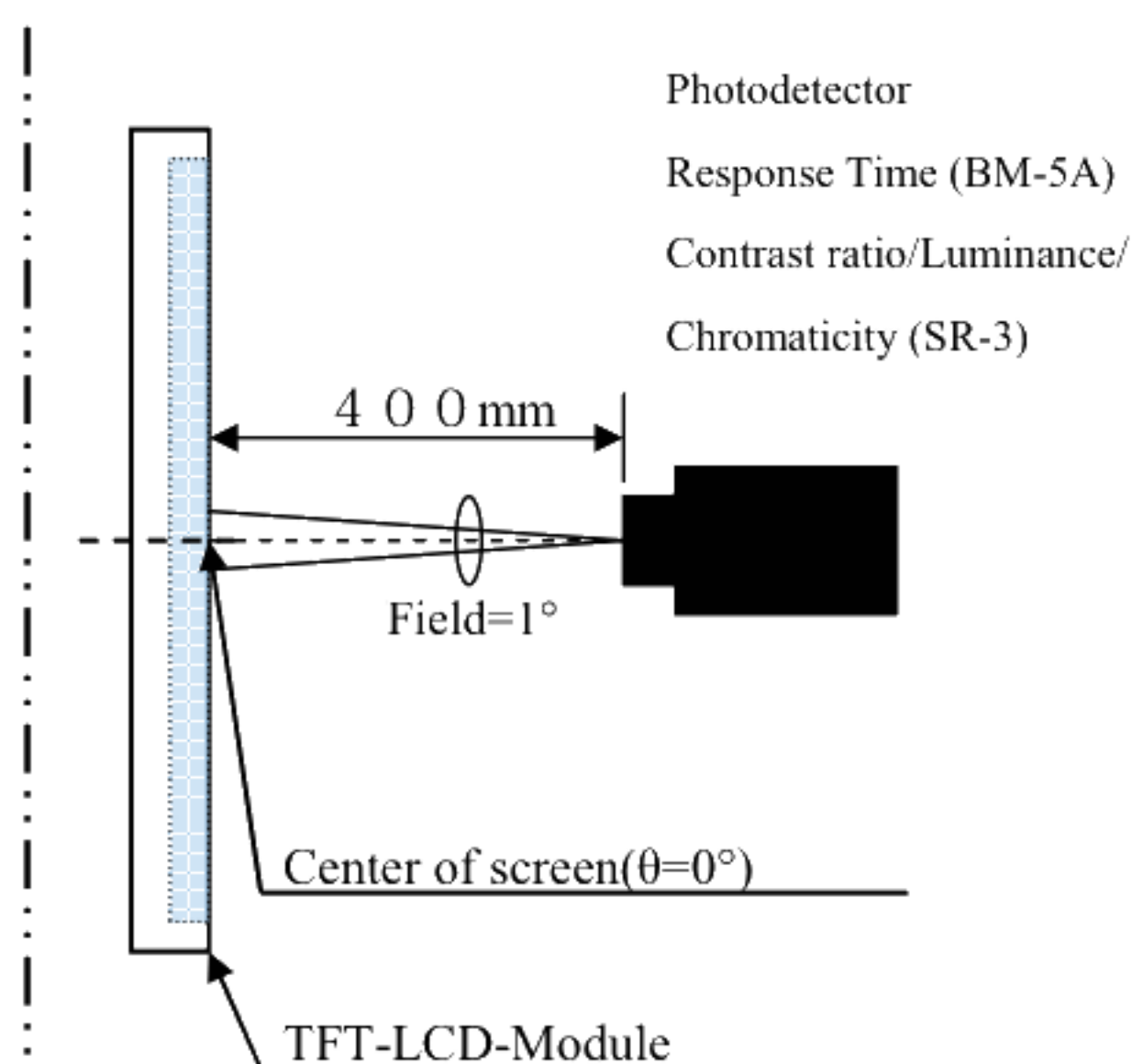
Fig2-2 Luminance/Contrast ratio/Response time/Chromaticity measurement method
