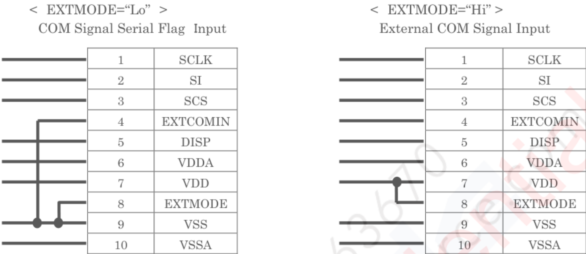
Figure 4-1 Recommended circuit
