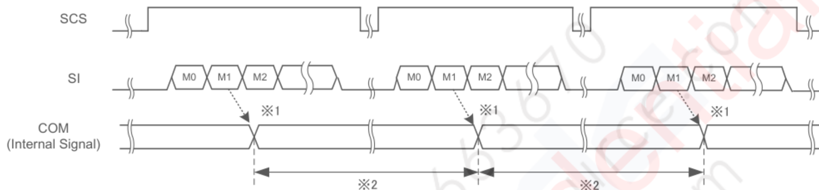
Figure 6-9 COM Inversion (EXTMODE=Lo)
