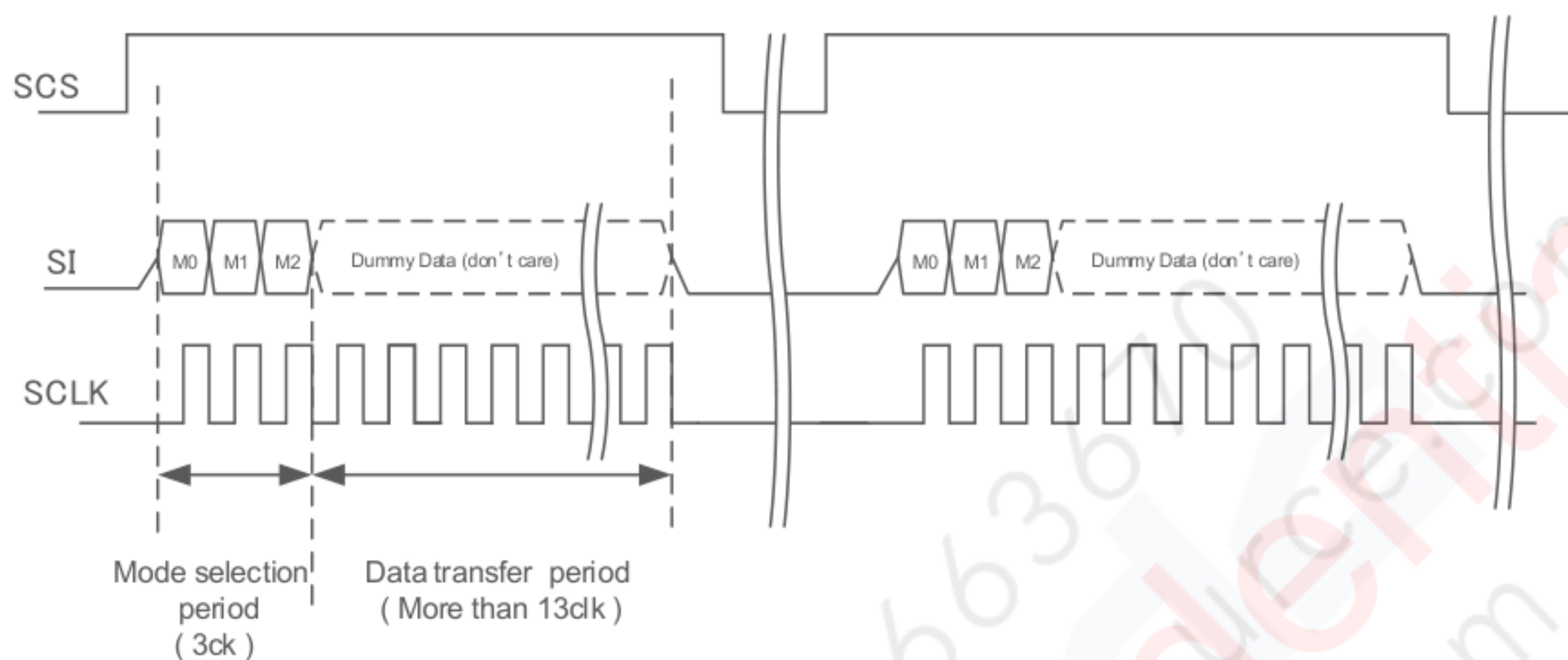
Figure 6-7 HOLD mode
