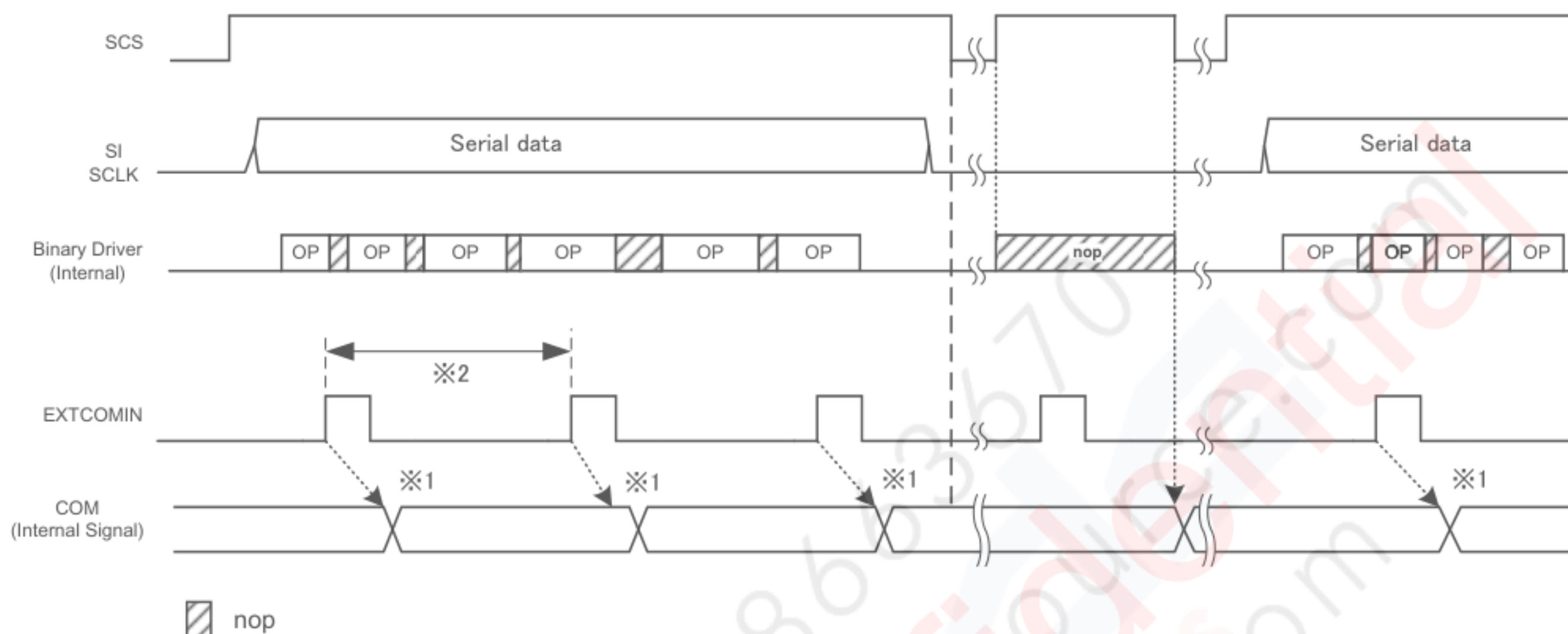
Figure 6-10 COM Inversion (EXTMODE=Hi) 1
