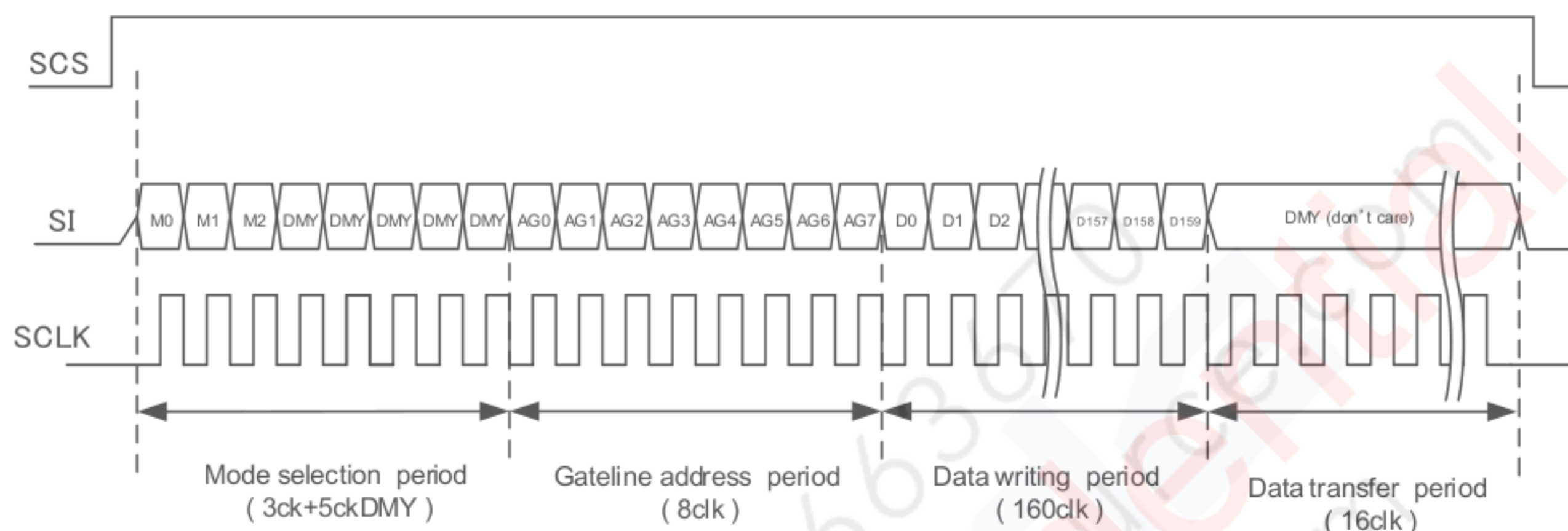
Figure 6-5 Data update mode by 1line
