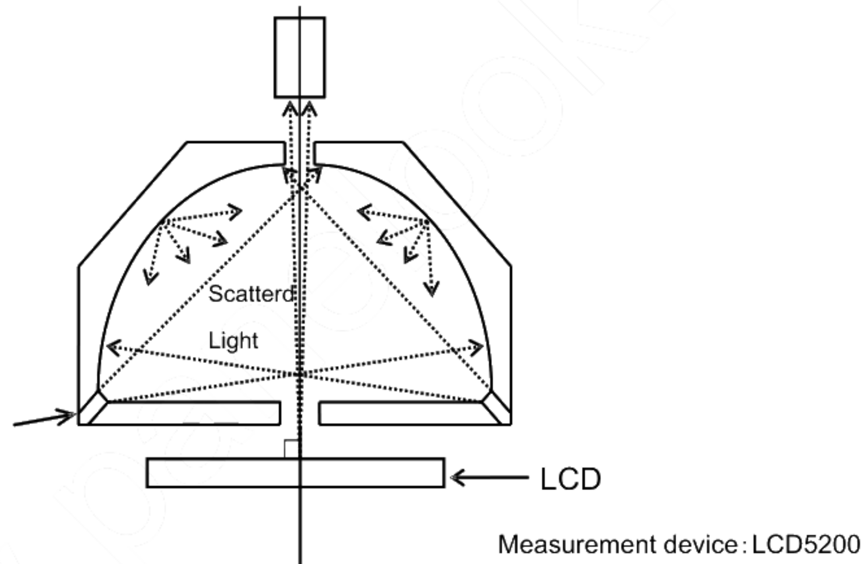
Figure 11-2 Reflection mode viewing angle measurement method
